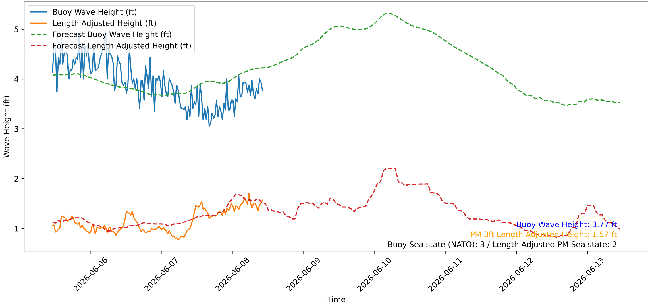
Wave Heights over Time for Red Beach at 2026-06-08 10:40:46
