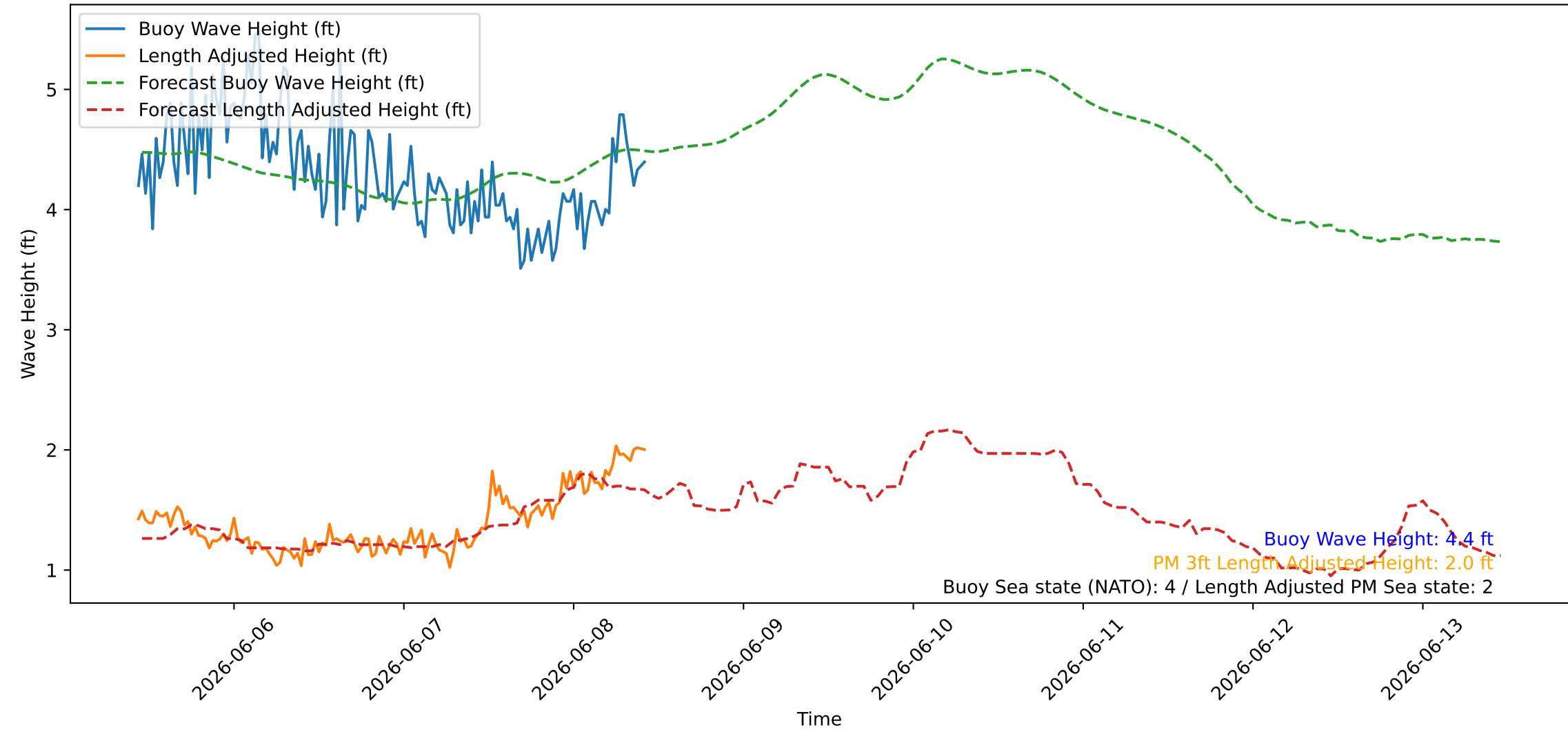
Wave Heights over Time for Oceanside Harbor at 2026-06-08 10:40:26
