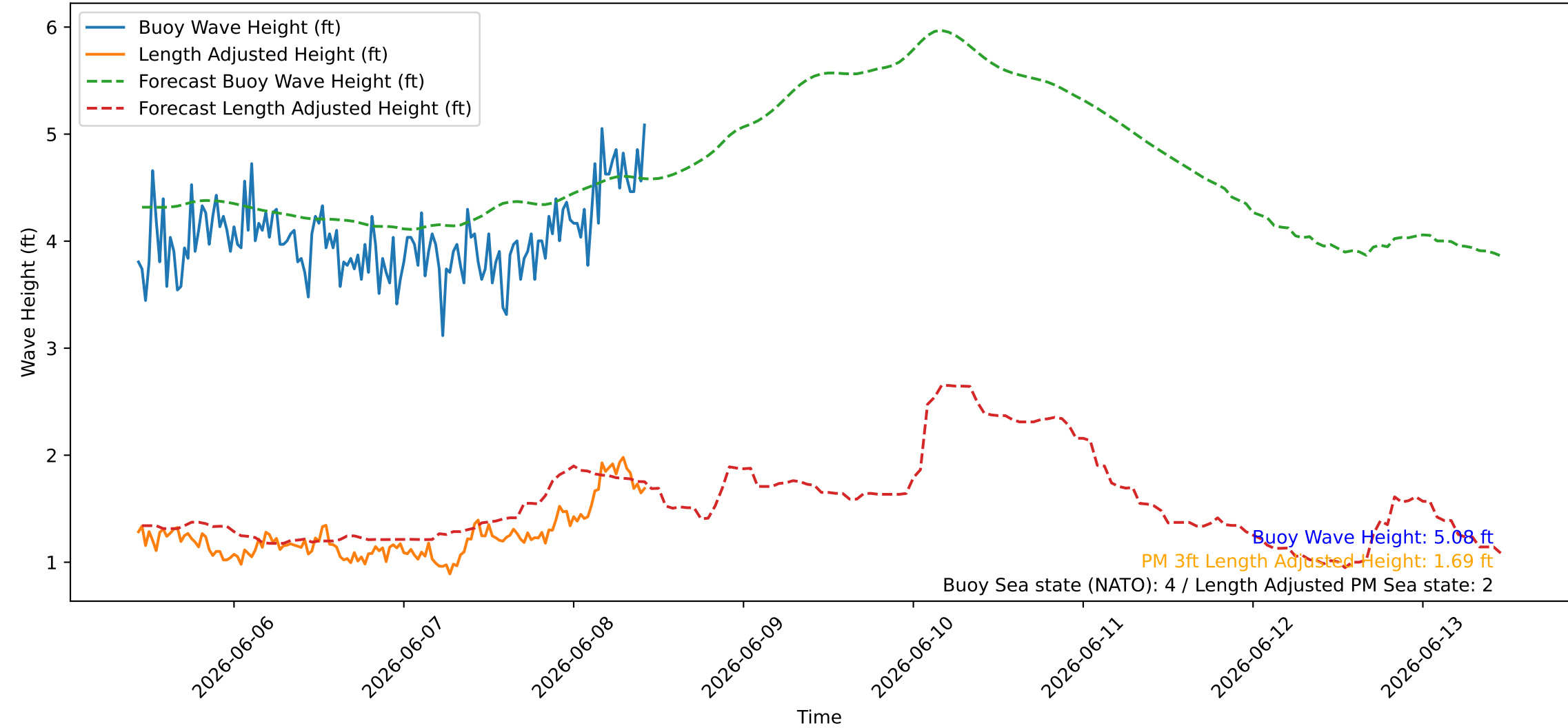
Wave Heights over Time for Green Beach at 2026-06-08 10:41:14
