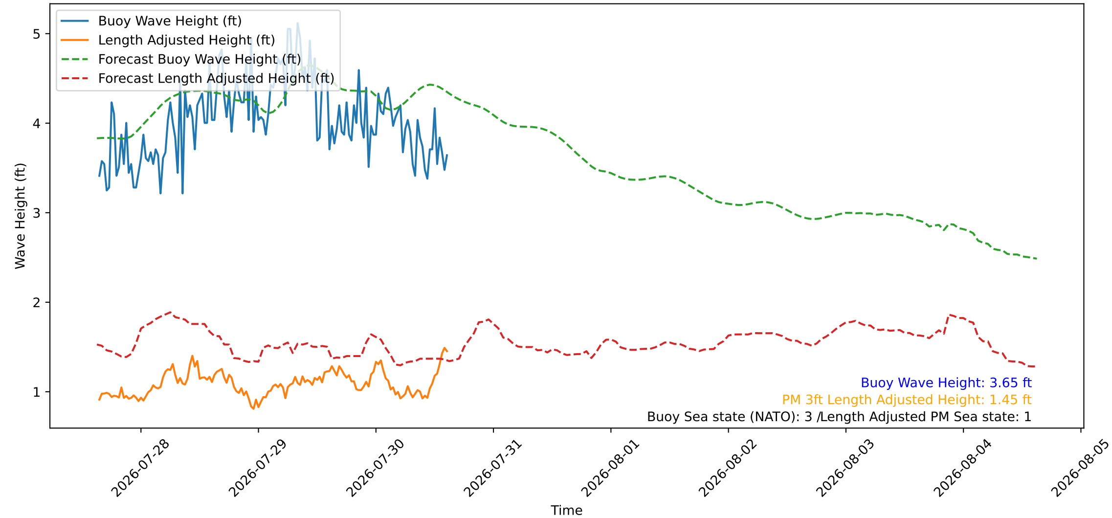
Wave Heights over Time for Red Beach at 2026-07-30 15:20:48
