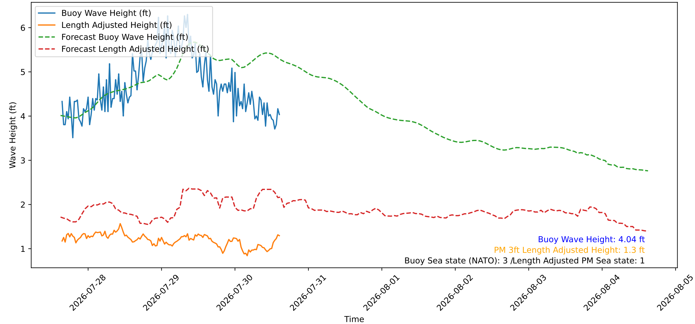
Wave Heights over Time for Green Beach at 2026-07-30 15:21:11
