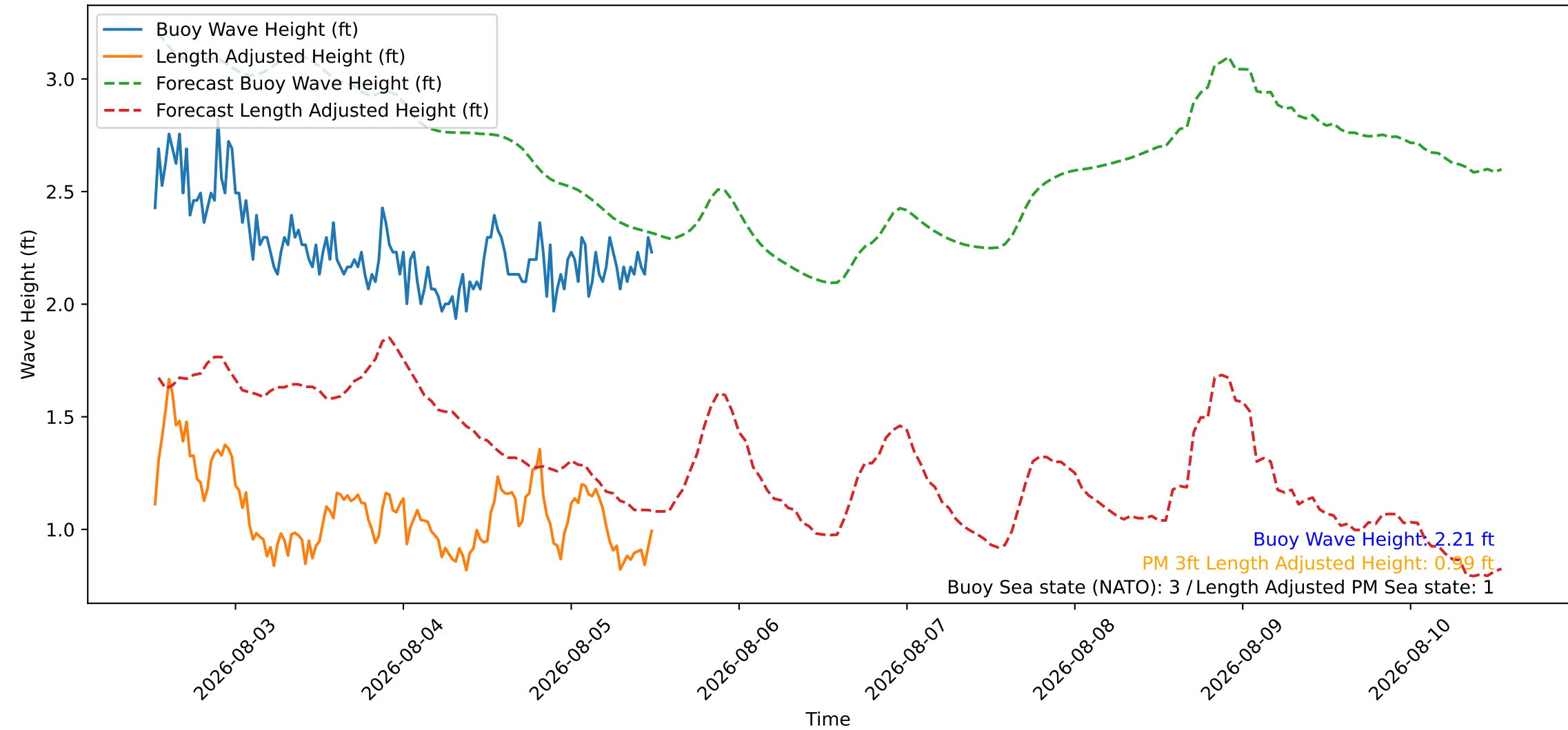
Wave Heights over Time for Green Beach at 2026-08-05 12:31:09
