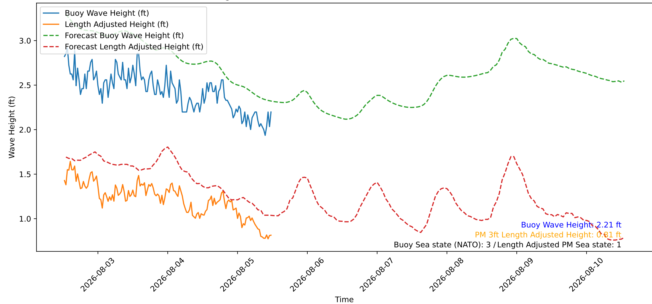
Wave Heights over Time for Oceanside Harbor at 2026-08-05 12:30:27
