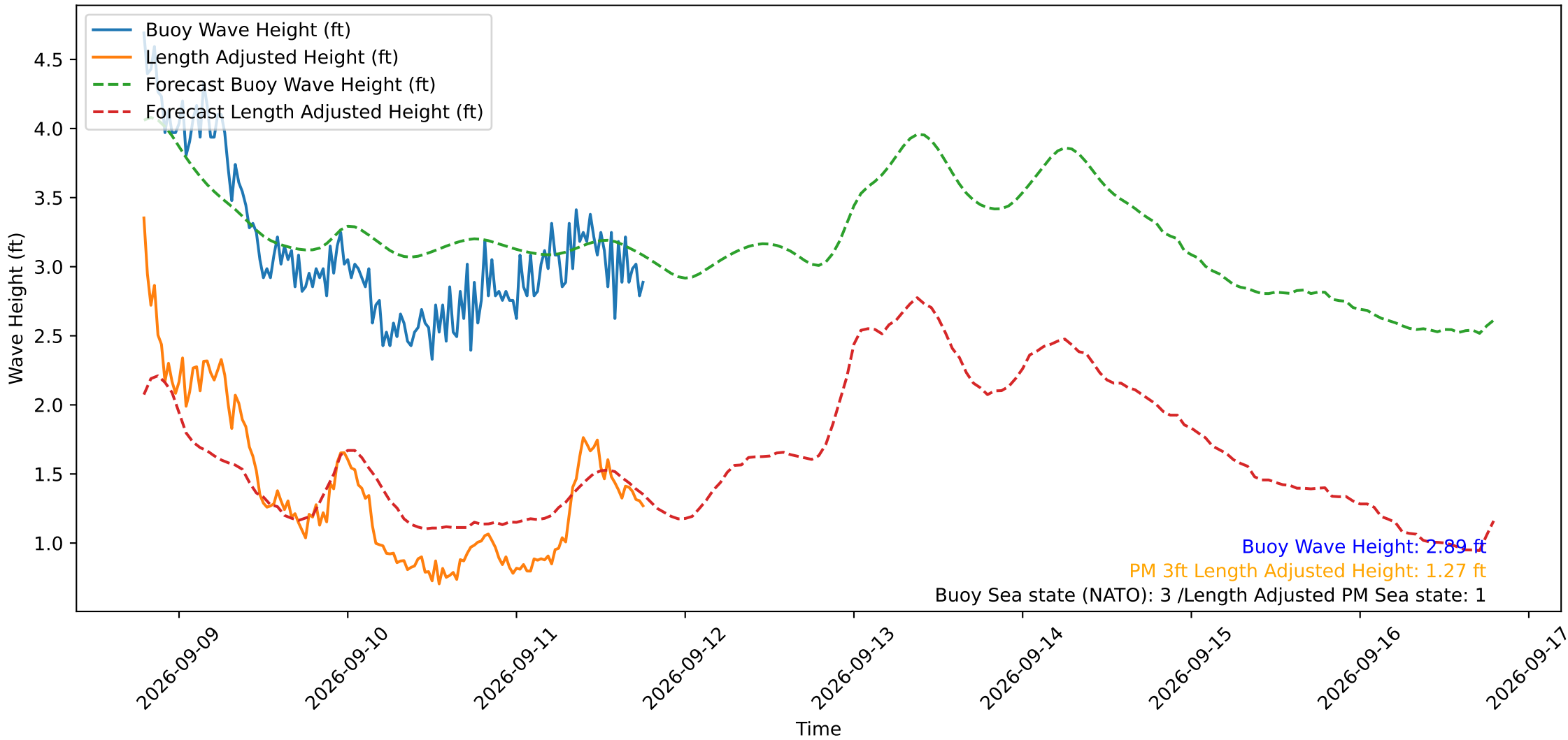
Wave Heights over Time for Red Beach at 2026-09-11 18:50:50
