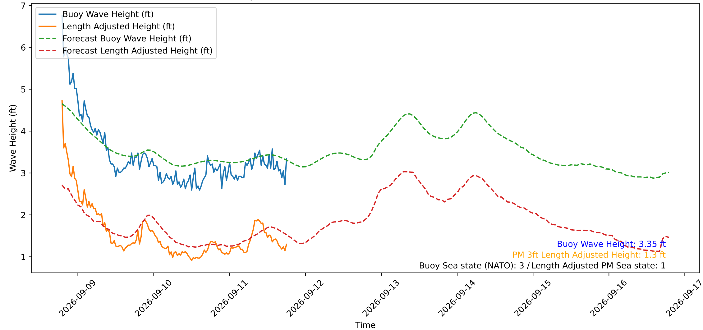
Wave Heights over Time for Green Beach at 2026-09-11 18:51:14
