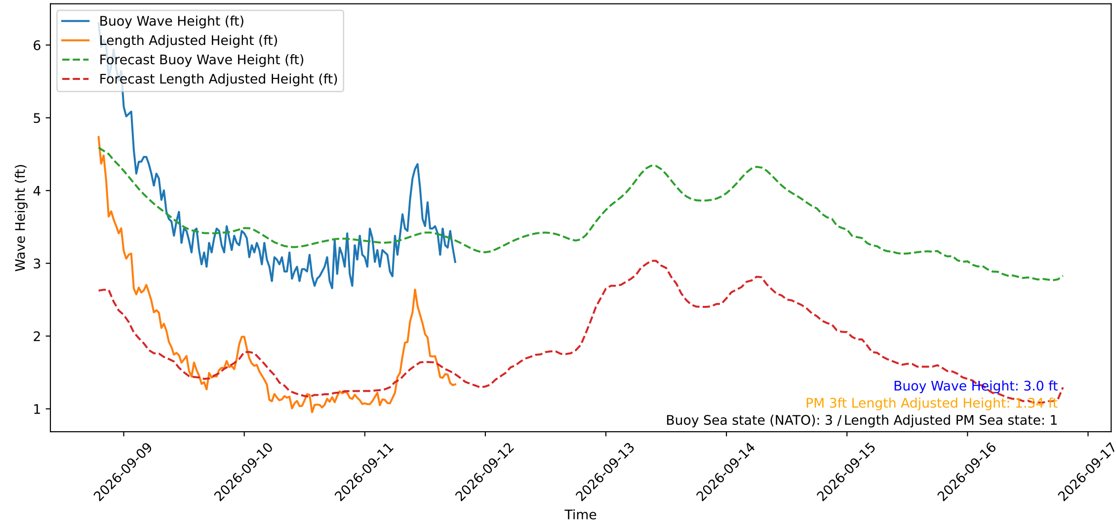
Wave Heights over Time for Oceanside Harbor at 2026-09-11 18:50:29
