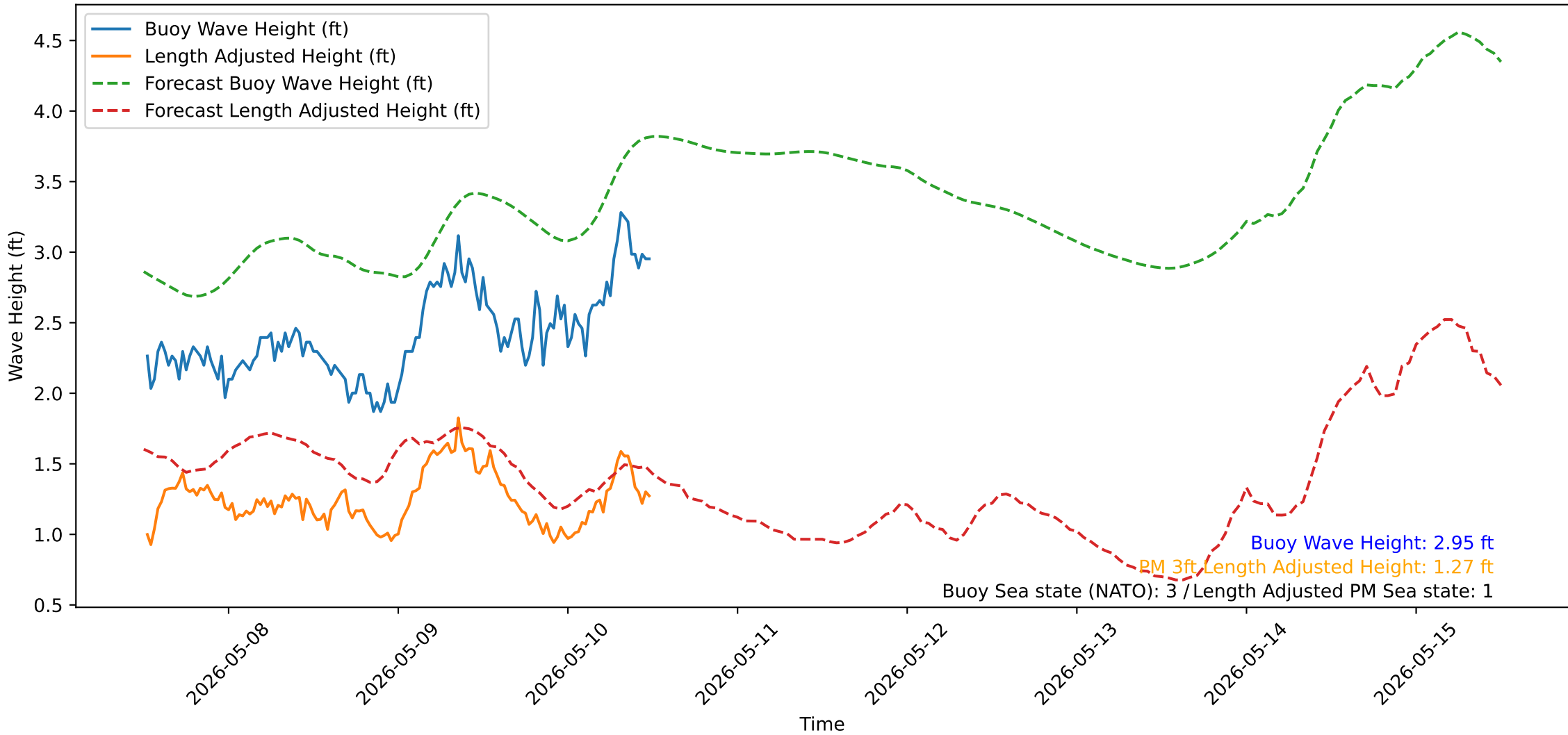
Wave Heights over Time for Oceanside Harbor at 2026-05-10 12:20:33
