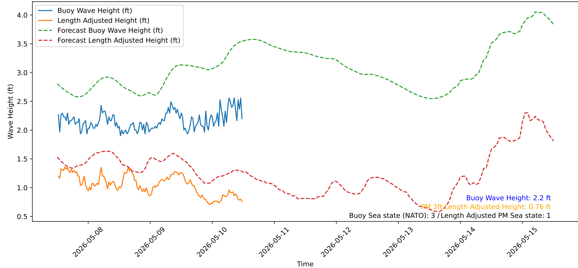
Wave Heights over Time for Red Beach at 2026-05-10 12:20:56
