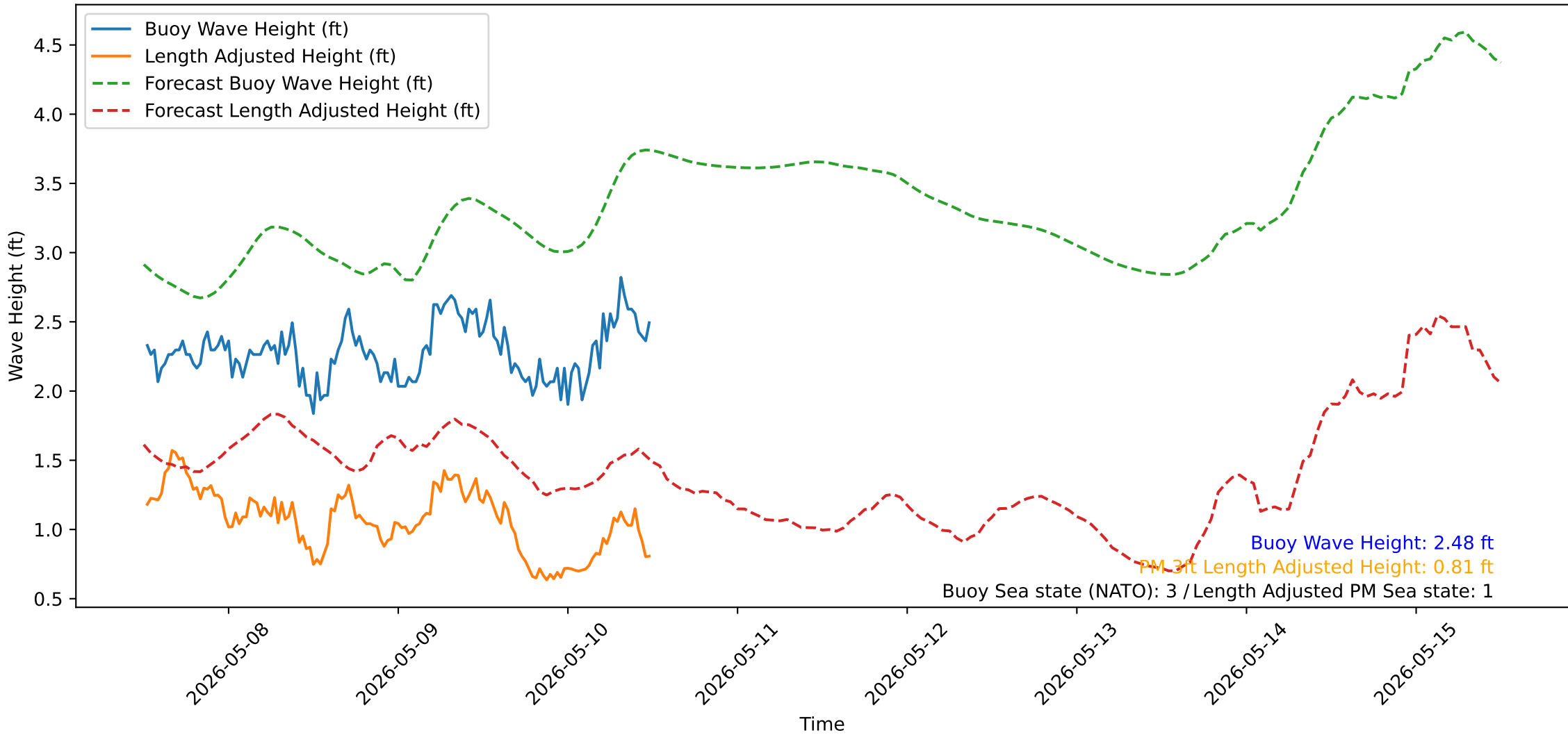
Wave Heights over Time for Green Beach at 2026-05-10 12:21:21
