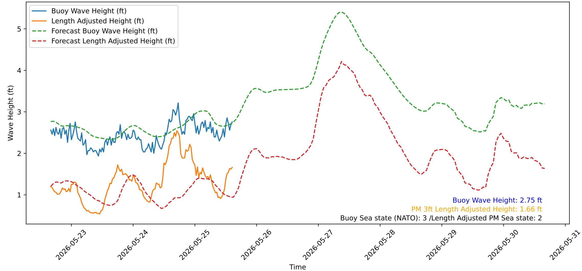
Wave Heights over Time for Red Beach at 2026-05-25 15:30:49
