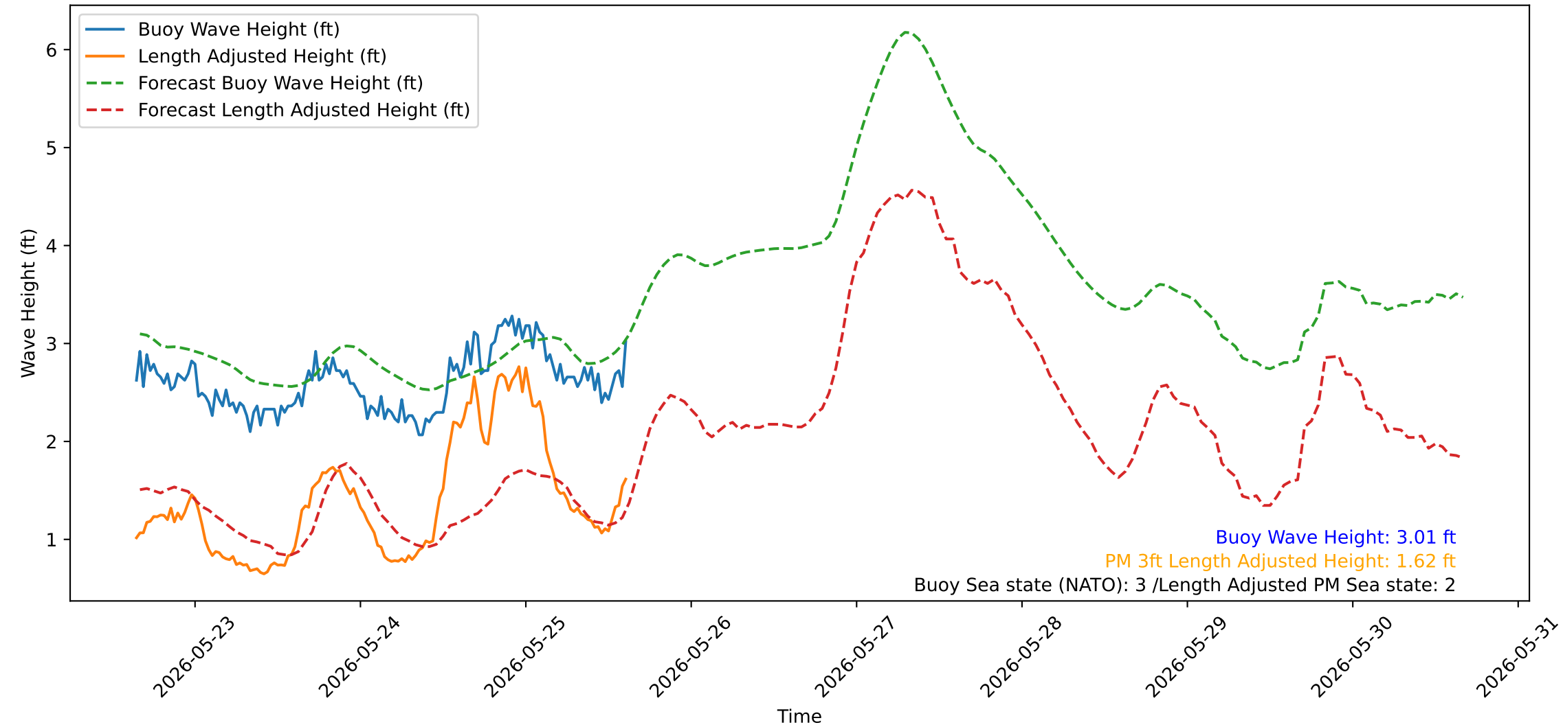
Wave Heights over Time for Green Beach at 2026-05-25 15:31:11
