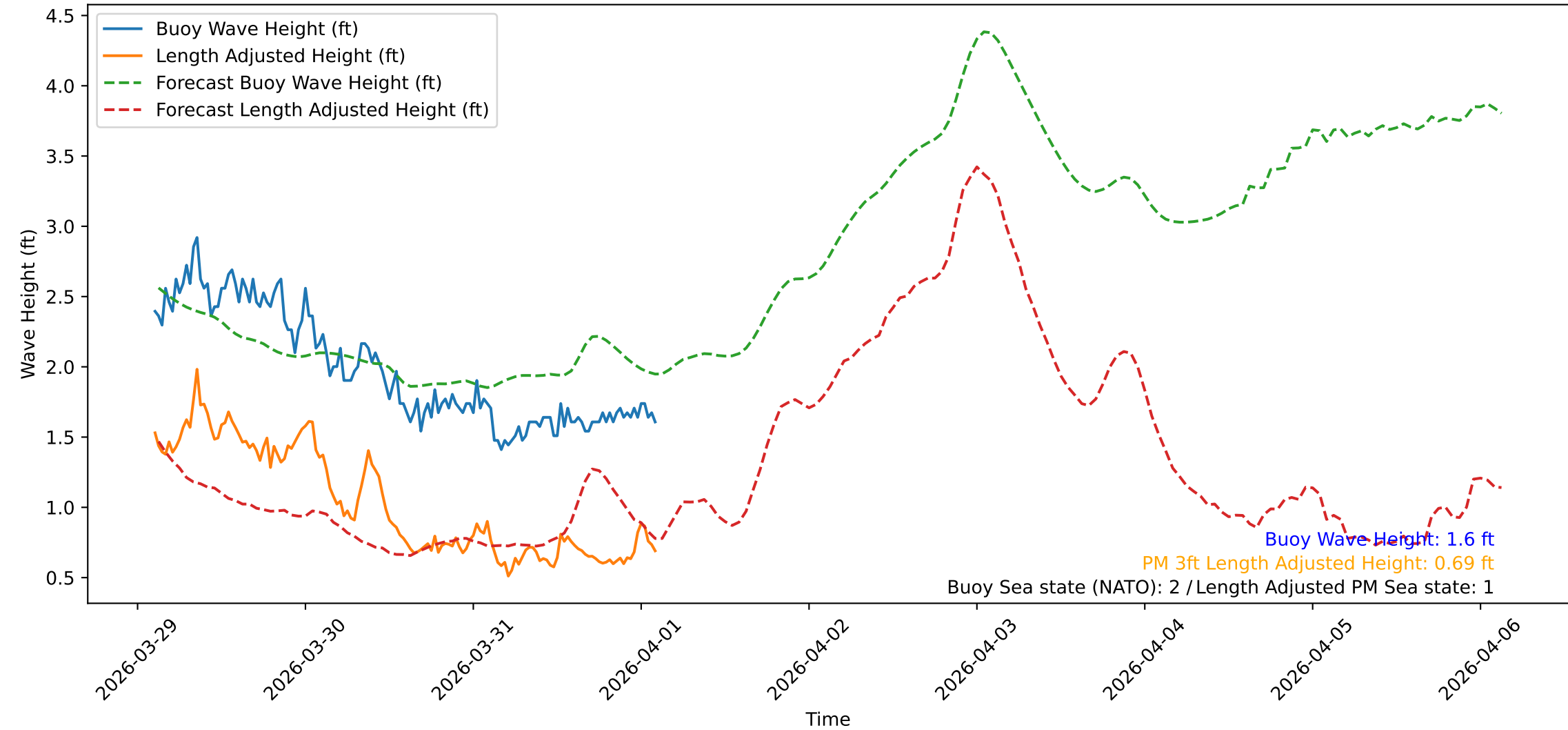
Wave Heights over Time for Green Beach at 2026-04-01 02:41:09
