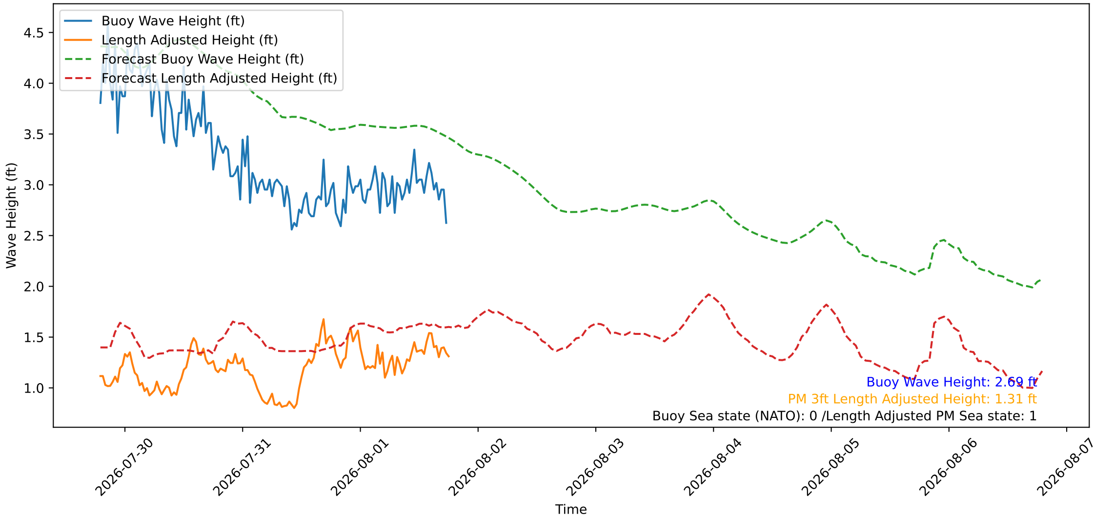
Wave Heights over Time for Red Beach at 2026-08-01 18:40:46
