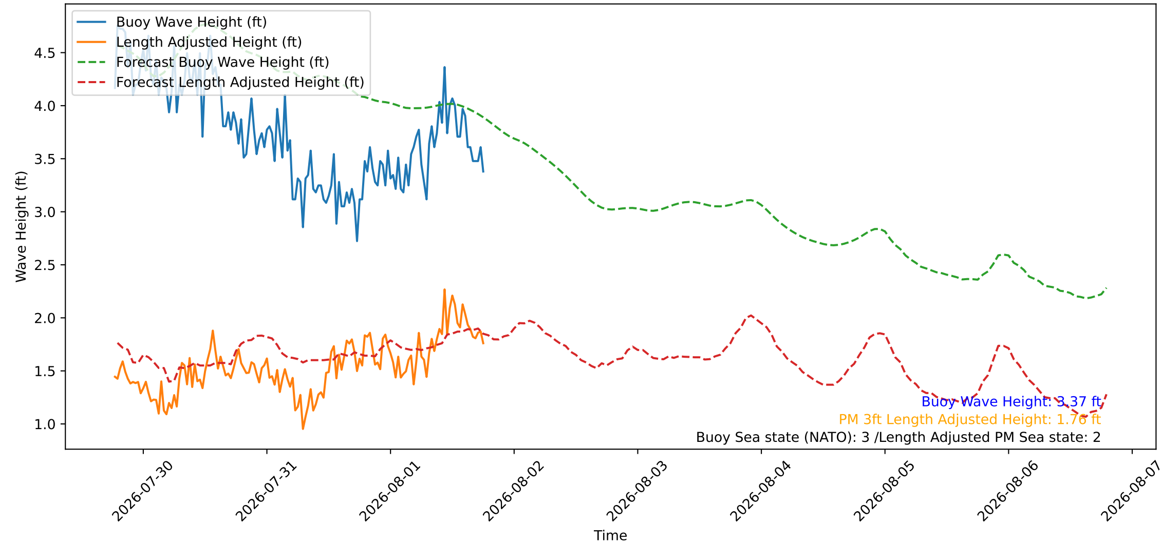
Wave Heights over Time for Oceanside Harbor at 2026-08-01 18:40:26
