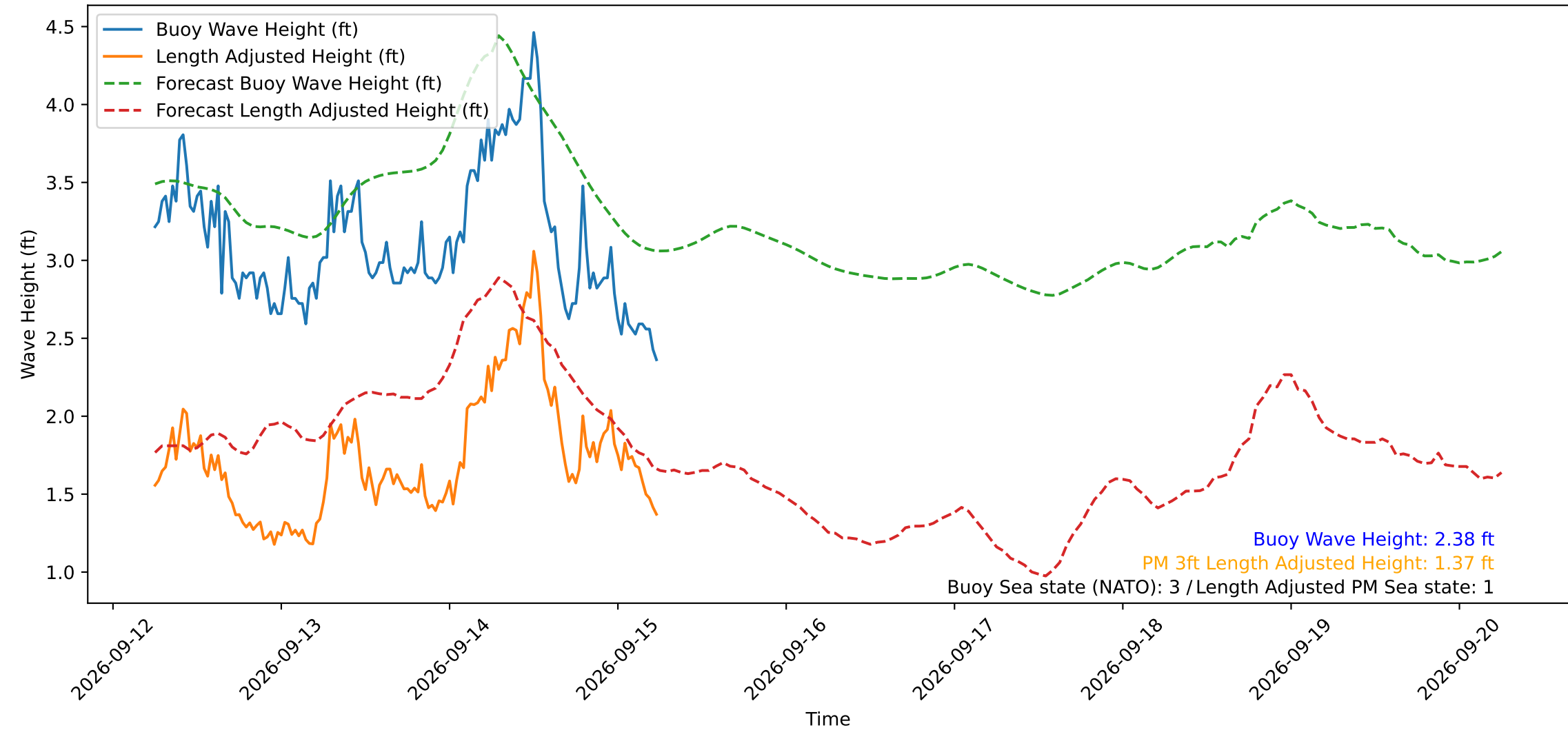
Wave Heights over Time for Oceanside Harbor at 2026-09-15 06:10:30
