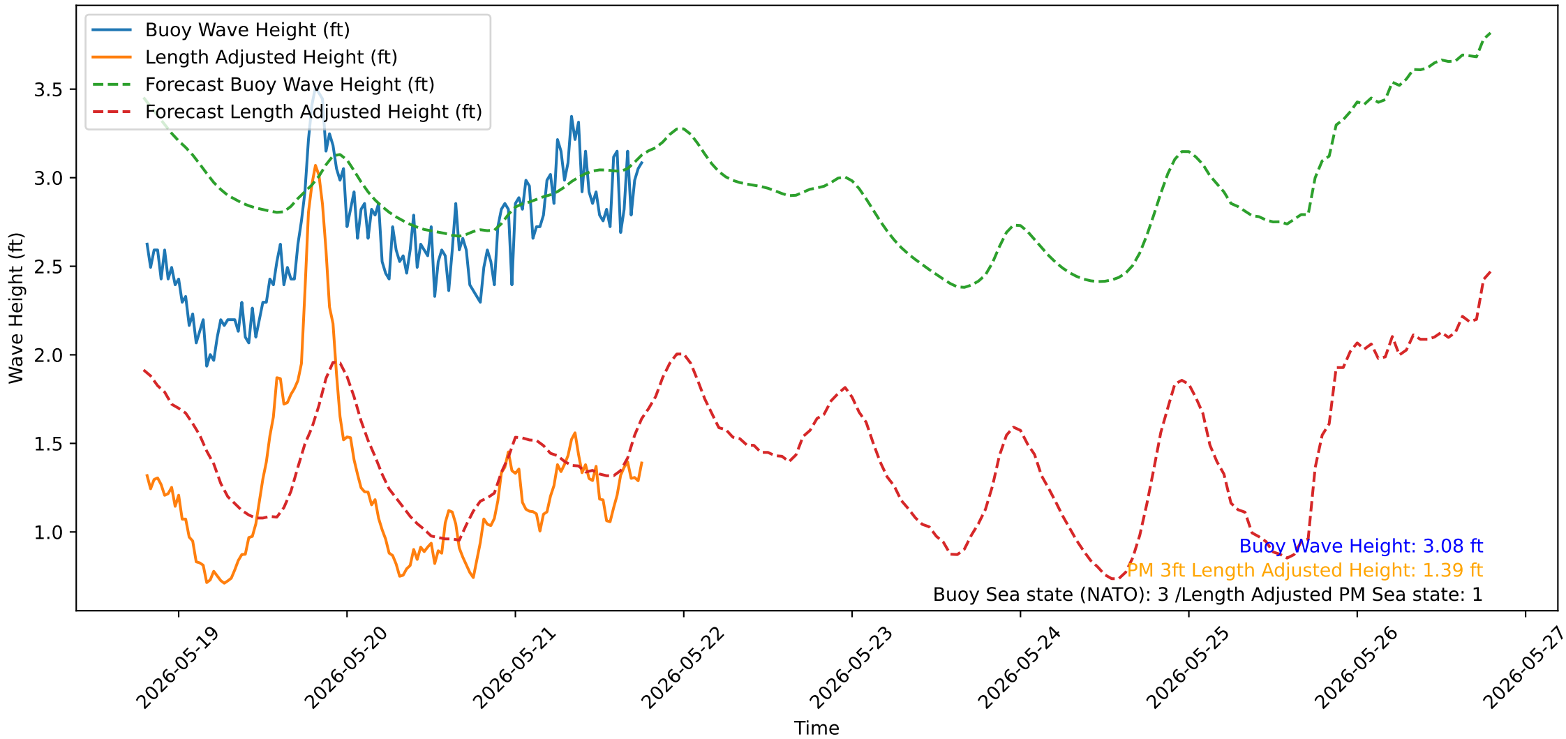
Wave Heights over Time for Red Beach at 2026-05-21 19:00:51
