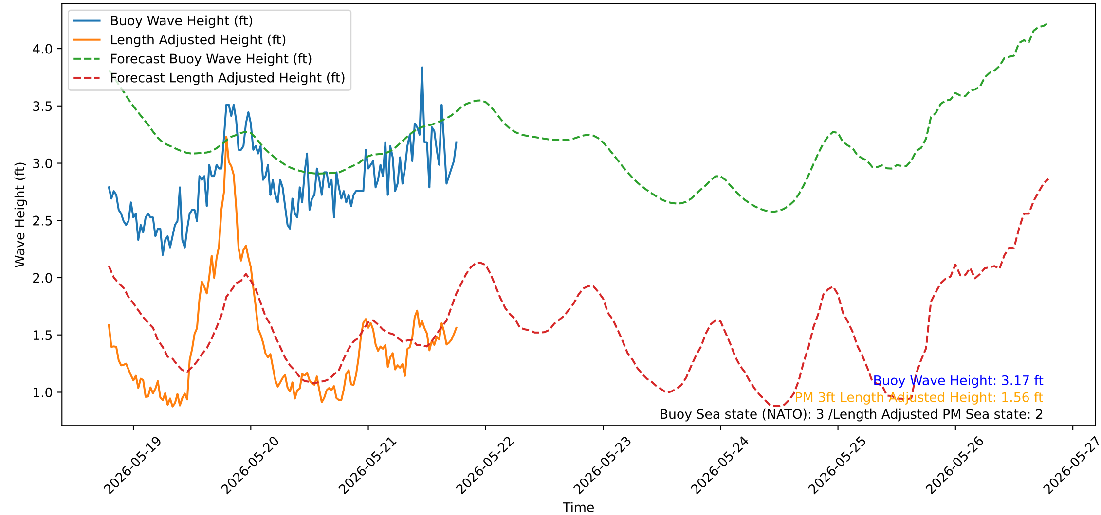
Wave Heights over Time for Oceanside Harbor at 2026-05-21 19:00:31
