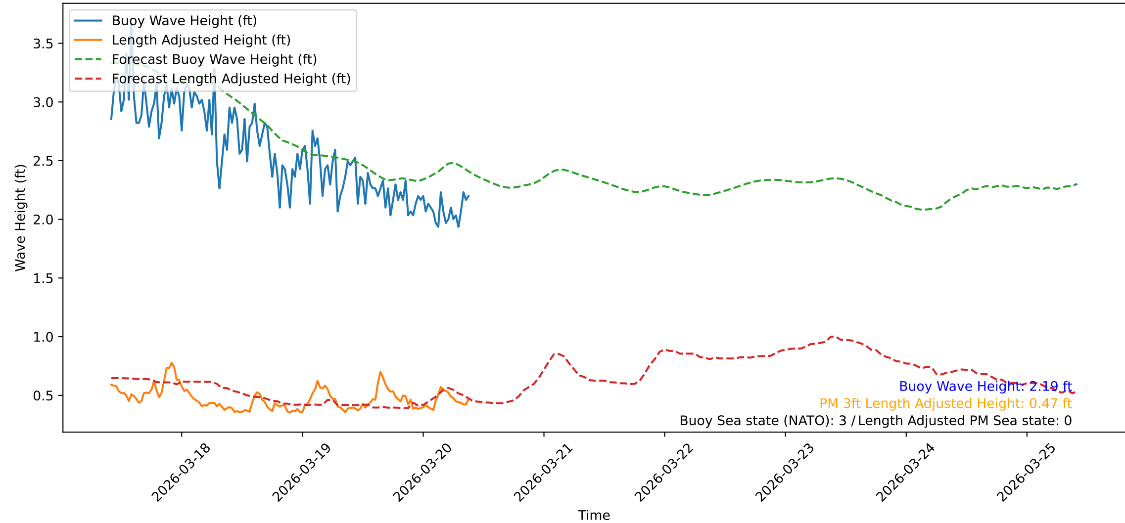
Wave Heights over Time for Red Beach at 2026-03-20 09:40:47
