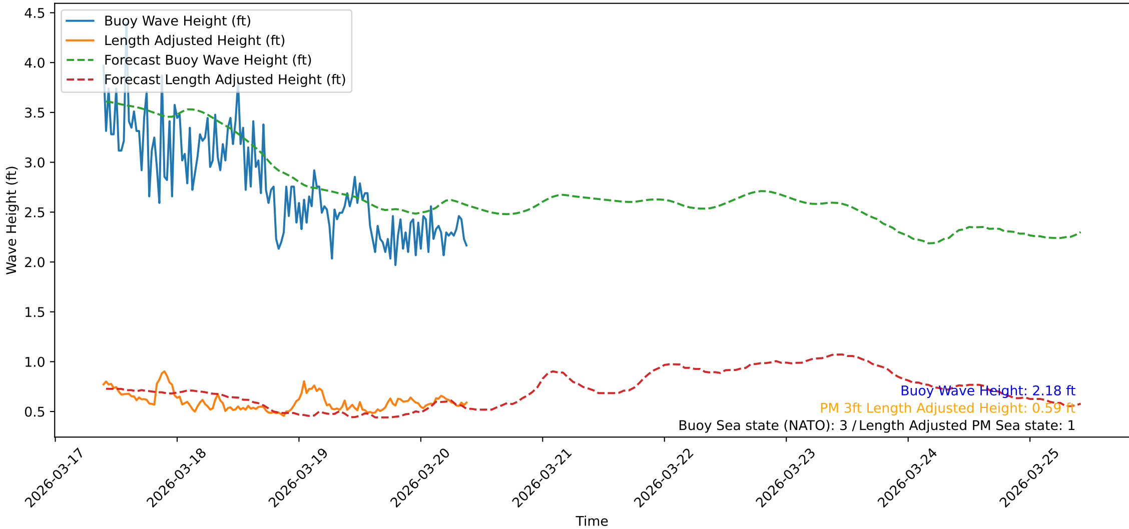
Wave Heights over Time for Oceanside Harbor at 2026-03-20 09:40:31
