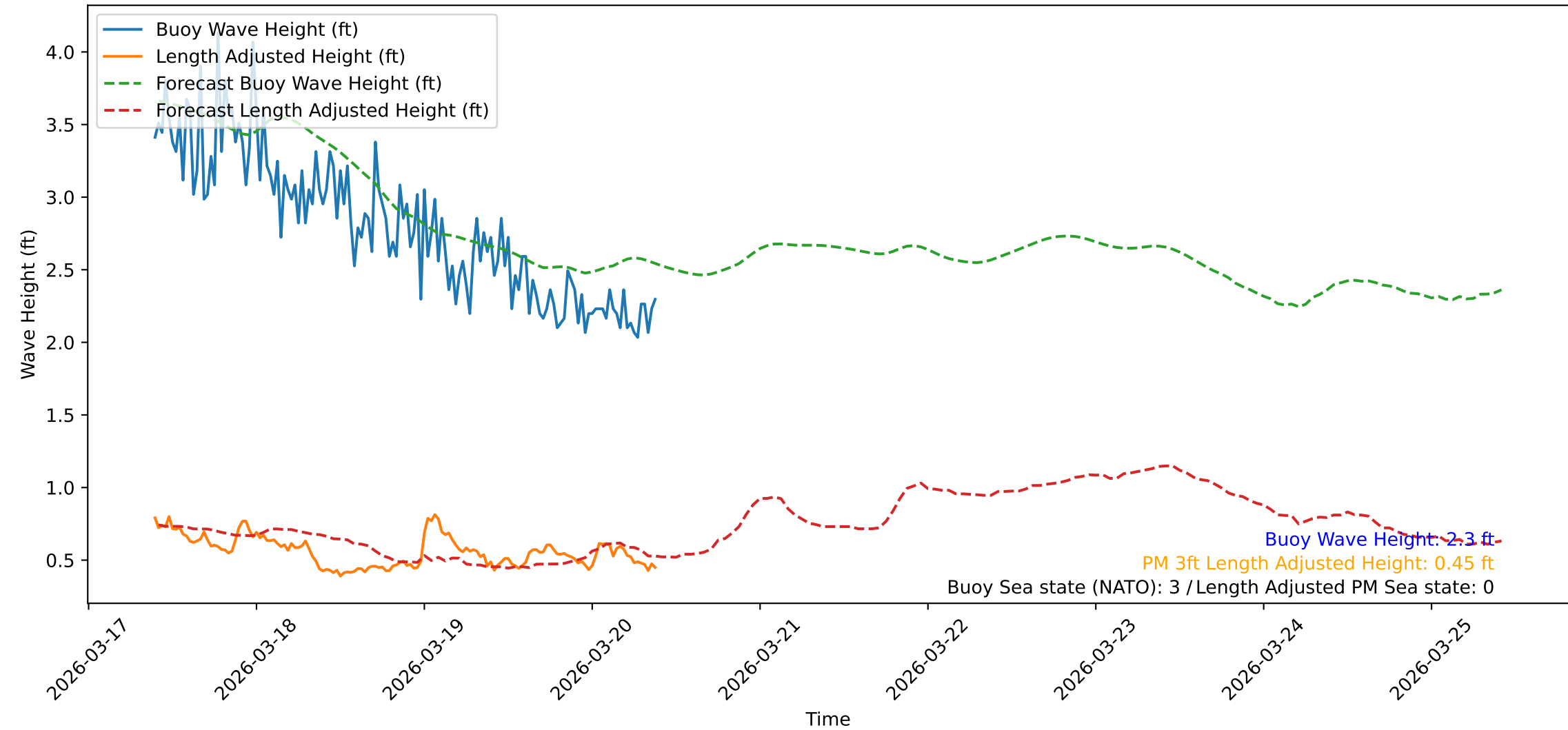
Wave Heights over Time for Green Beach at 2026-03-20 09:41:10
