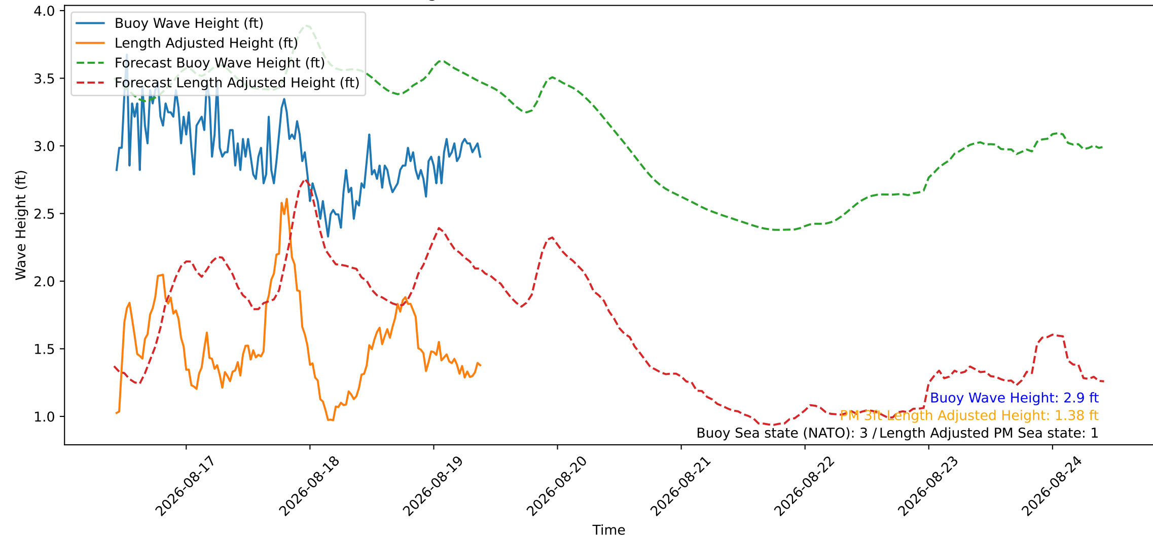
Wave Heights over Time for Red Beach at 2026-08-19 10:00:46
