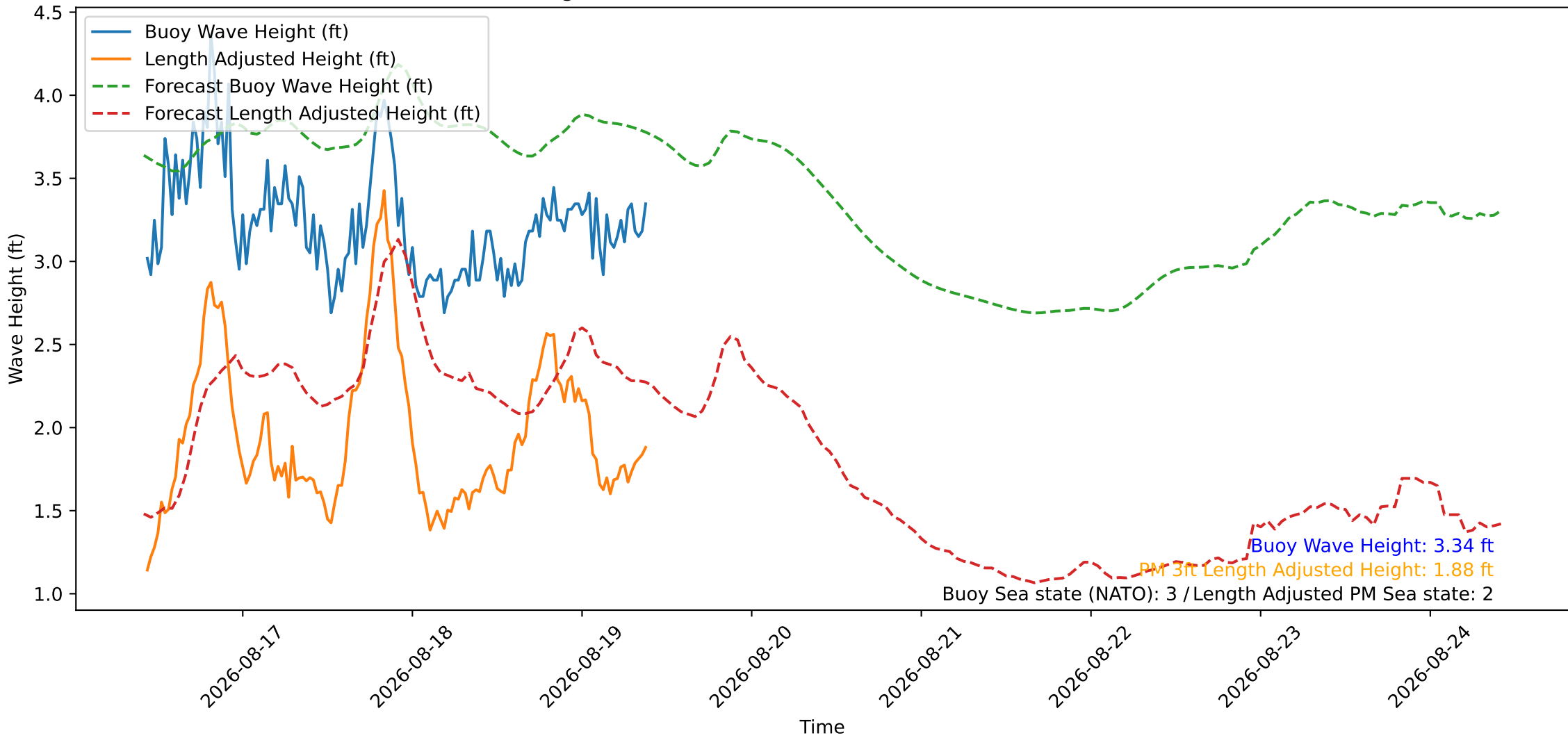
Wave Heights over Time for Green Beach at 2026-08-19 10:01:09
