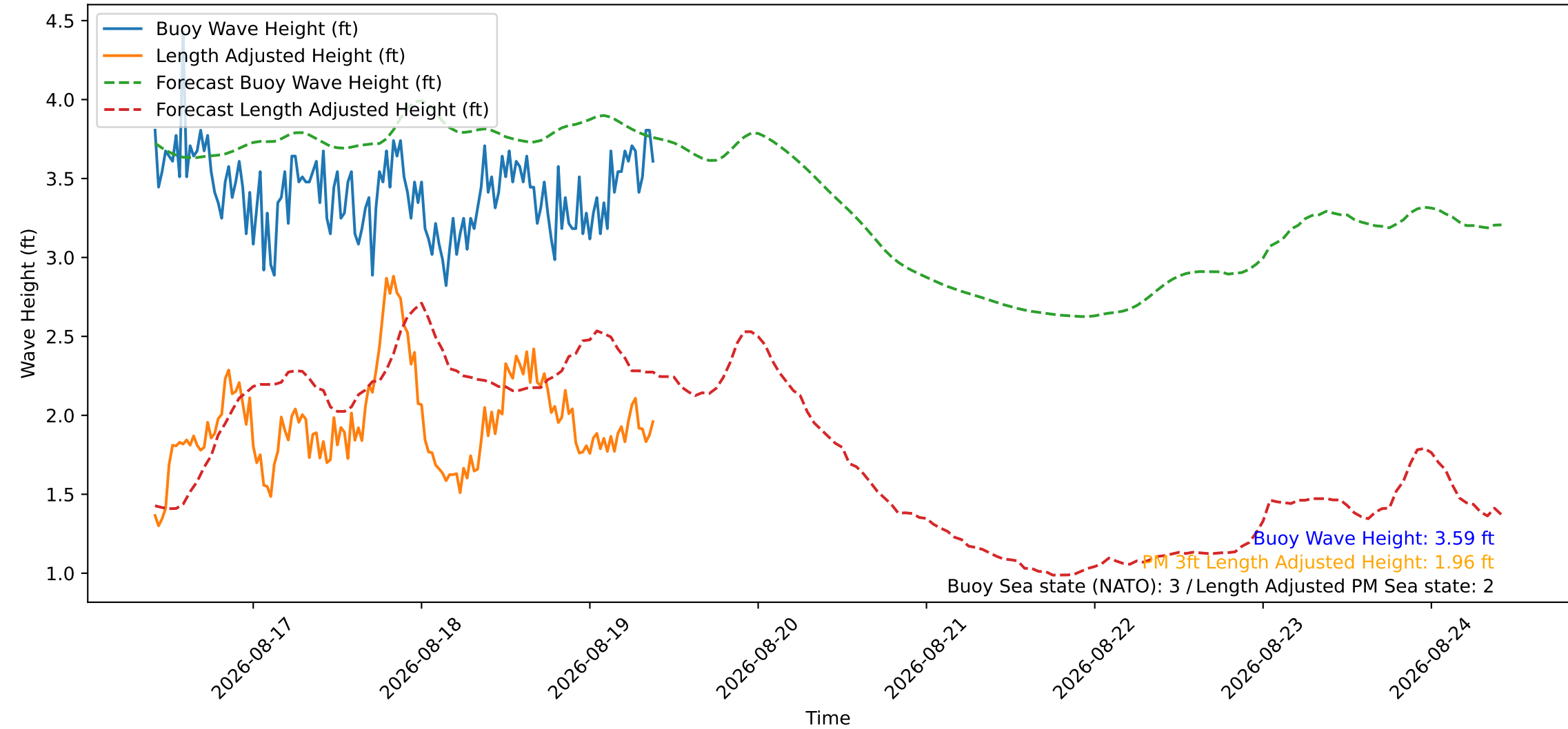
Wave Heights over Time for Oceanside Harbor at 2026-08-19 10:00:26
