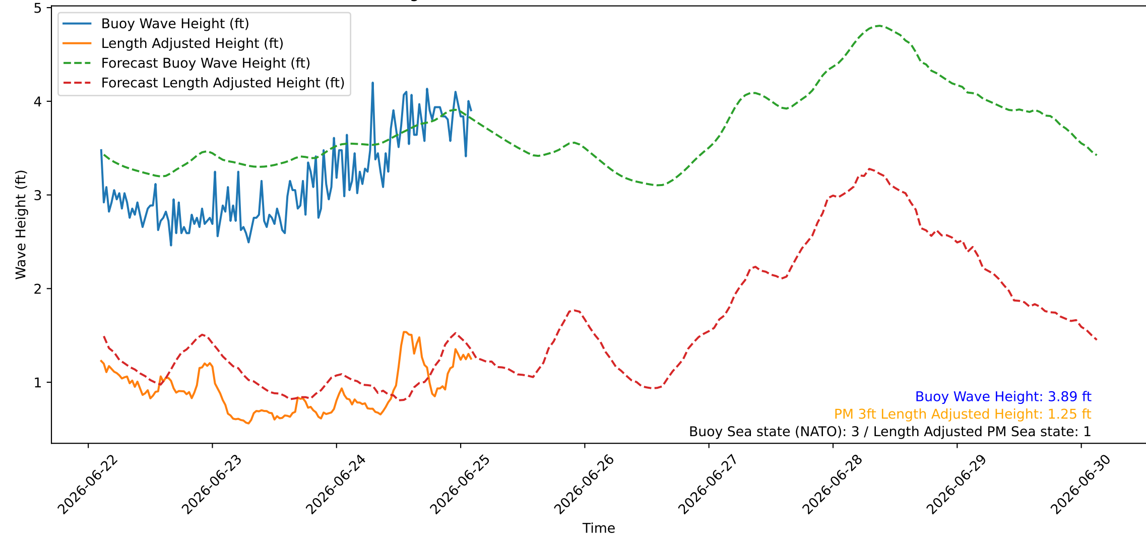
Wave Heights over Time for Green Beach at 2026-06-25 02:41:07
