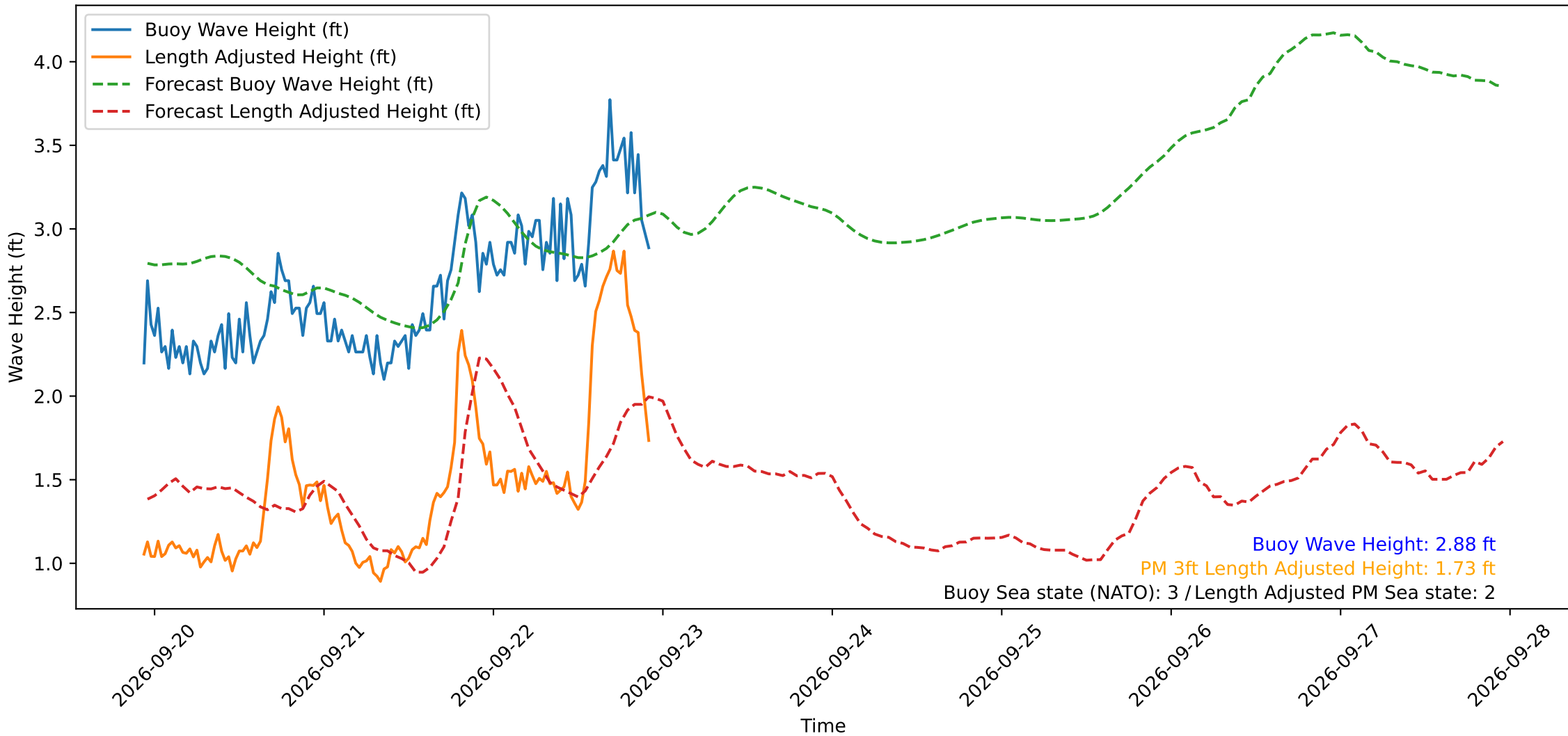
Wave Heights over Time for Oceanside Harbor at 2026-09-22 22:40:29
