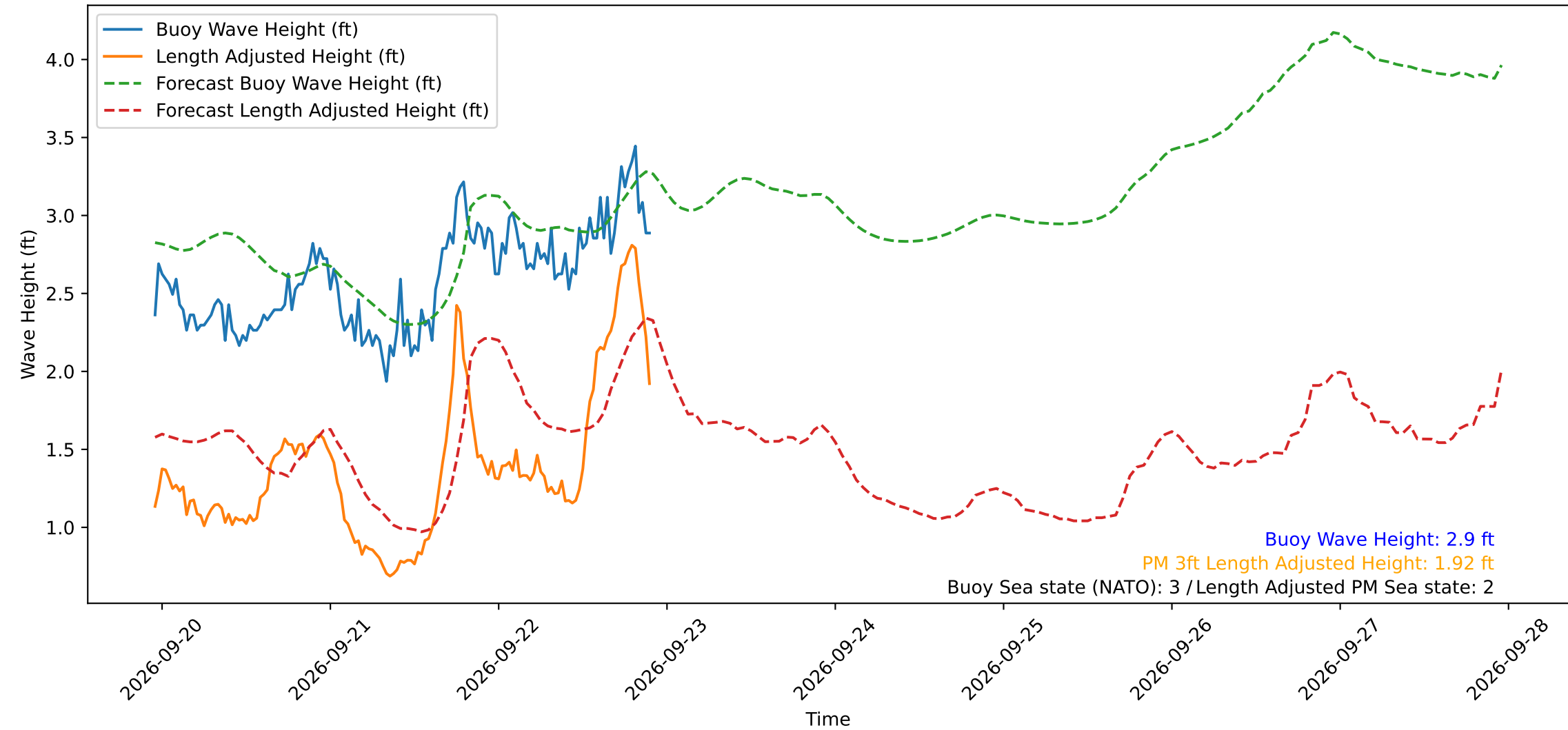
Wave Heights over Time for Green Beach at 2026-09-22 22:41:11
