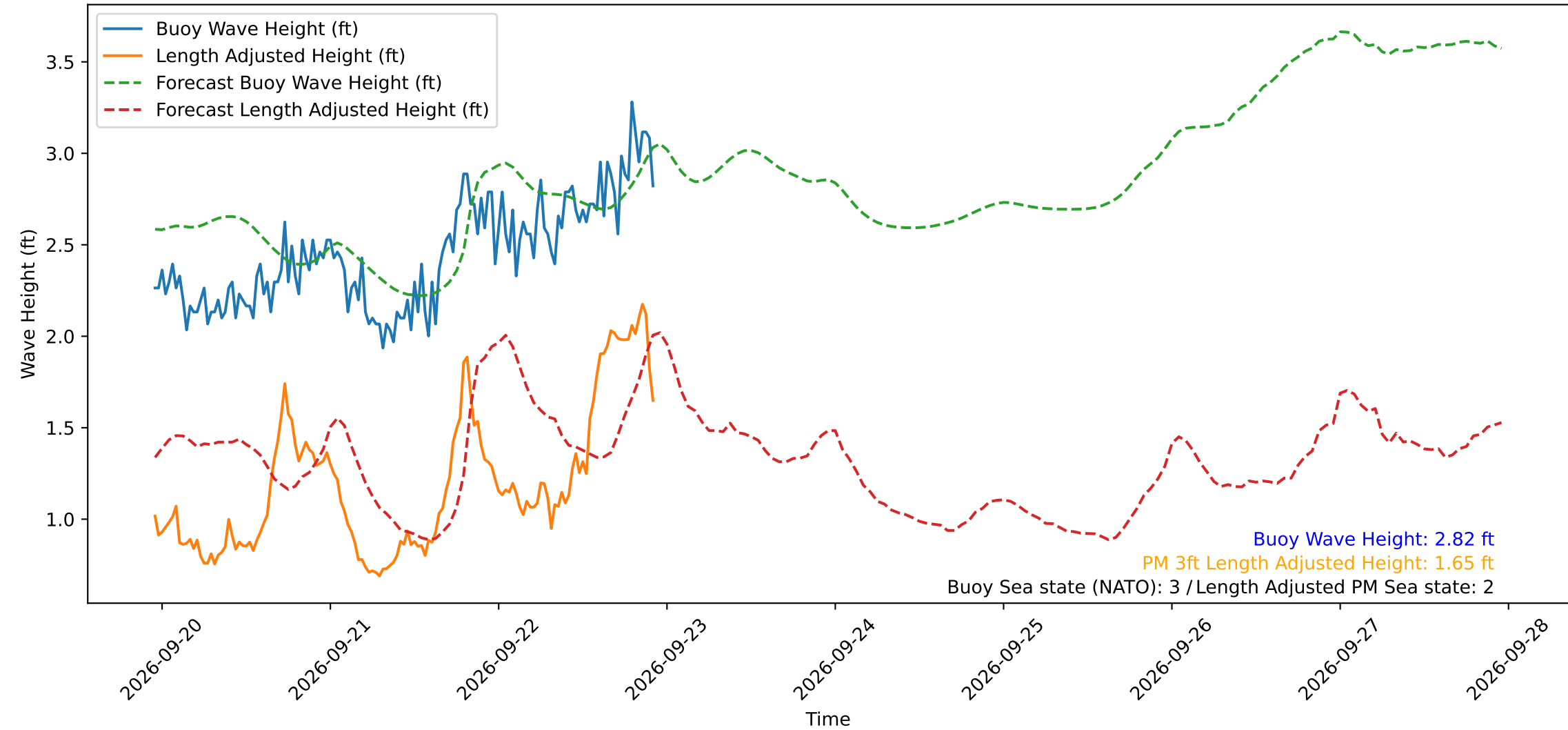
Wave Heights over Time for Red Beach at 2026-09-22 22:40:48
