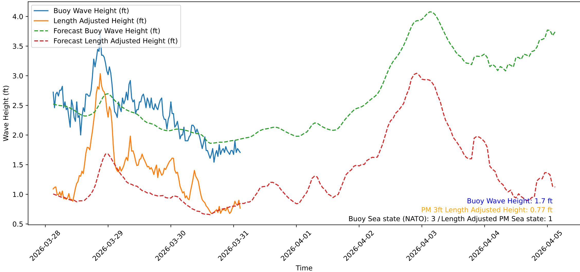
Wave Heights over Time for Green Beach at 2026-03-31 03:11:10
