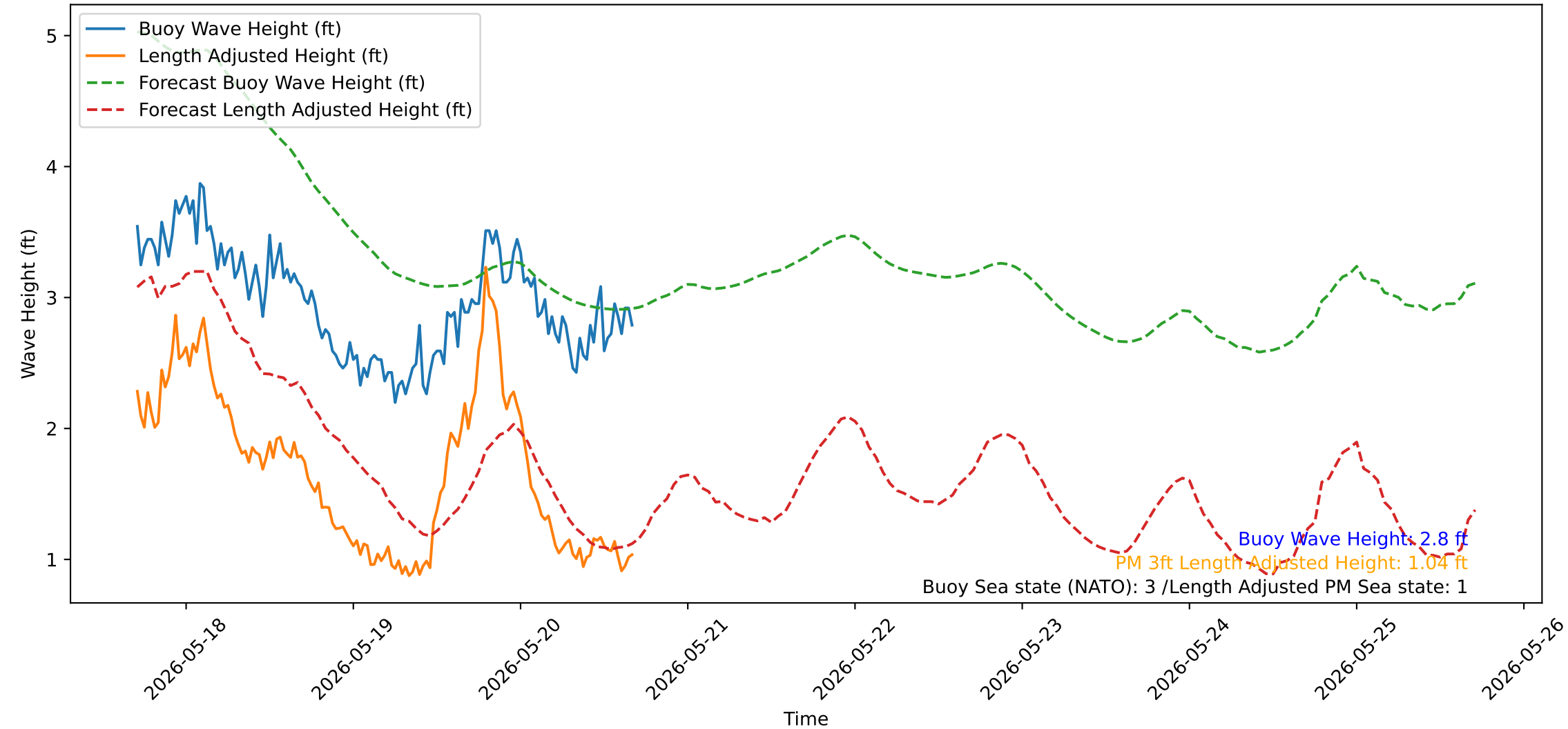
Wave Heights over Time for Oceanside Harbor at 2026-05-20 17:00:32
