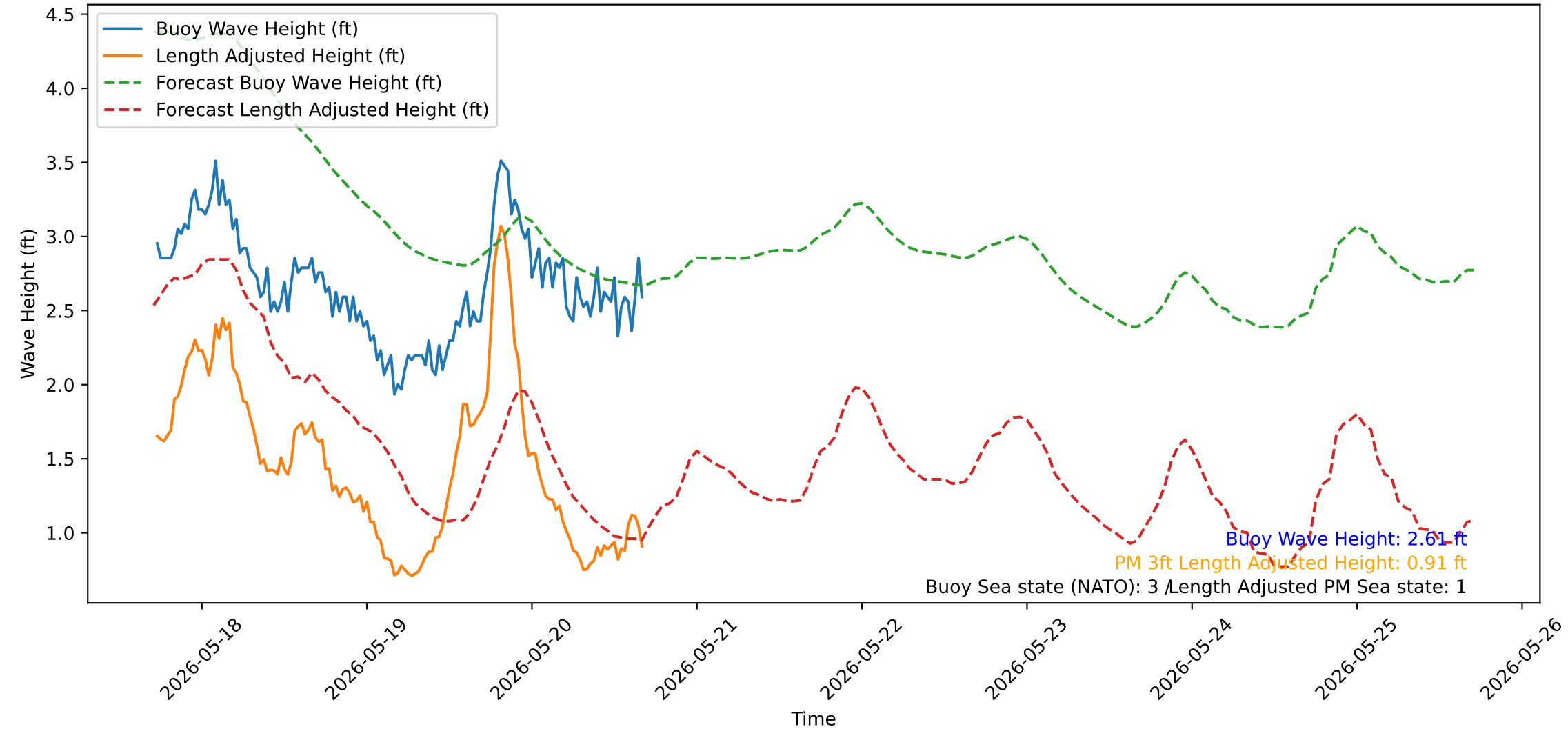
Wave Heights over Time for Red Beach at 2026-05-20 17:00:52
