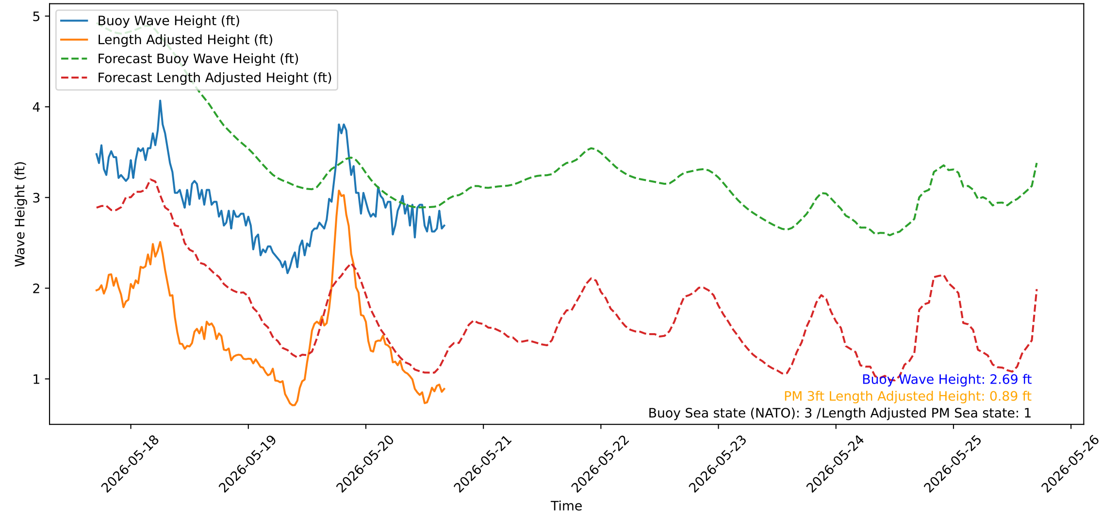
Wave Heights over Time for Green Beach at 2026-05-20 17:01:14
