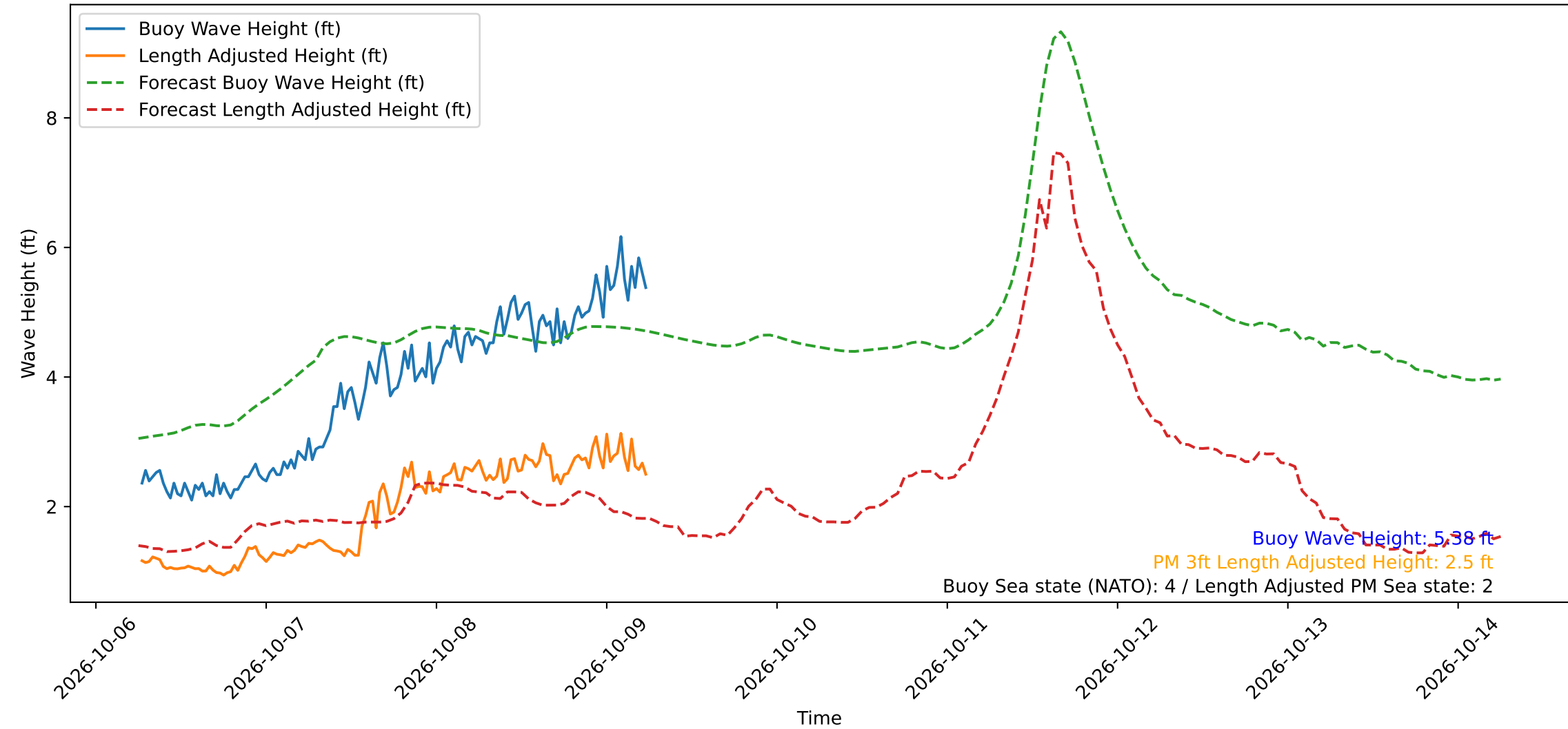
Wave Heights over Time for Green Beach at 2026-10-09 06:21:14
