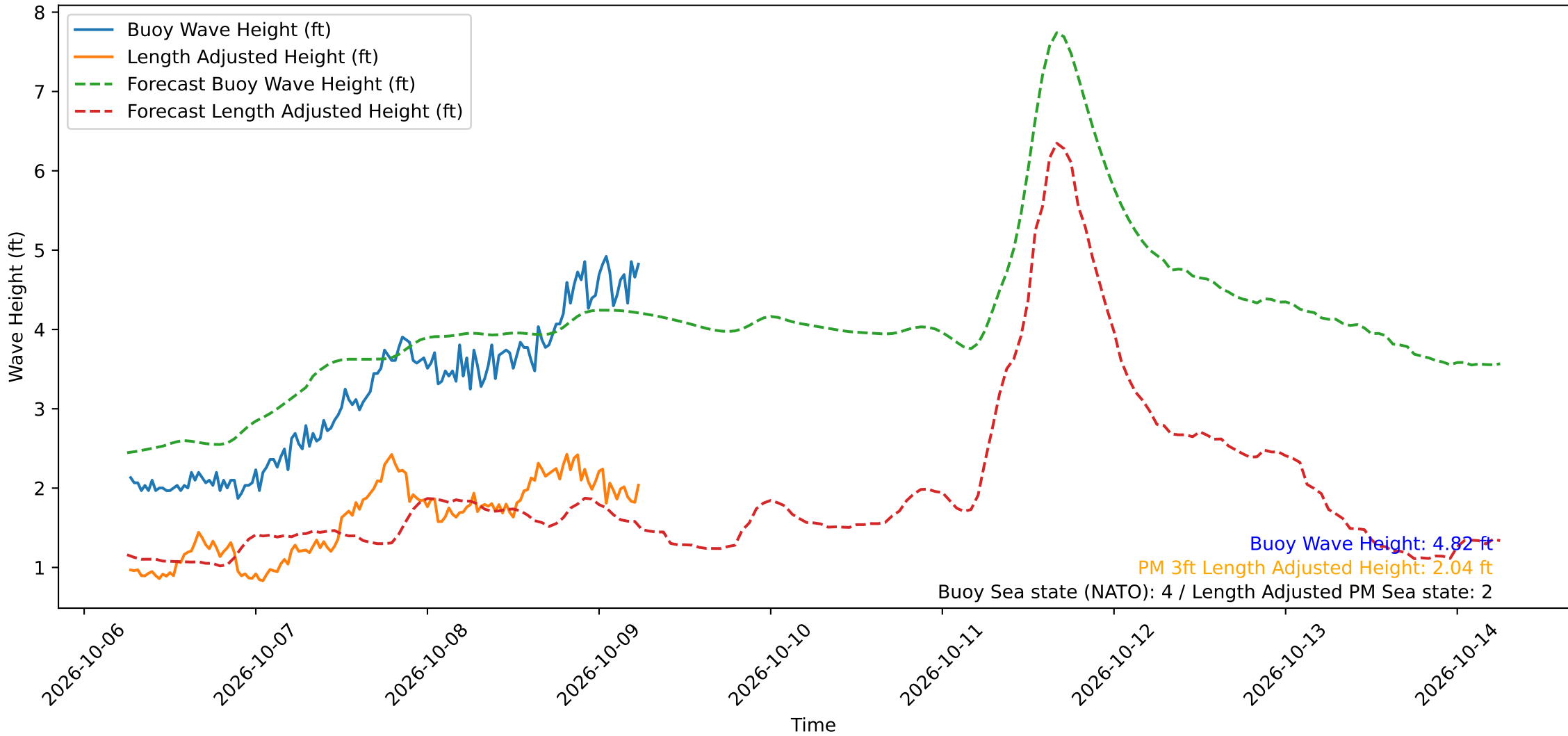
Wave Heights over Time for Red Beach at 2026-10-09 06:20:50
