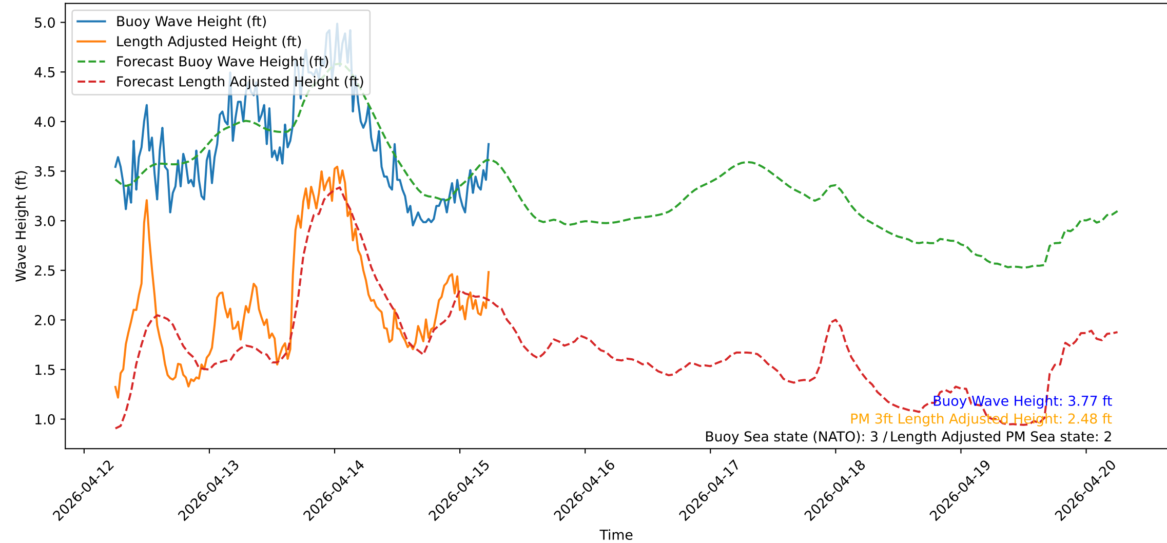
Wave Heights over Time for Green Beach at 2026-04-15 06:11:14
