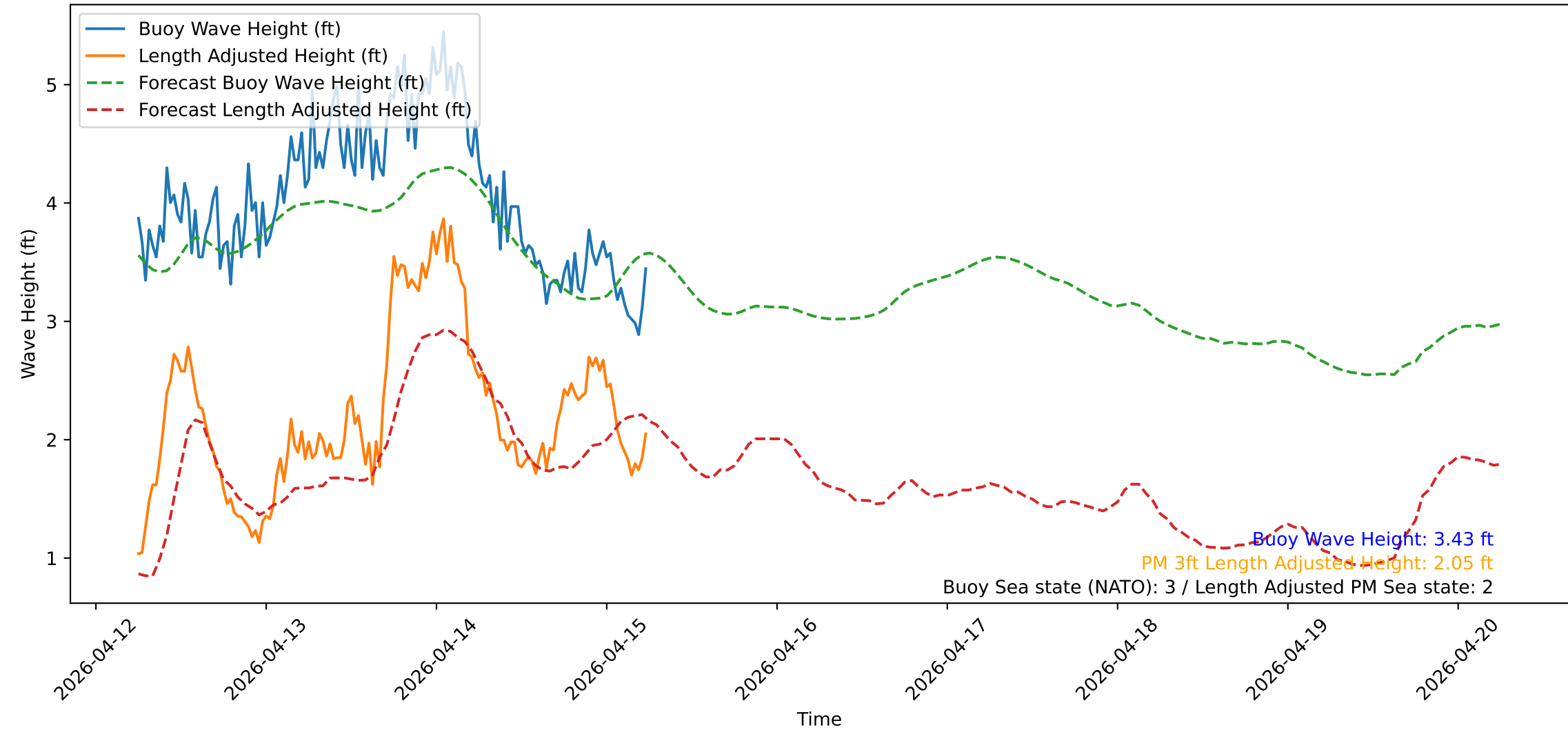
Wave Heights over Time for Oceanside Harbor at 2026-04-15 06:10:32
