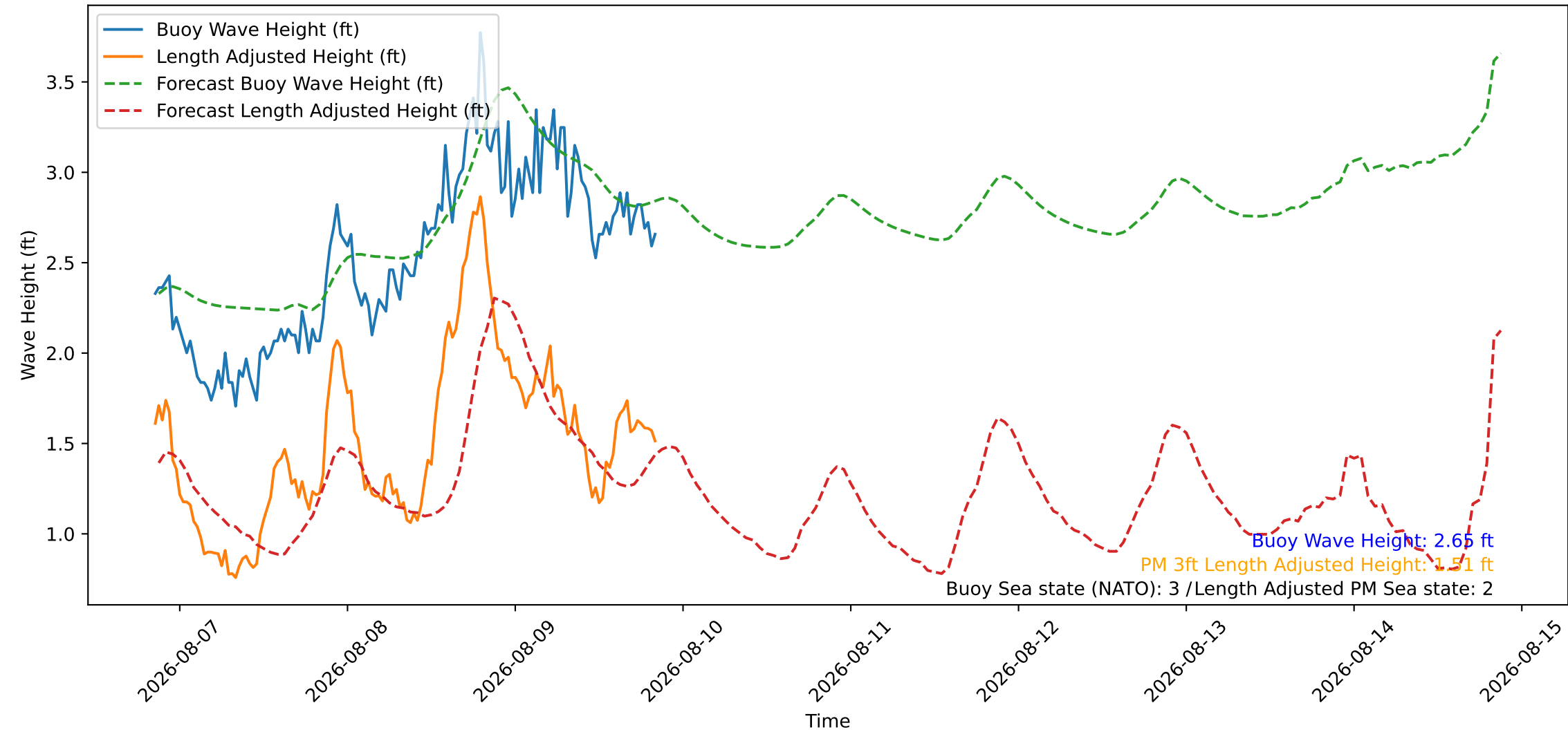
Wave Heights over Time for Green Beach at 2026-08-09 20:41:09
