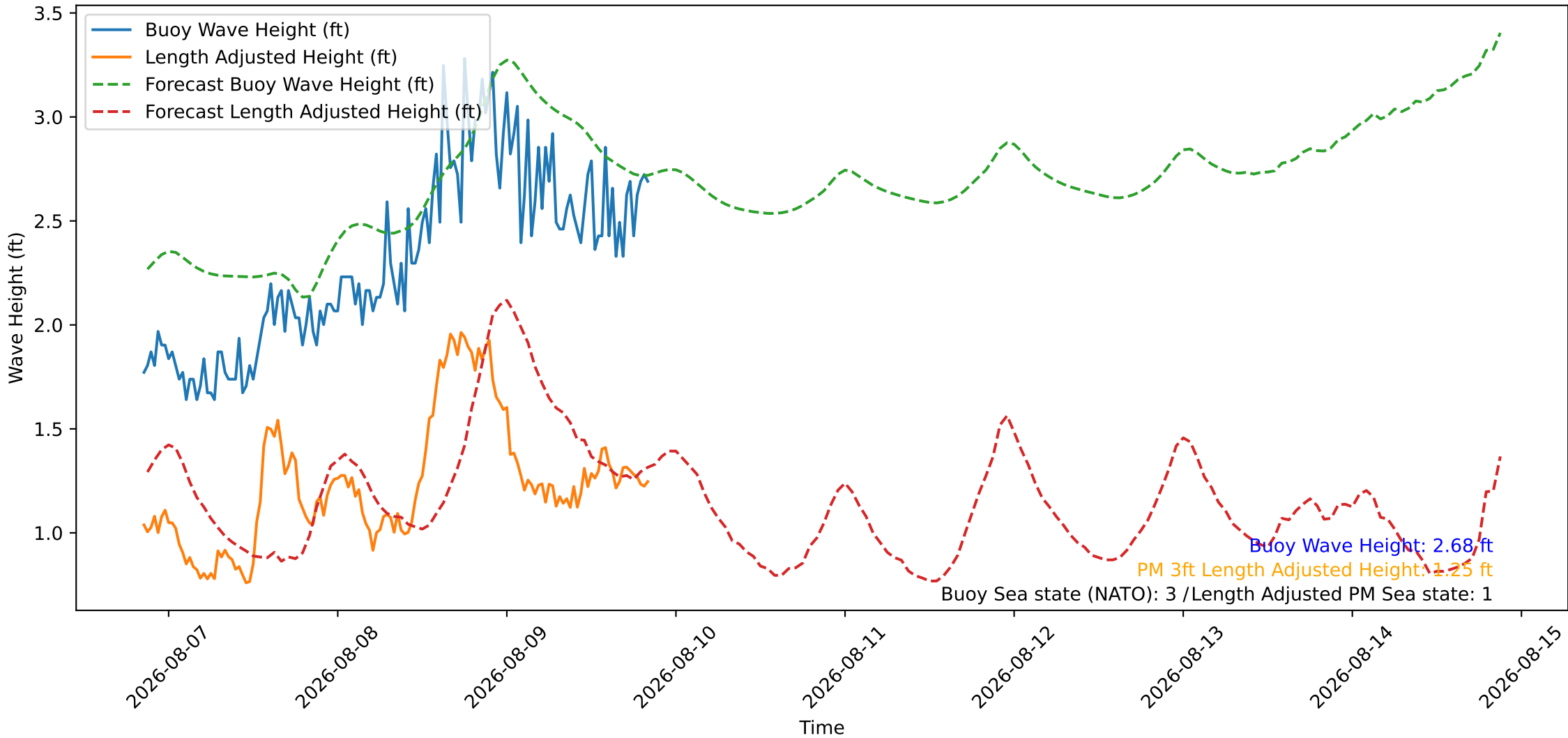
Wave Heights over Time for Oceanside Harbor at 2026-08-09 20:40:26
