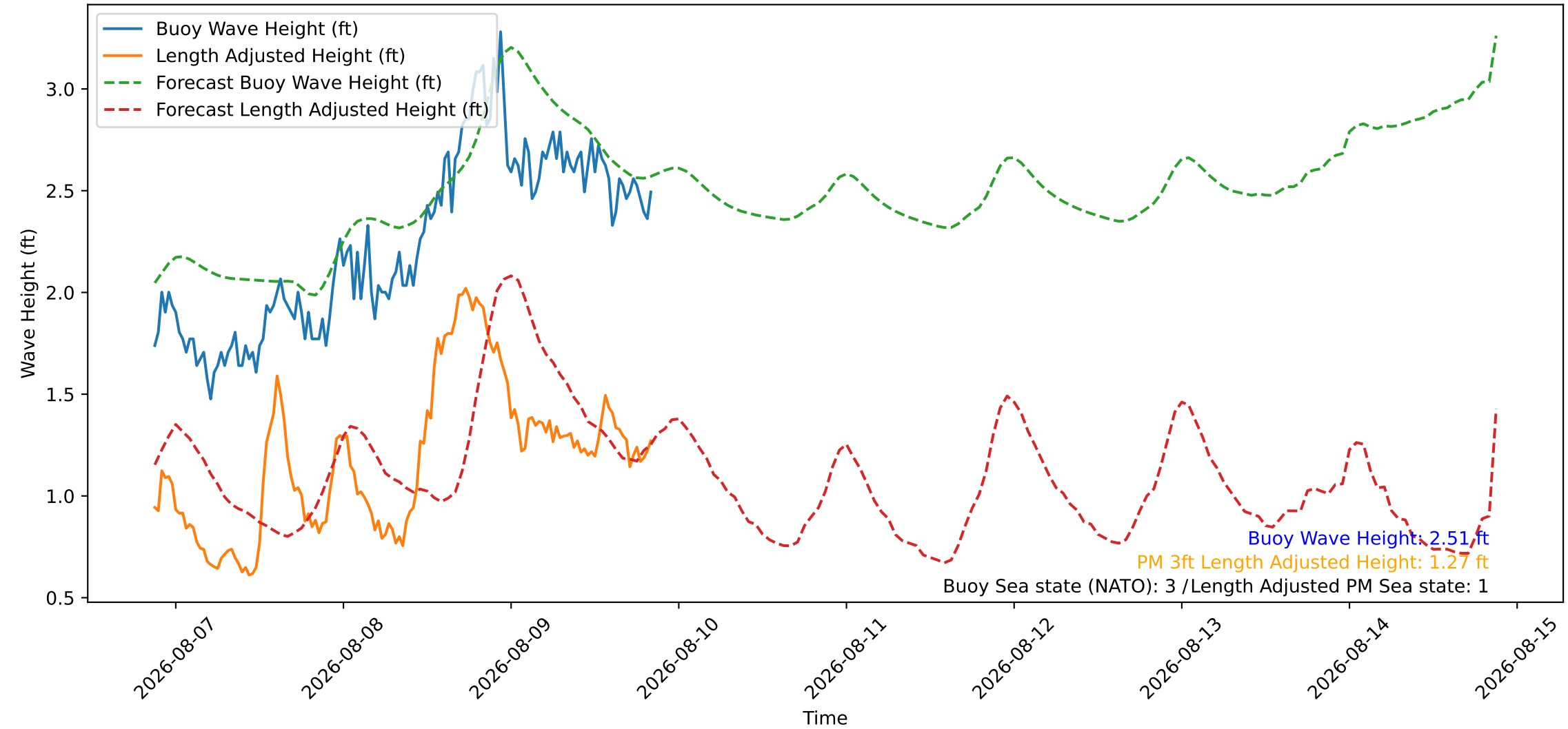
Wave Heights over Time for Red Beach at 2026-08-09 20:40:46
