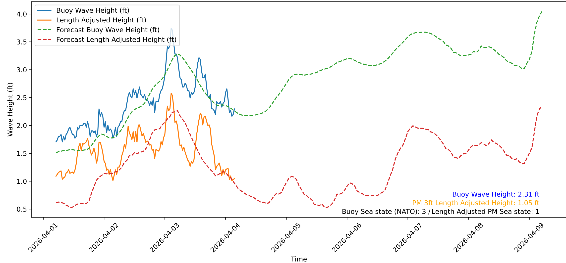
Wave Heights over Time for Red Beach at 2026-04-04 04:30:48
