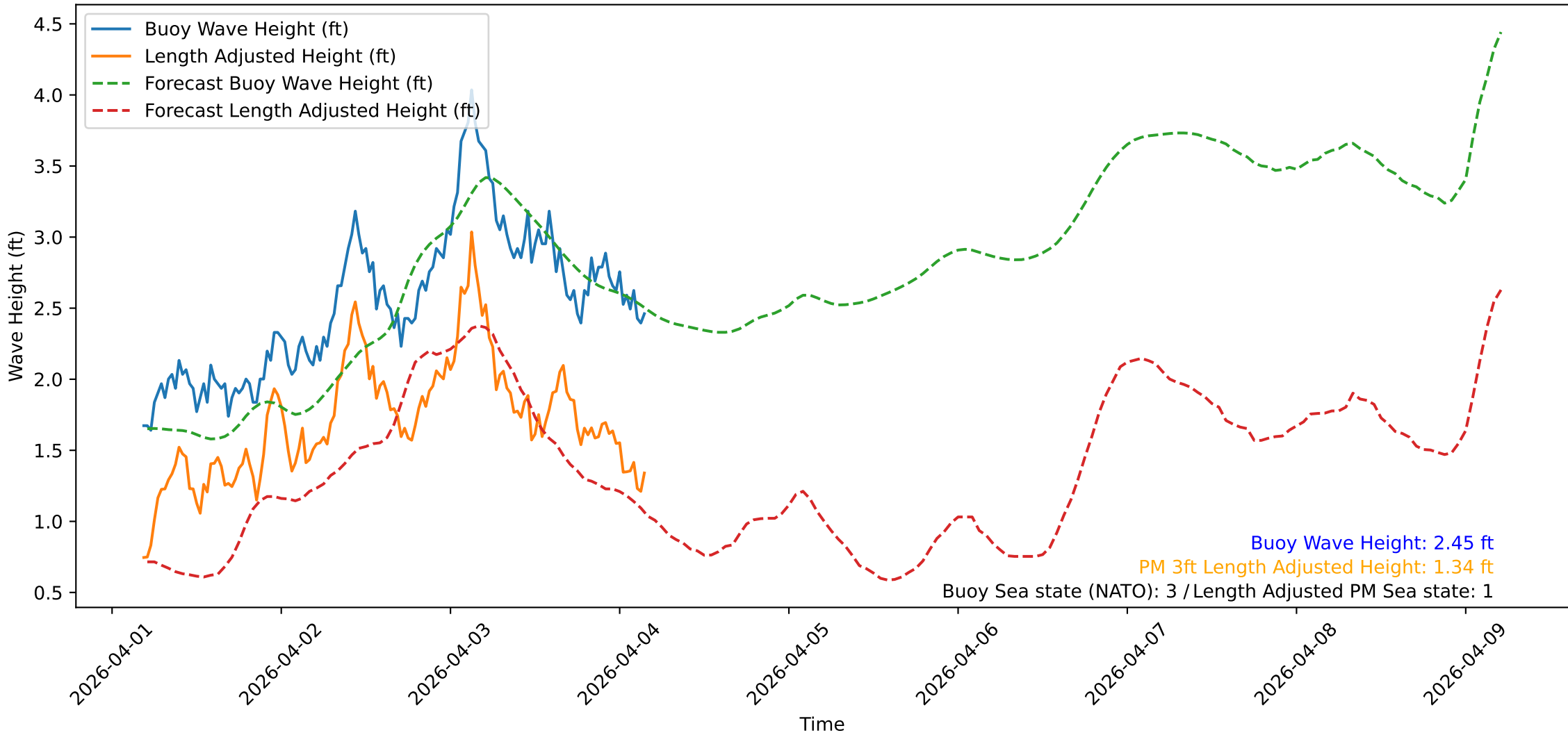
Wave Heights over Time for Oceanside Harbor at 2026-04-04 04:30:32
