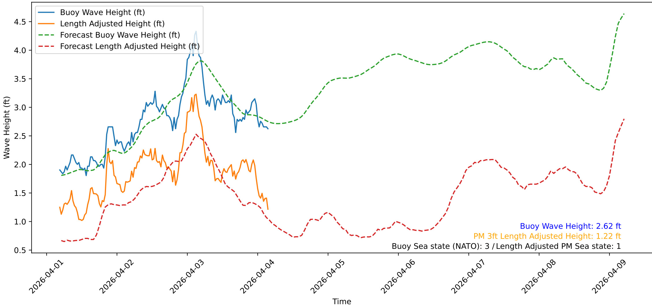
Wave Heights over Time for Green Beach at 2026-04-04 04:31:10
