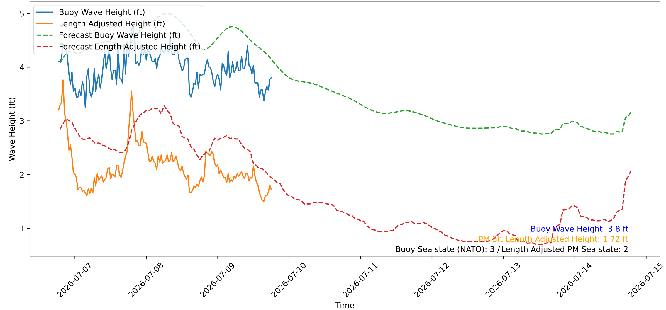
Wave Heights over Time for Green Beach at 2026-07-09 18:41:08
