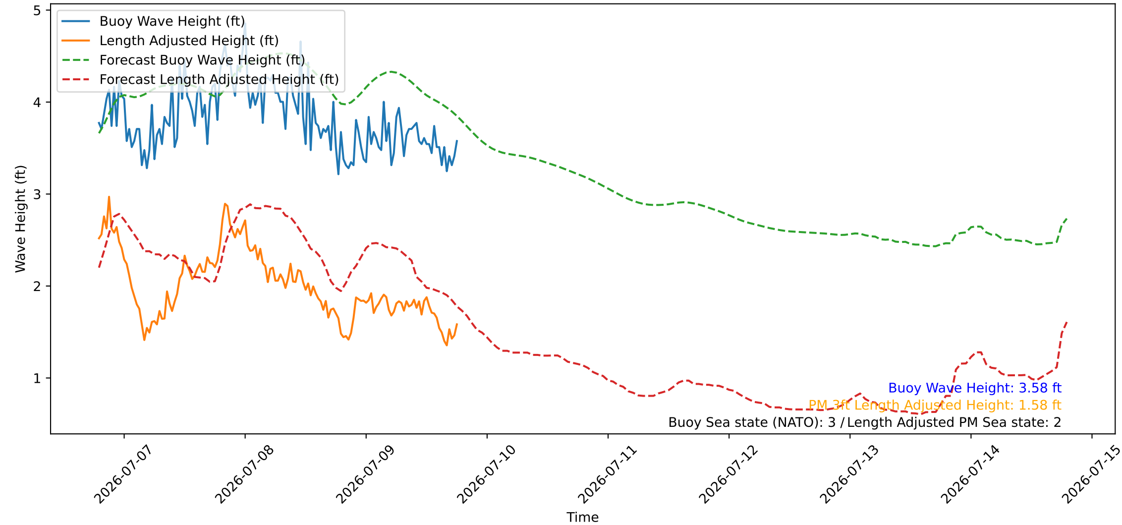
Wave Heights over Time for Red Beach at 2026-07-09 18:40:46
