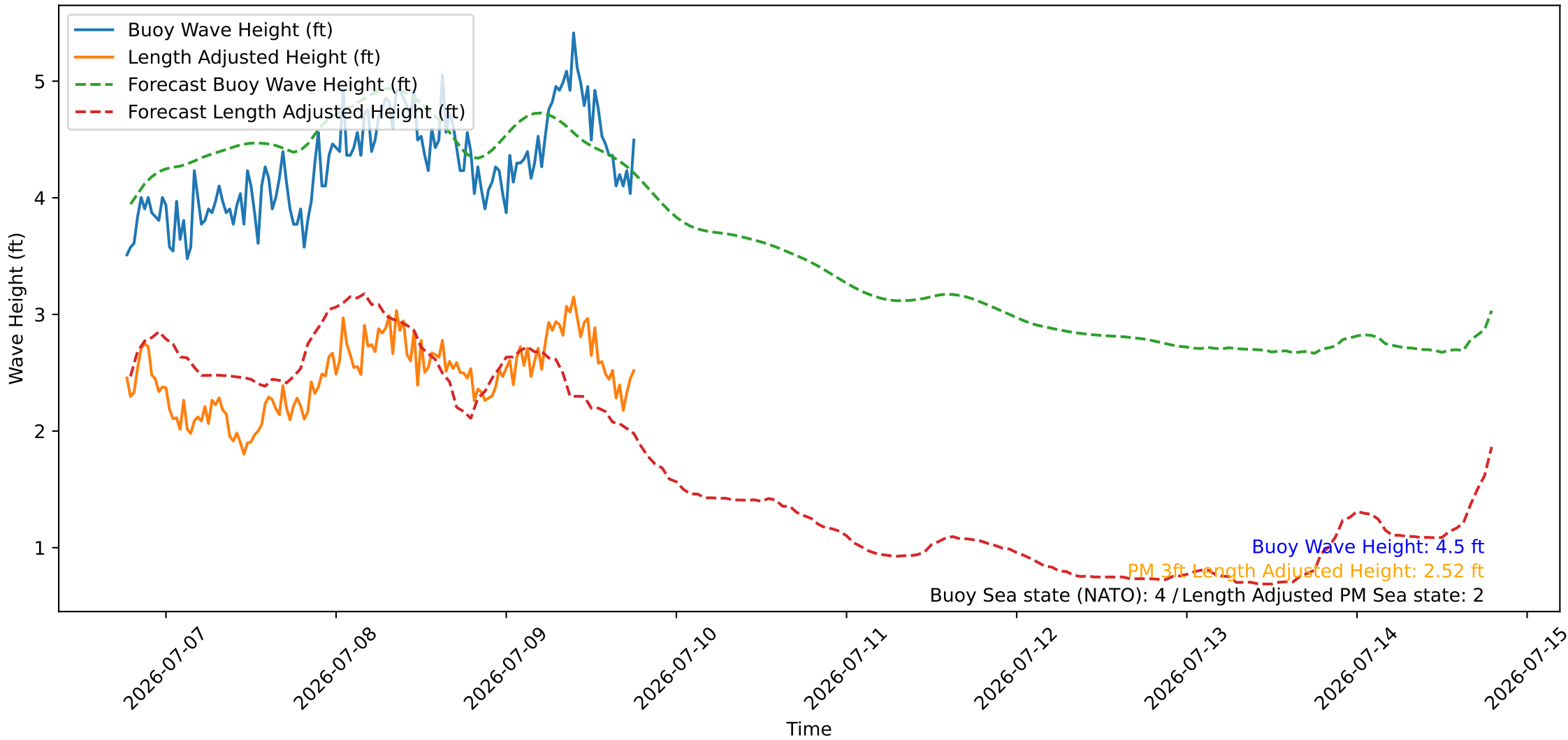
Wave Heights over Time for Oceanside Harbor at 2026-07-09 18:40:26
