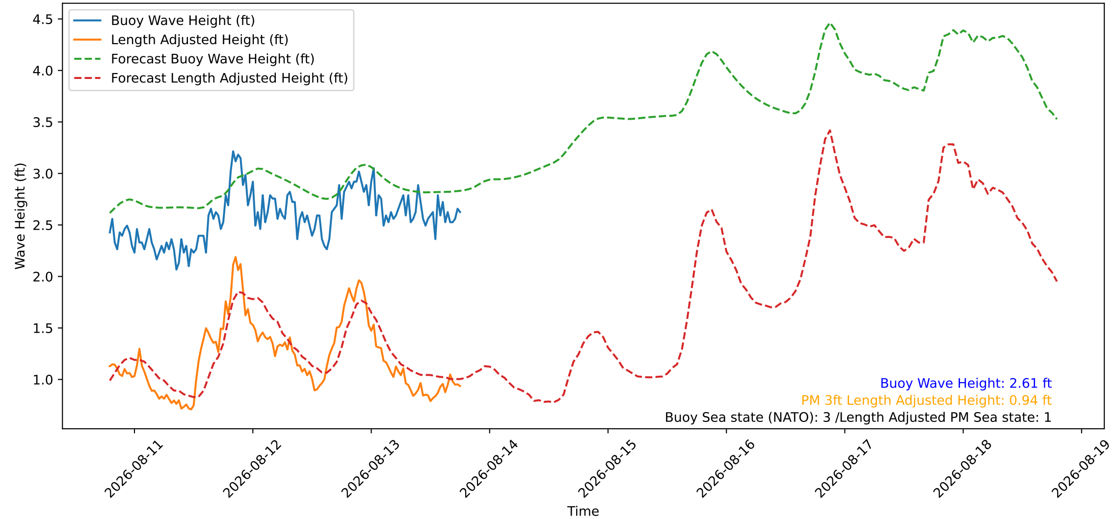
Wave Heights over Time for Green Beach at 2026-08-13 19:11:08
