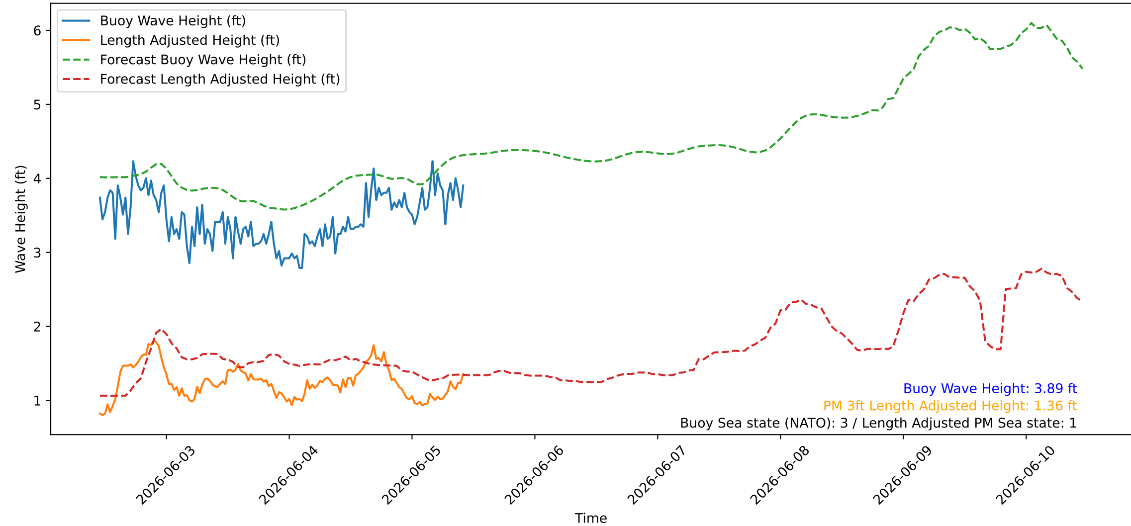
Wave Heights over Time for Green Beach at 2026-06-05 11:01:07
