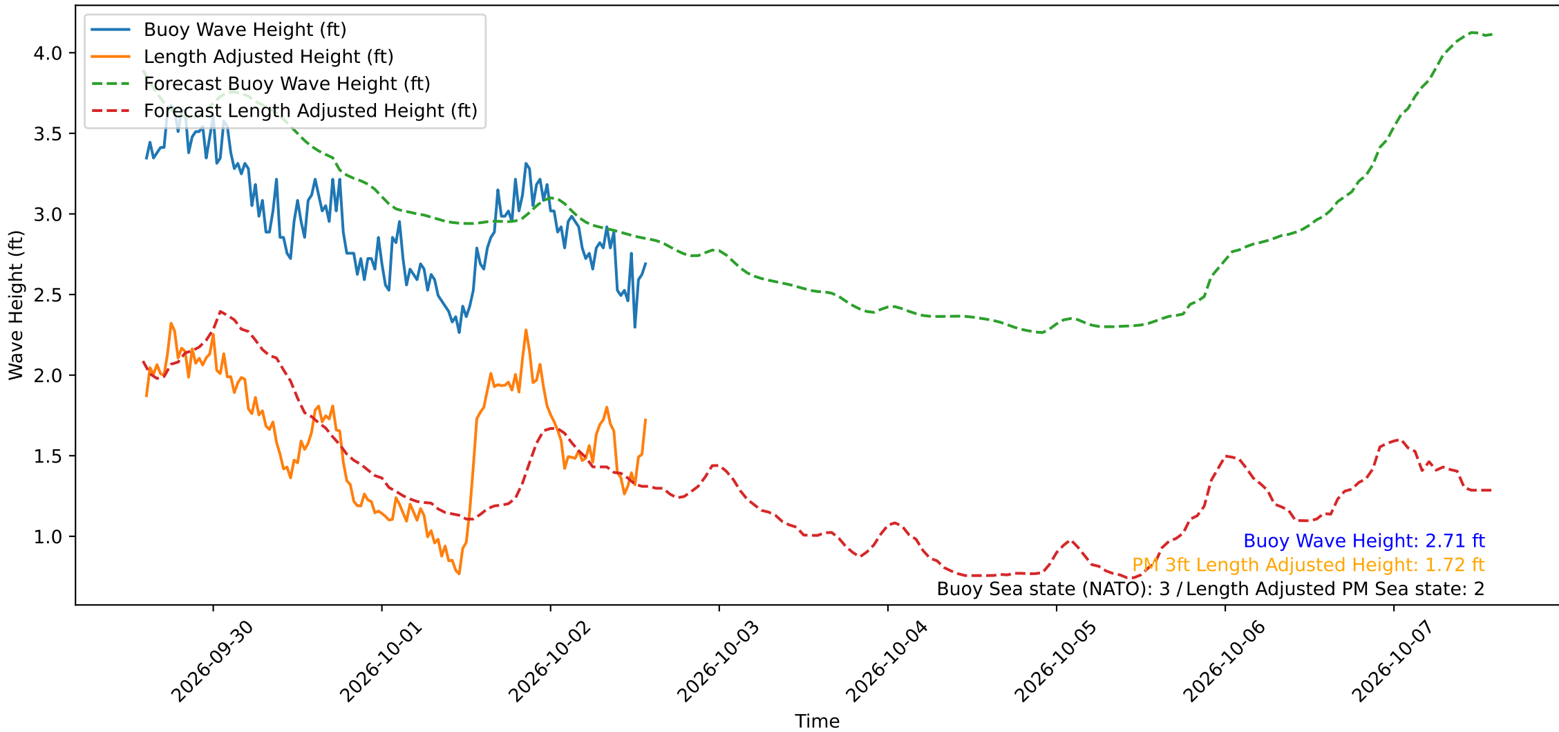
Wave Heights over Time for Oceanside Harbor at 2026-10-02 14:20:30
