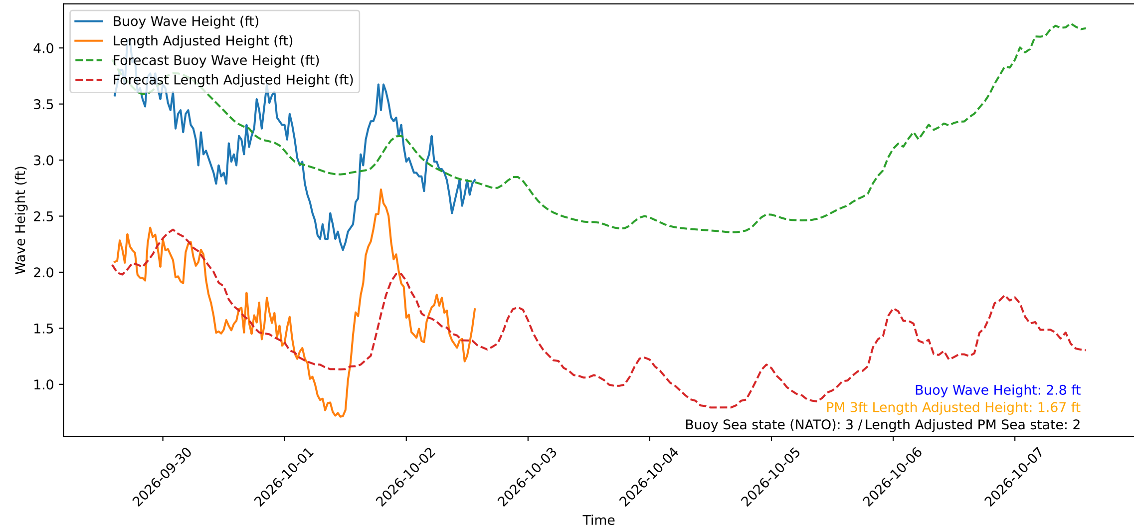
Wave Heights over Time for Green Beach at 2026-10-02 14:21:15
