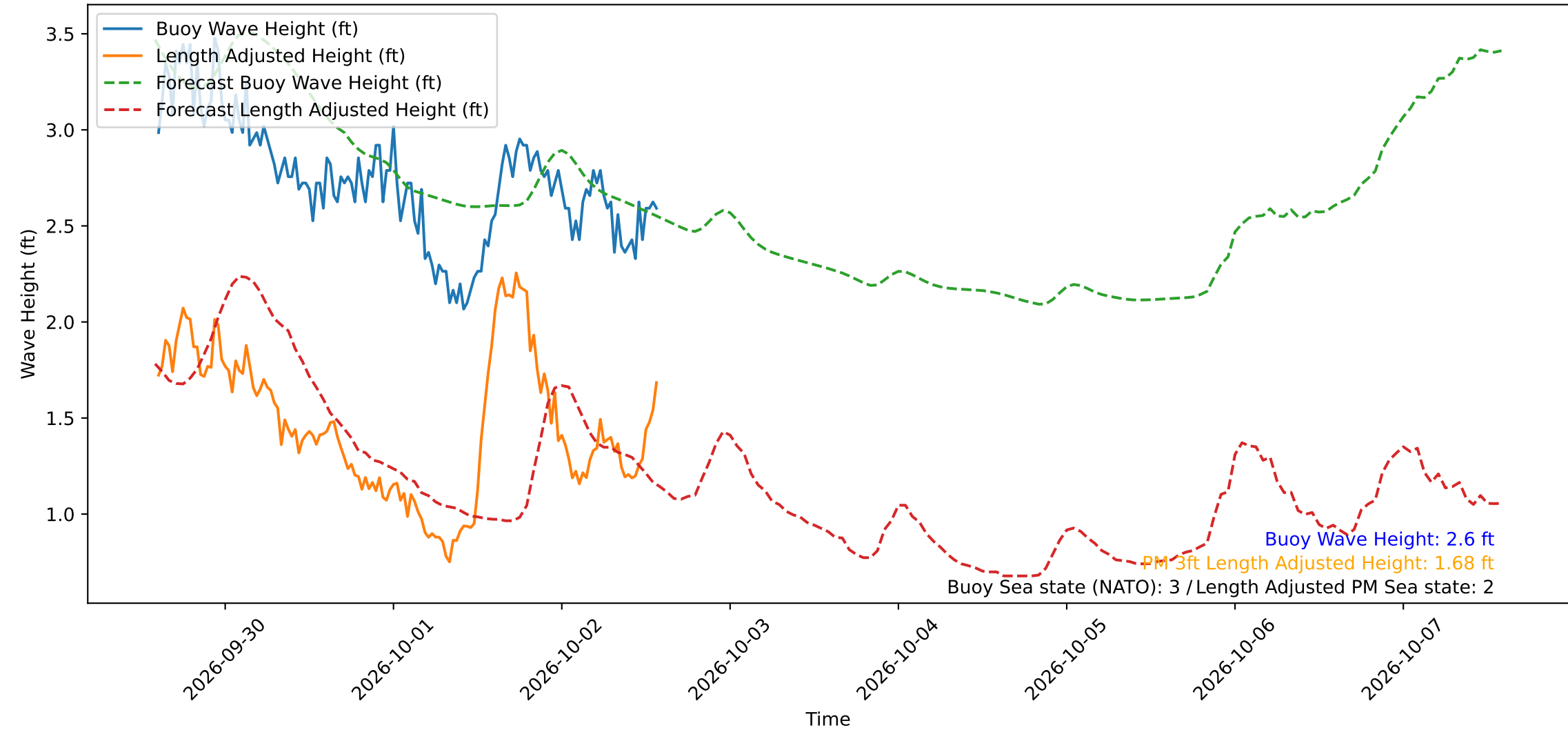
Wave Heights over Time for Red Beach at 2026-10-02 14:20:51
