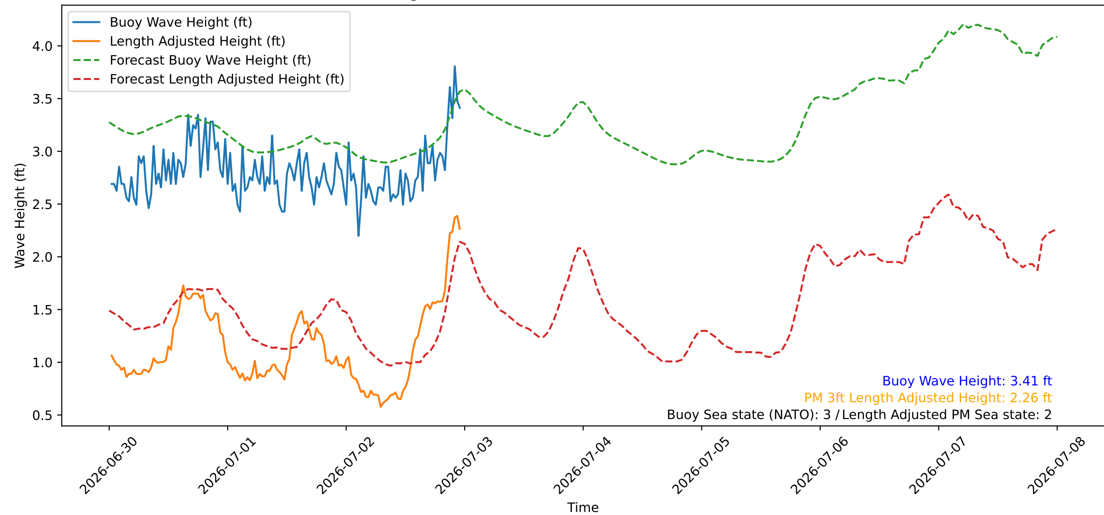
Wave Heights over Time for Red Beach at 2026-07-03 00:00:44
