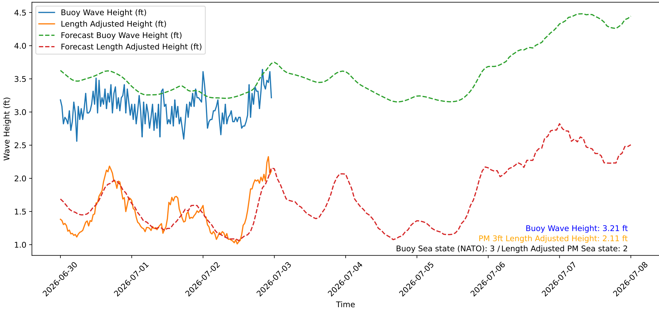
Wave Heights over Time for Oceanside Harbor at 2026-07-03 00:00:26
