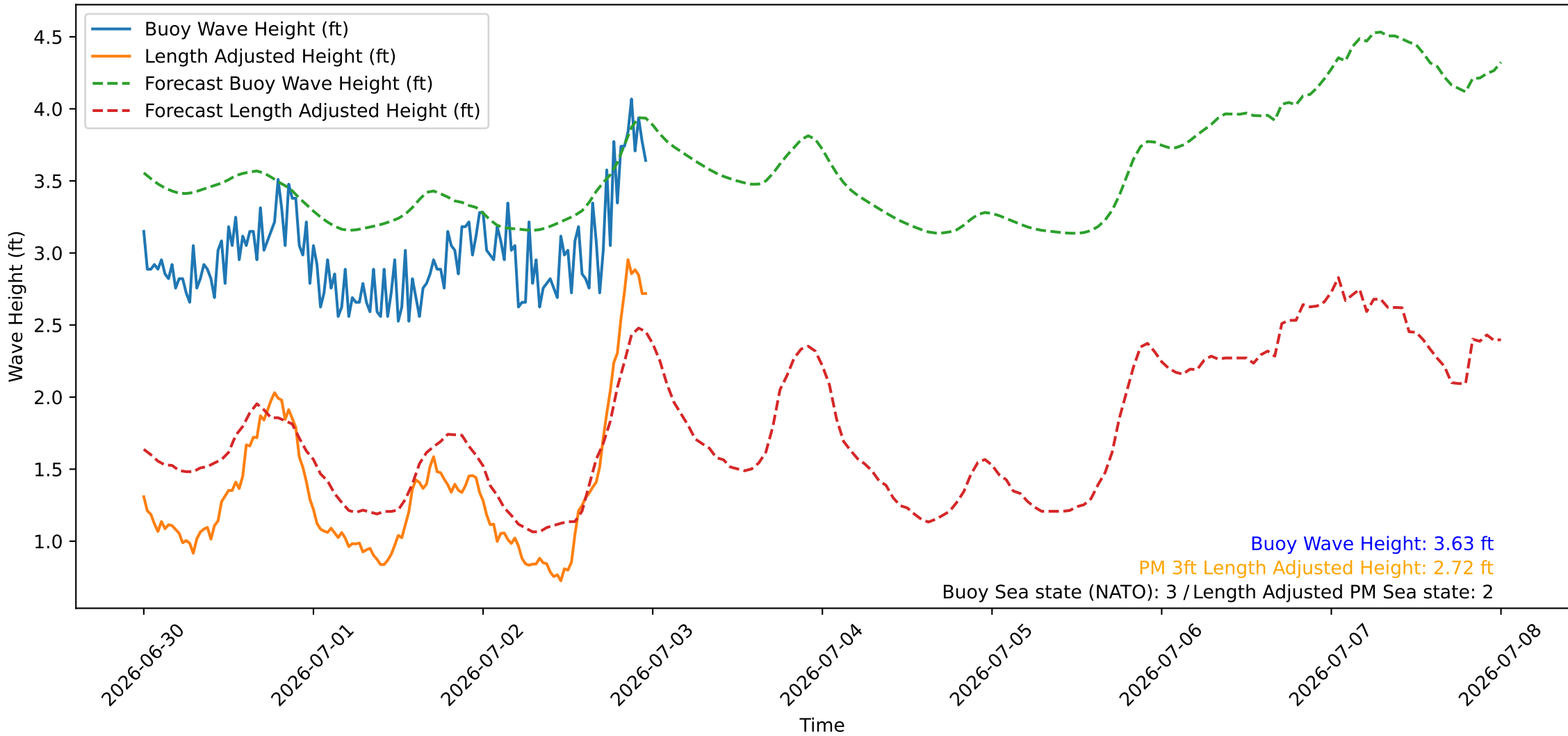
Wave Heights over Time for Green Beach at 2026-07-03 00:01:06
