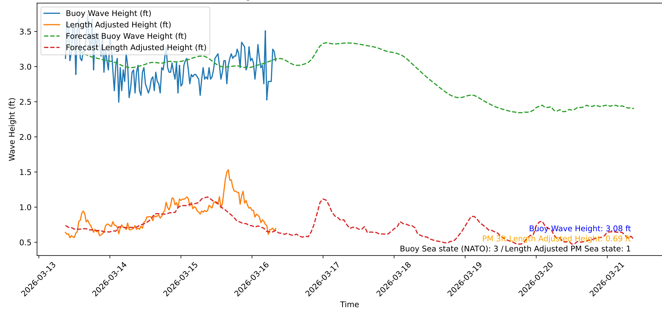
Wave Heights over Time for Red Beach at 2026-03-16 08:51:03
