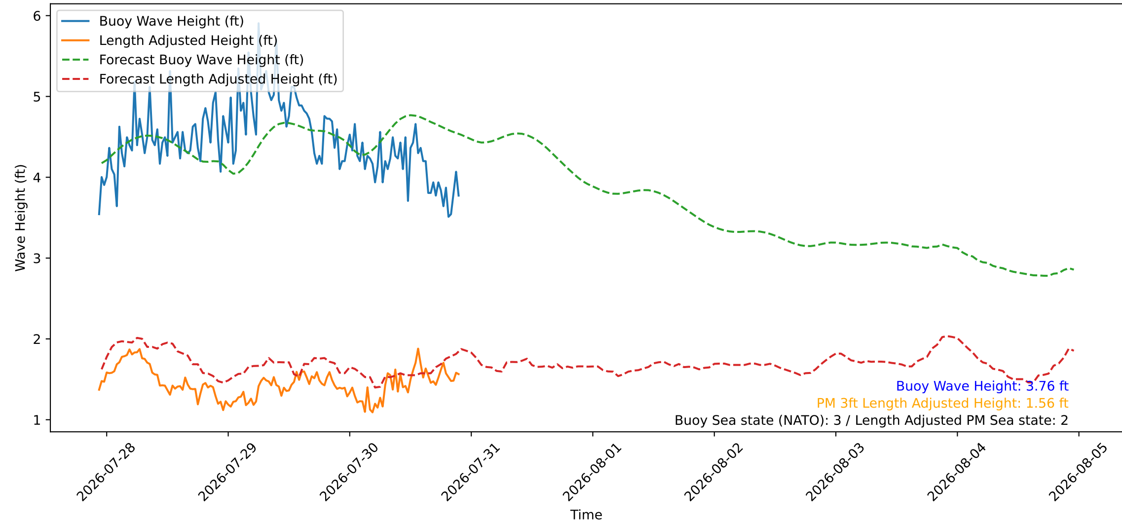
Wave Heights over Time for Oceanside Harbor at 2026-07-30 22:40:26
