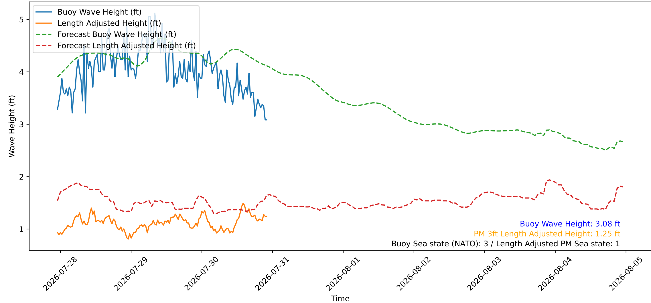
Wave Heights over Time for Red Beach at 2026-07-30 22:40:46
