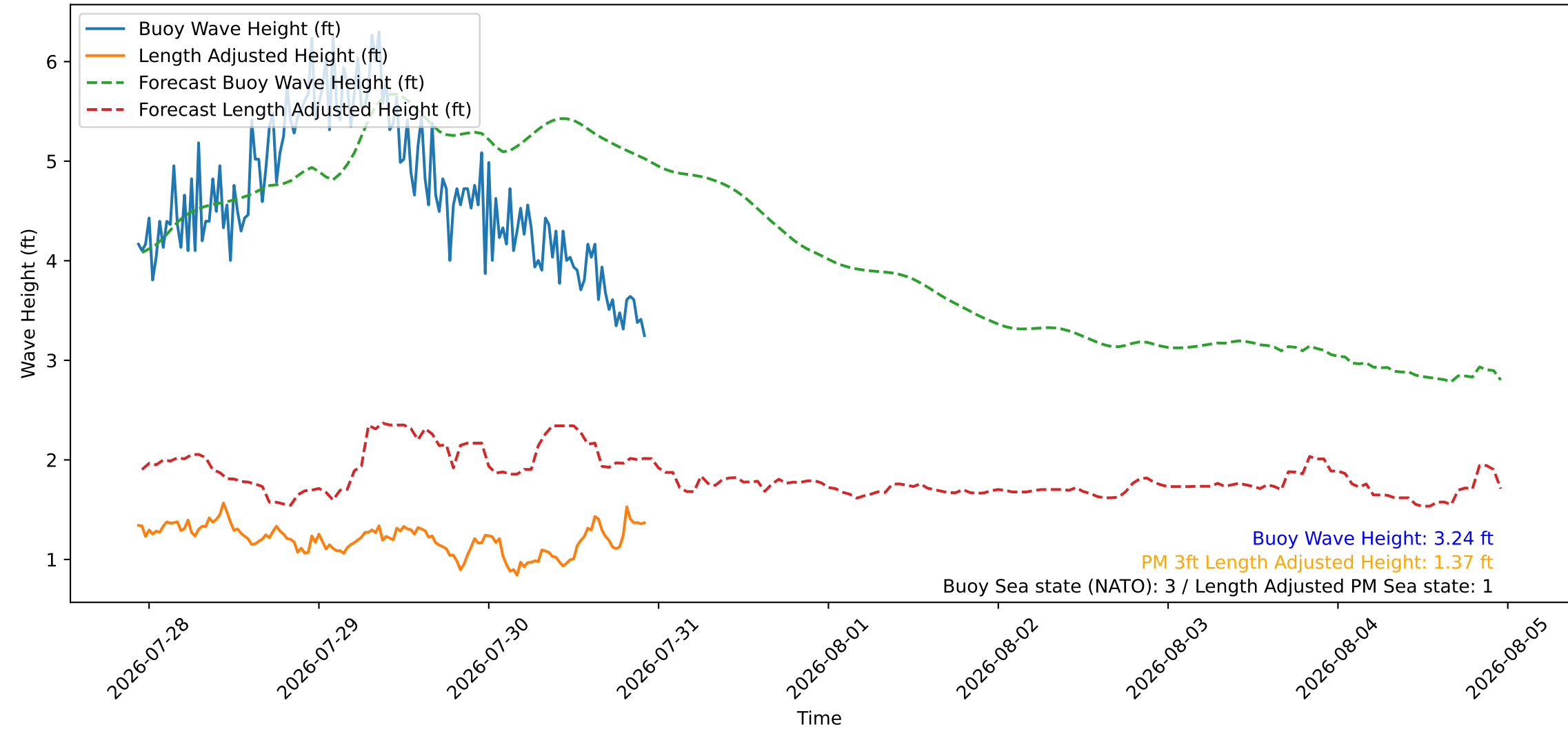
Wave Heights over Time for Green Beach at 2026-07-30 22:41:08
