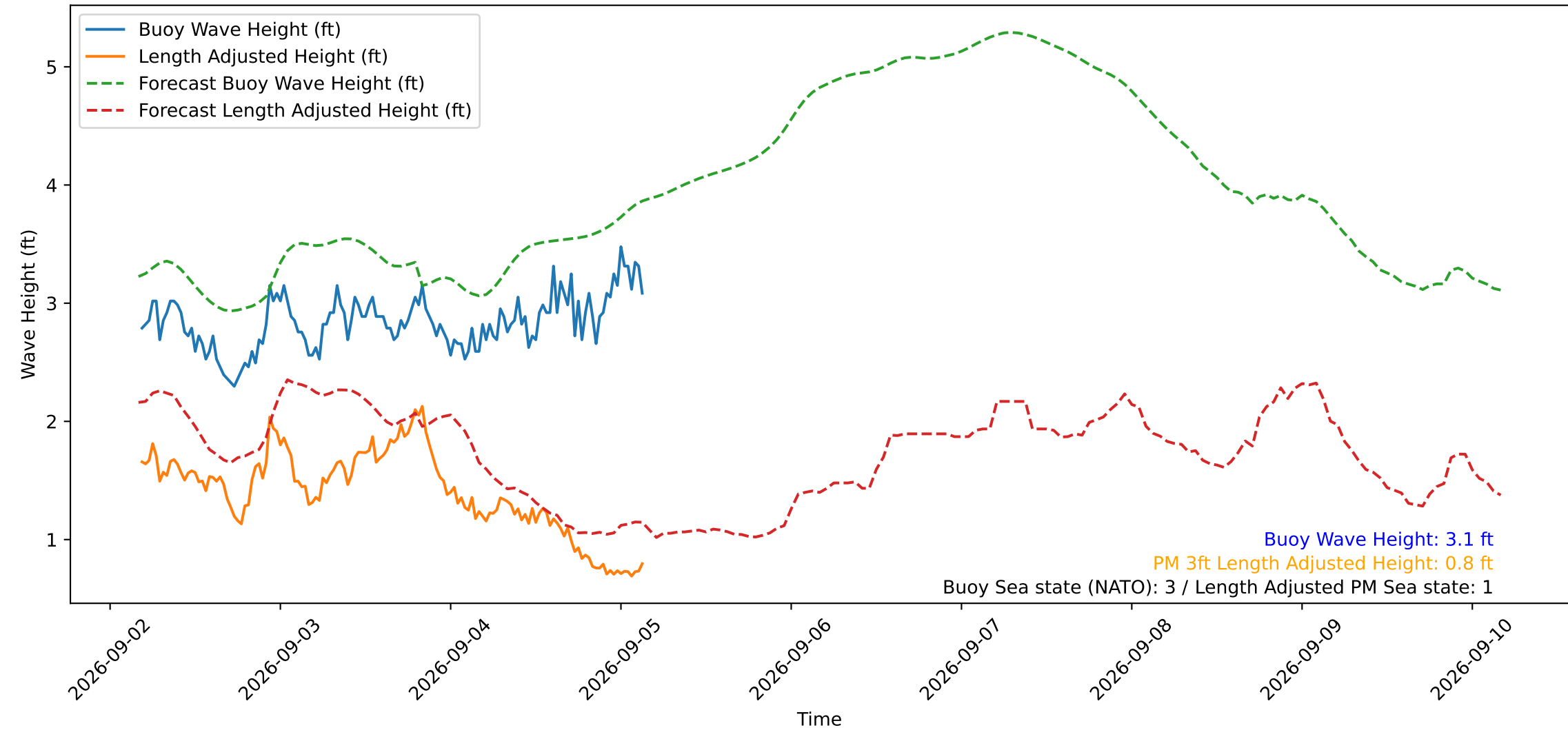
Wave Heights over Time for Red Beach at 2026-09-05 04:00:50
