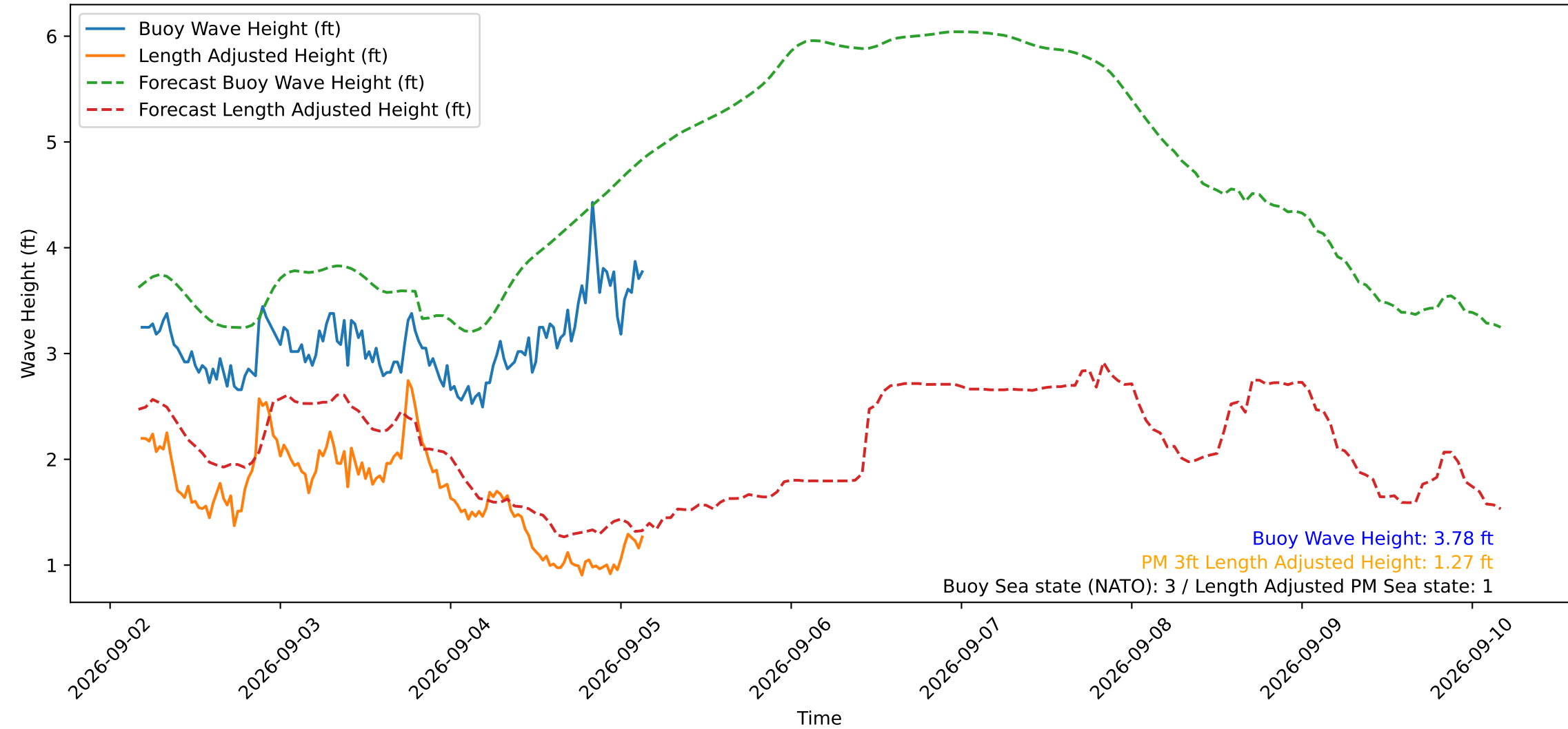
Wave Heights over Time for Green Beach at 2026-09-05 04:01:12
