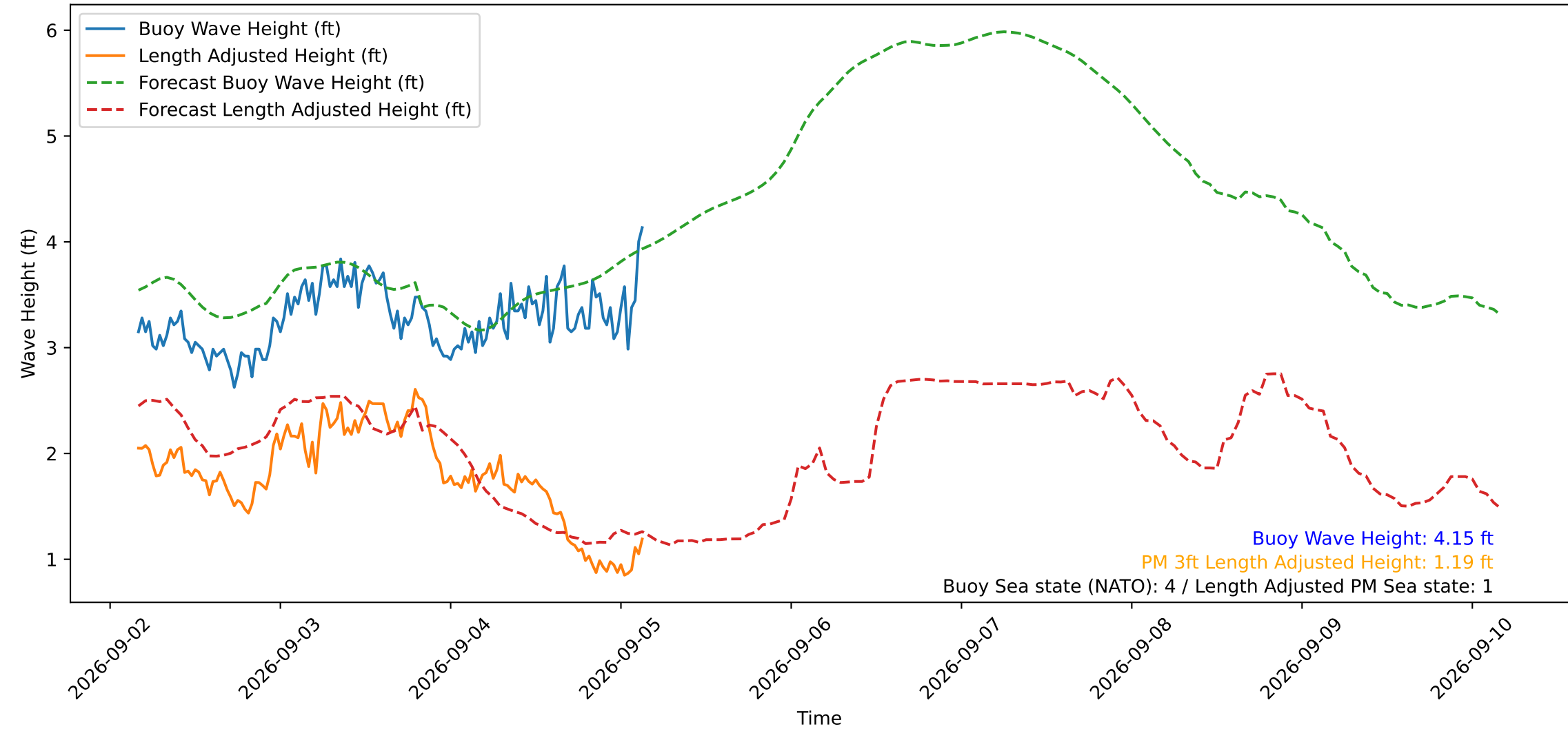
Wave Heights over Time for Oceanside Harbor at 2026-09-05 04:00:30
