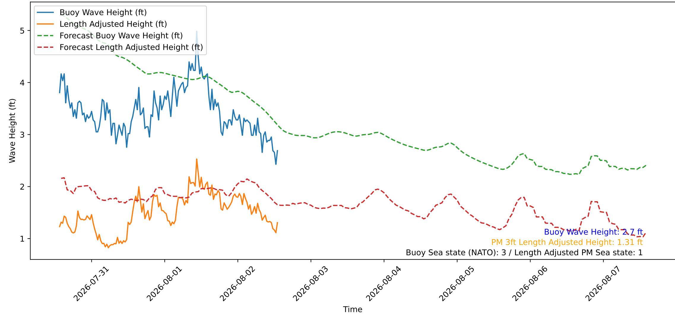
Wave Heights over Time for Green Beach at 2026-08-02 13:41:08
