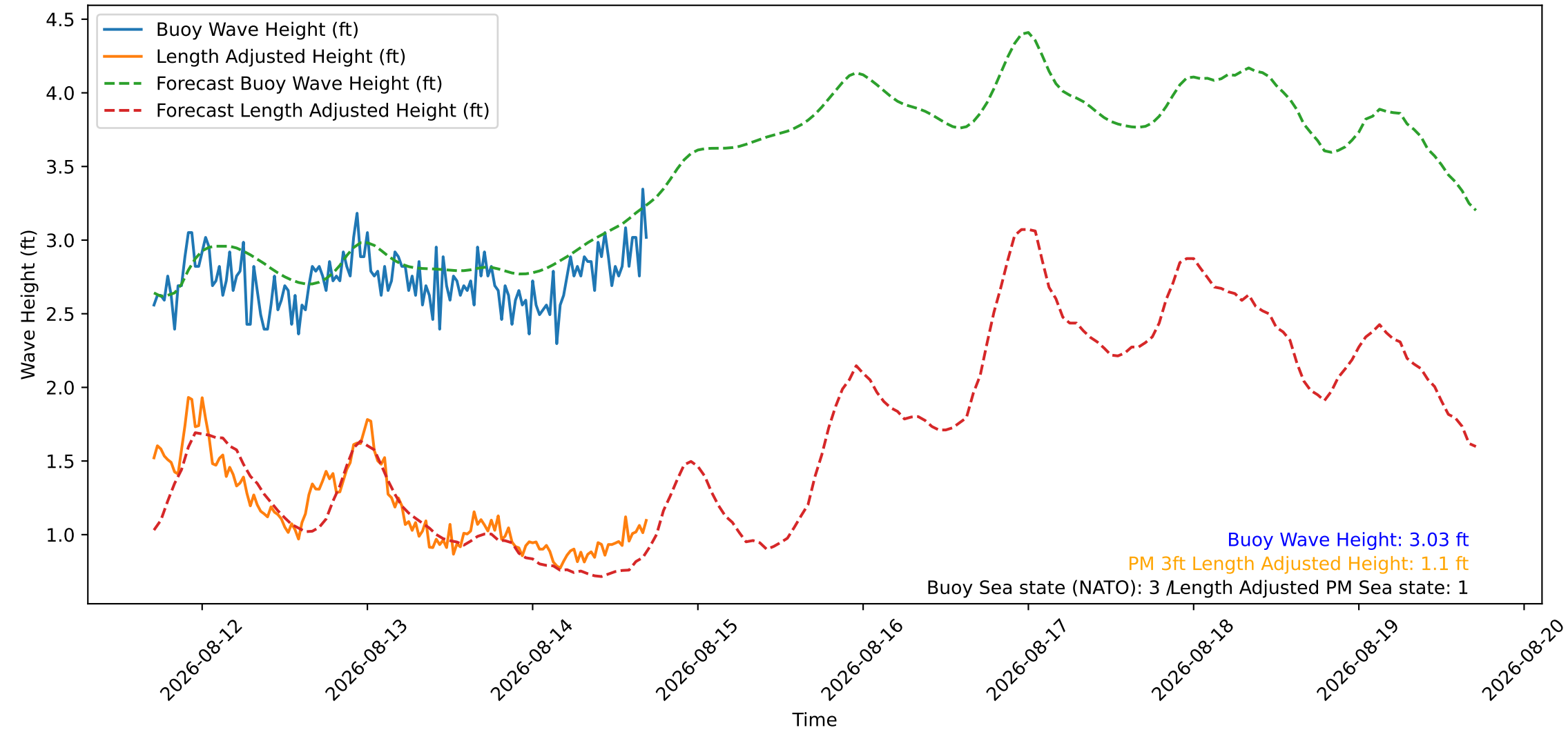
Wave Heights over Time for Oceanside Harbor at 2026-08-14 17:10:27
