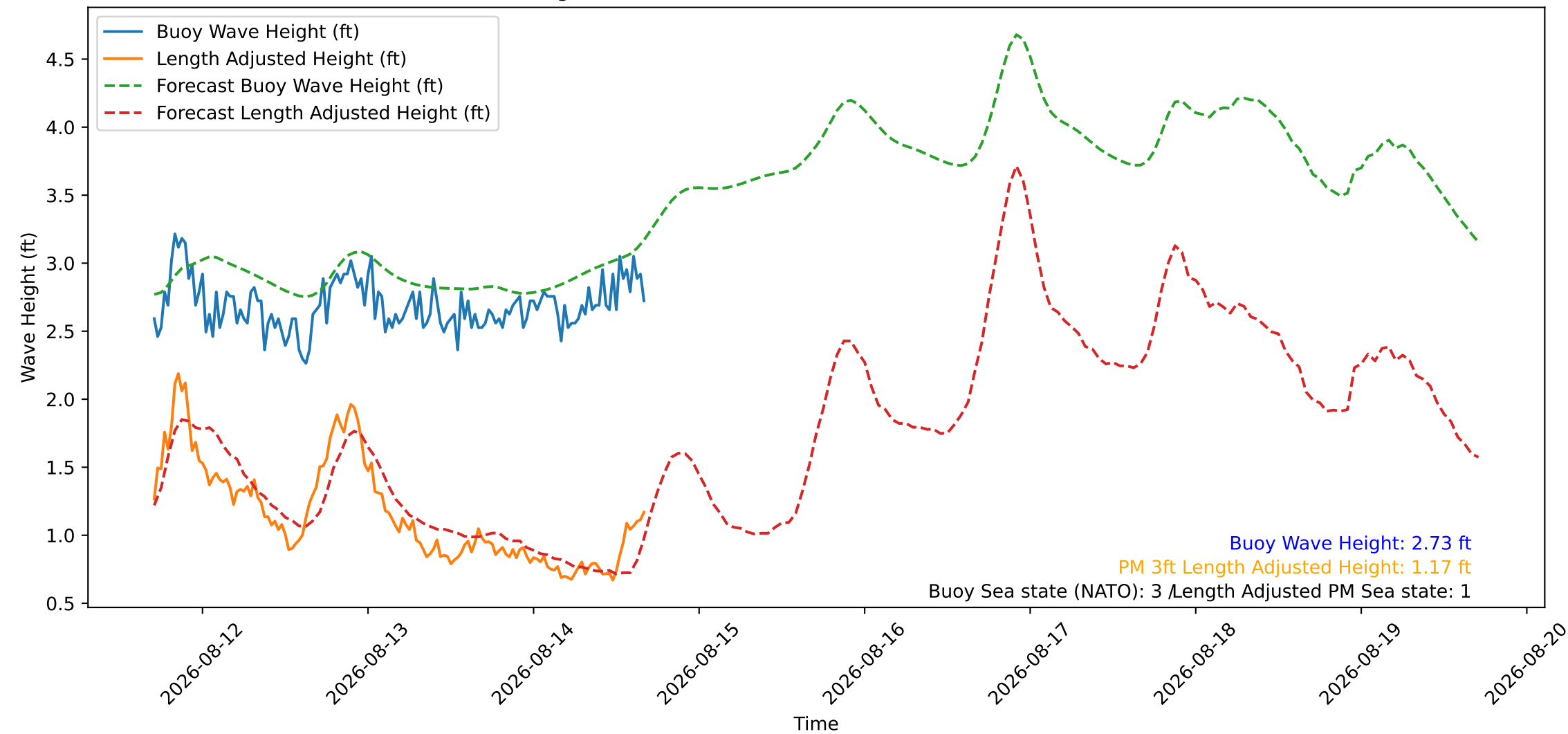
Wave Heights over Time for Green Beach at 2026-08-14 17:11:09
