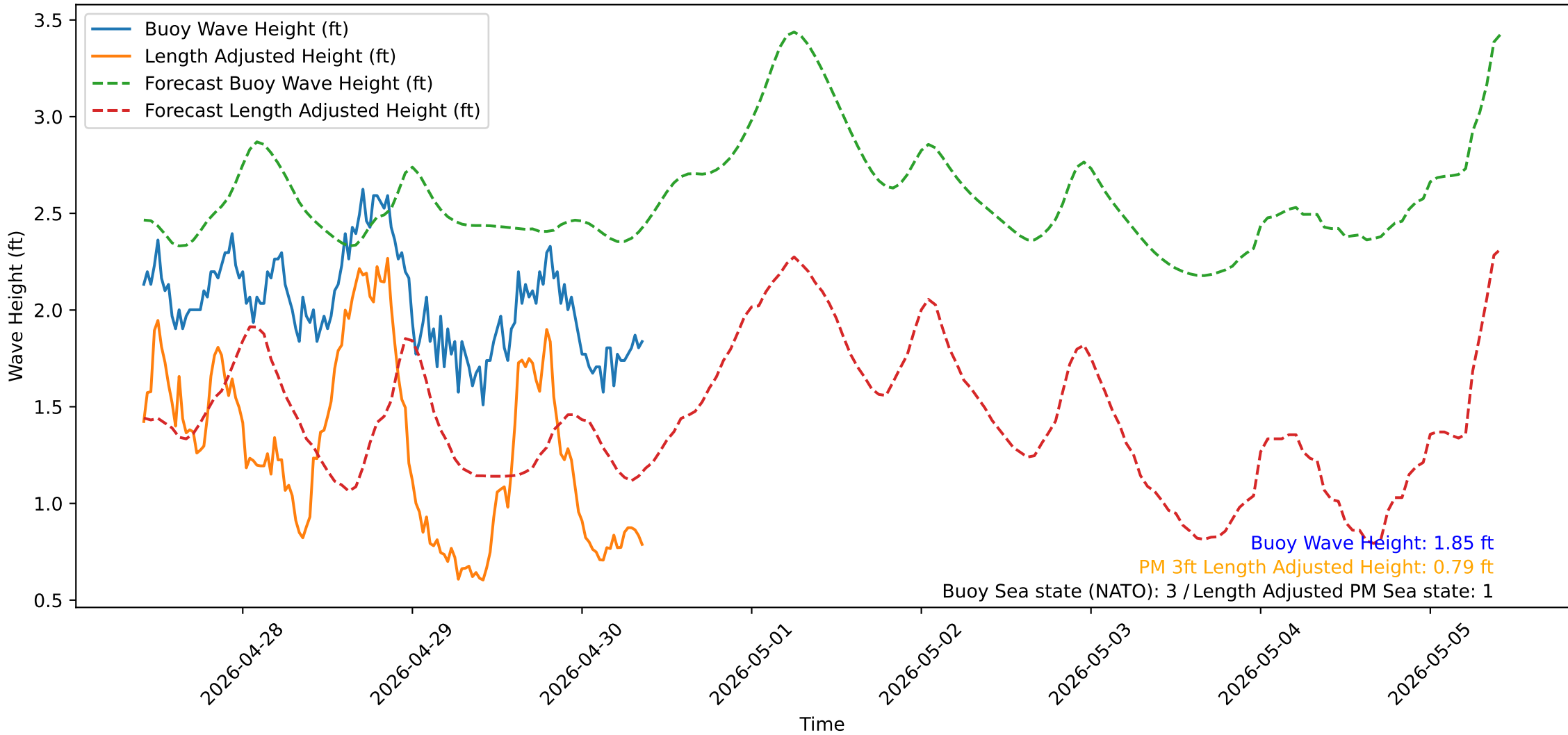
Wave Heights over Time for Red Beach at 2026-04-30 09:30:50
