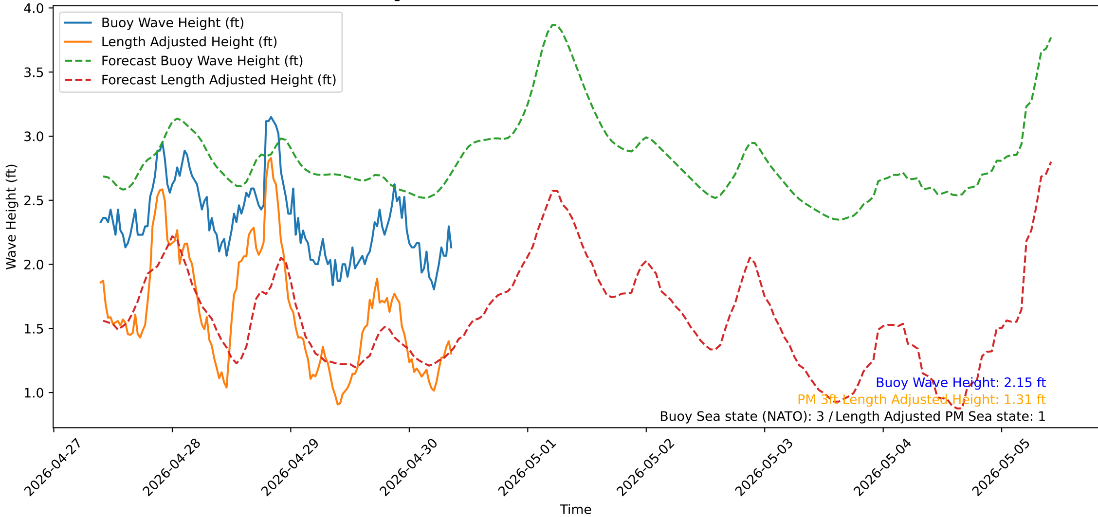
Wave Heights over Time for Green Beach at 2026-04-30 09:31:13
