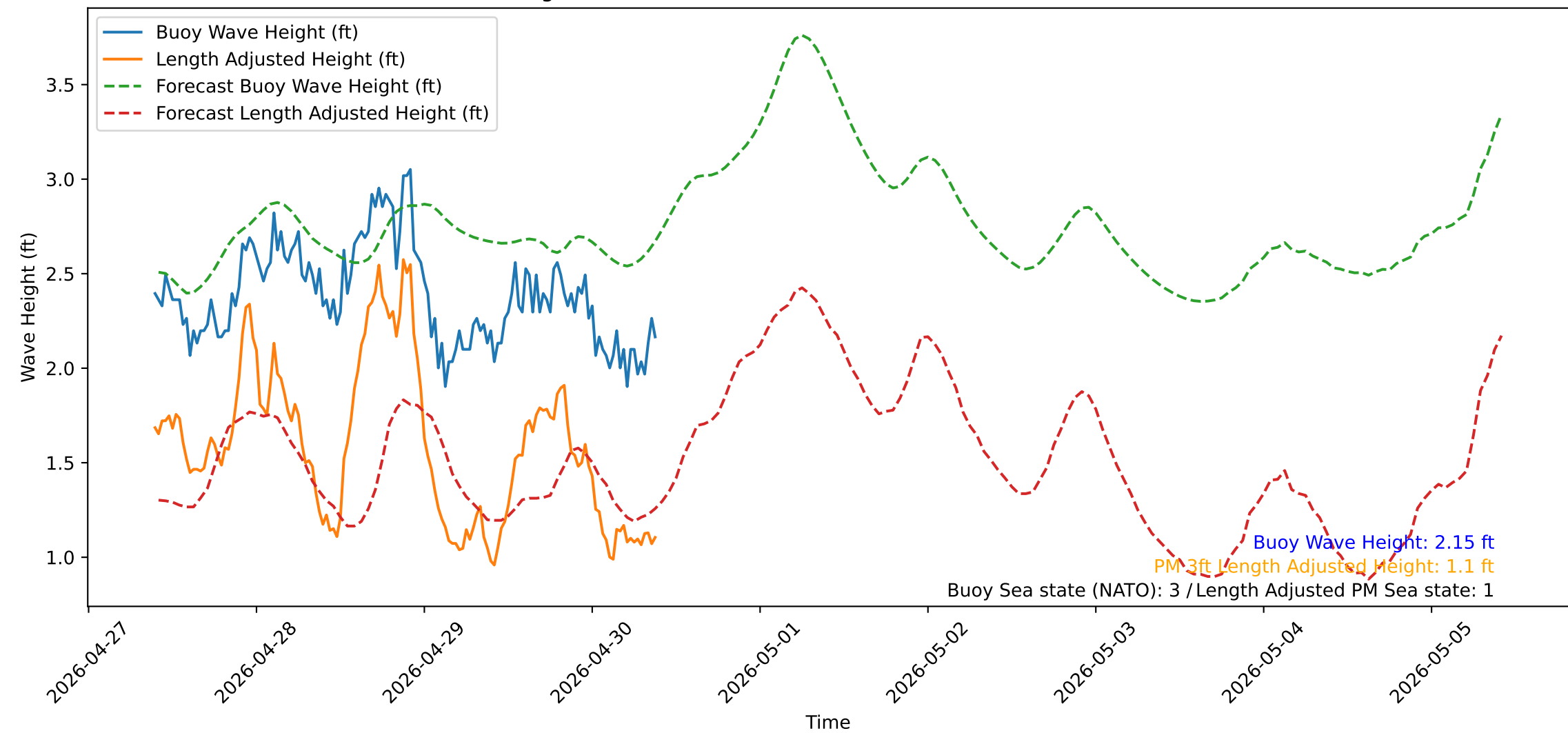
Wave Heights over Time for Oceanside Harbor at 2026-04-30 09:30:31
