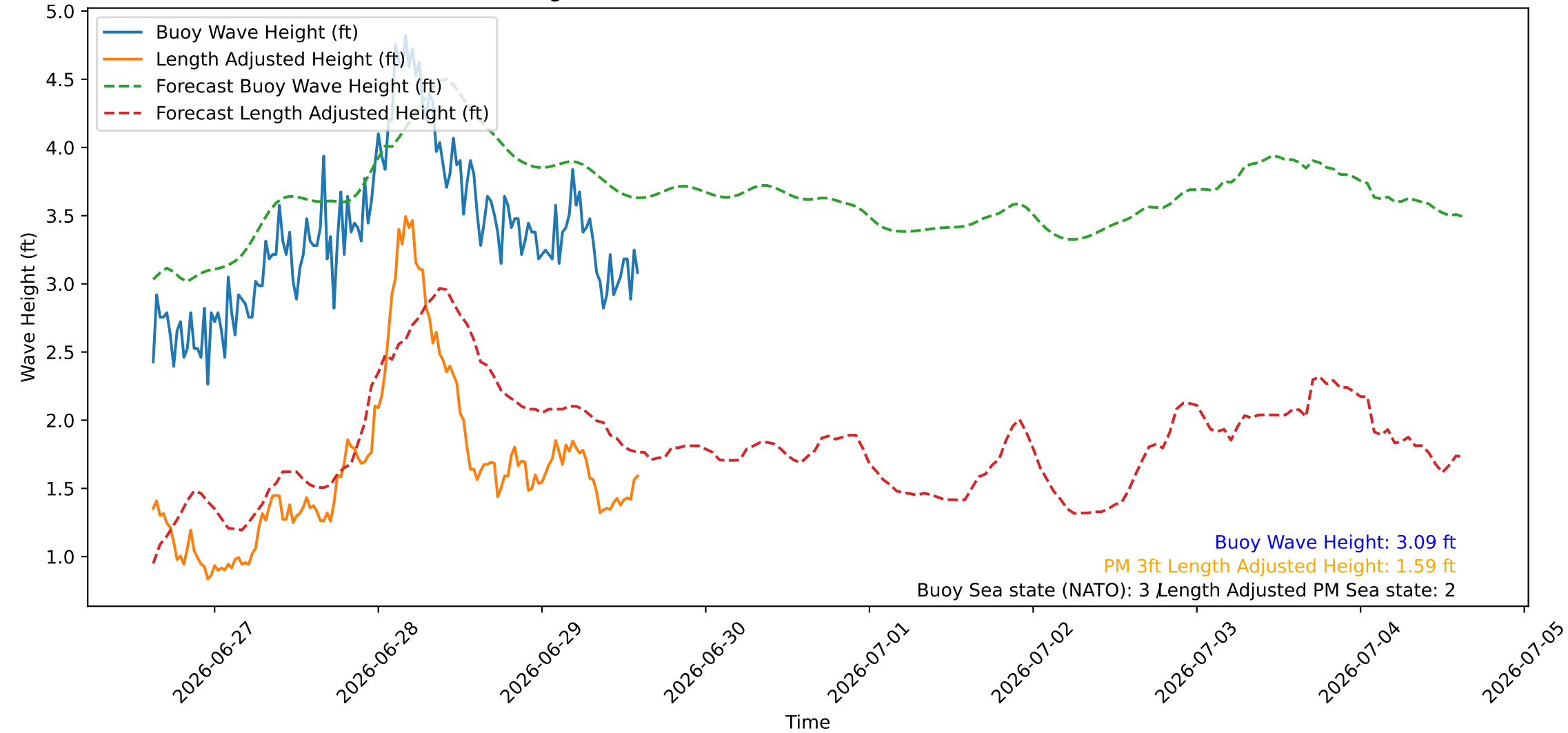
Wave Heights over Time for Green Beach at 2026-06-29 15:01:07
