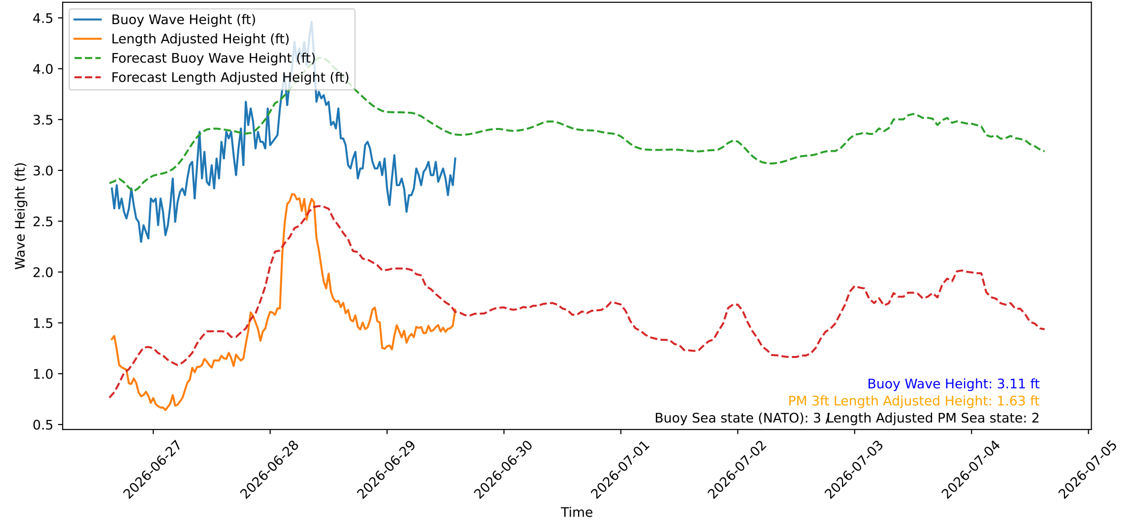
Wave Heights over Time for Red Beach at 2026-06-29 15:00:45
