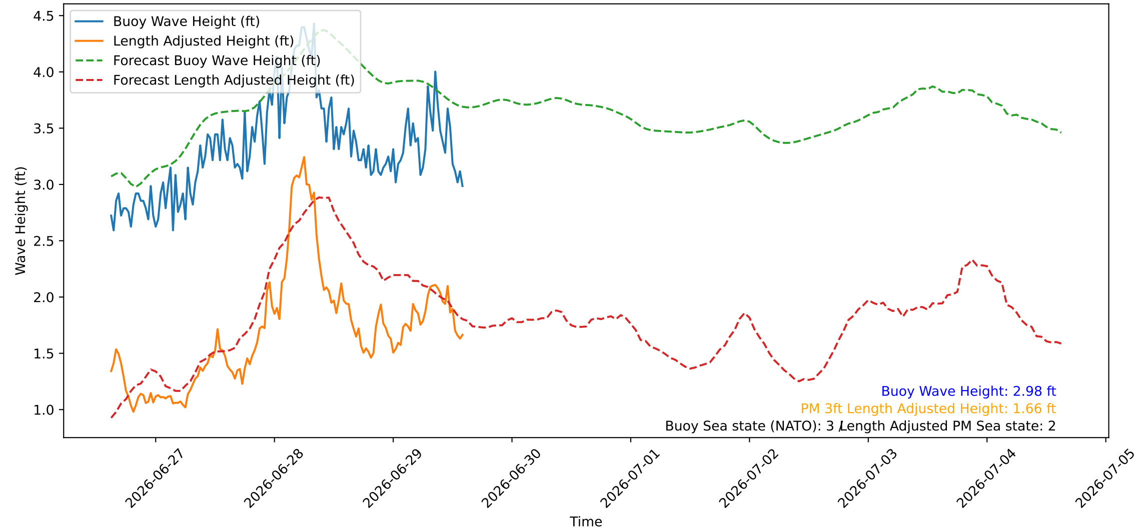
Wave Heights over Time for Oceanside Harbor at 2026-06-29 15:00:26
