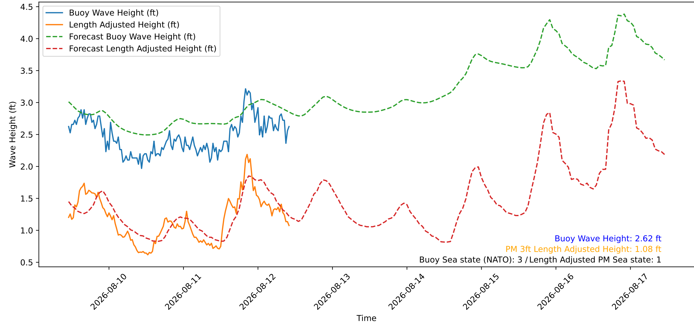
Wave Heights over Time for Green Beach at 2026-08-12 10:51:09
