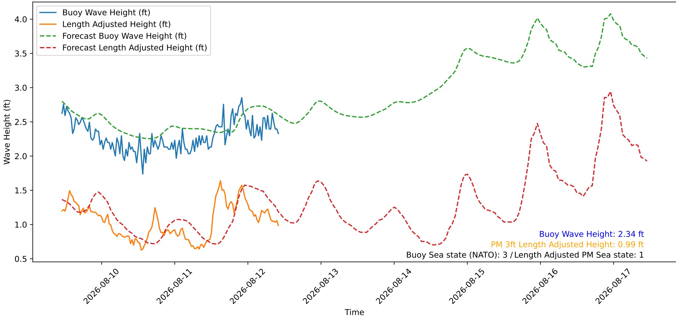
Wave Heights over Time for Red Beach at 2026-08-12 10:50:47
