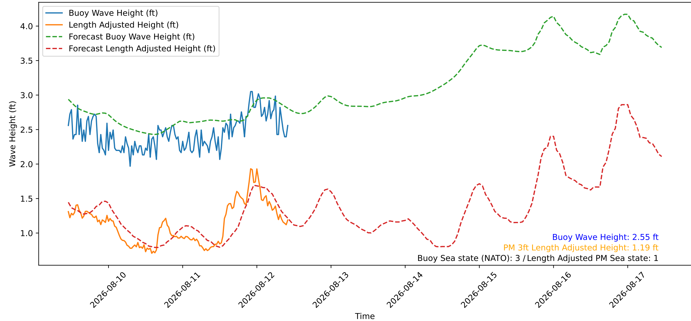
Wave Heights over Time for Oceanside Harbor at 2026-08-12 10:50:27
