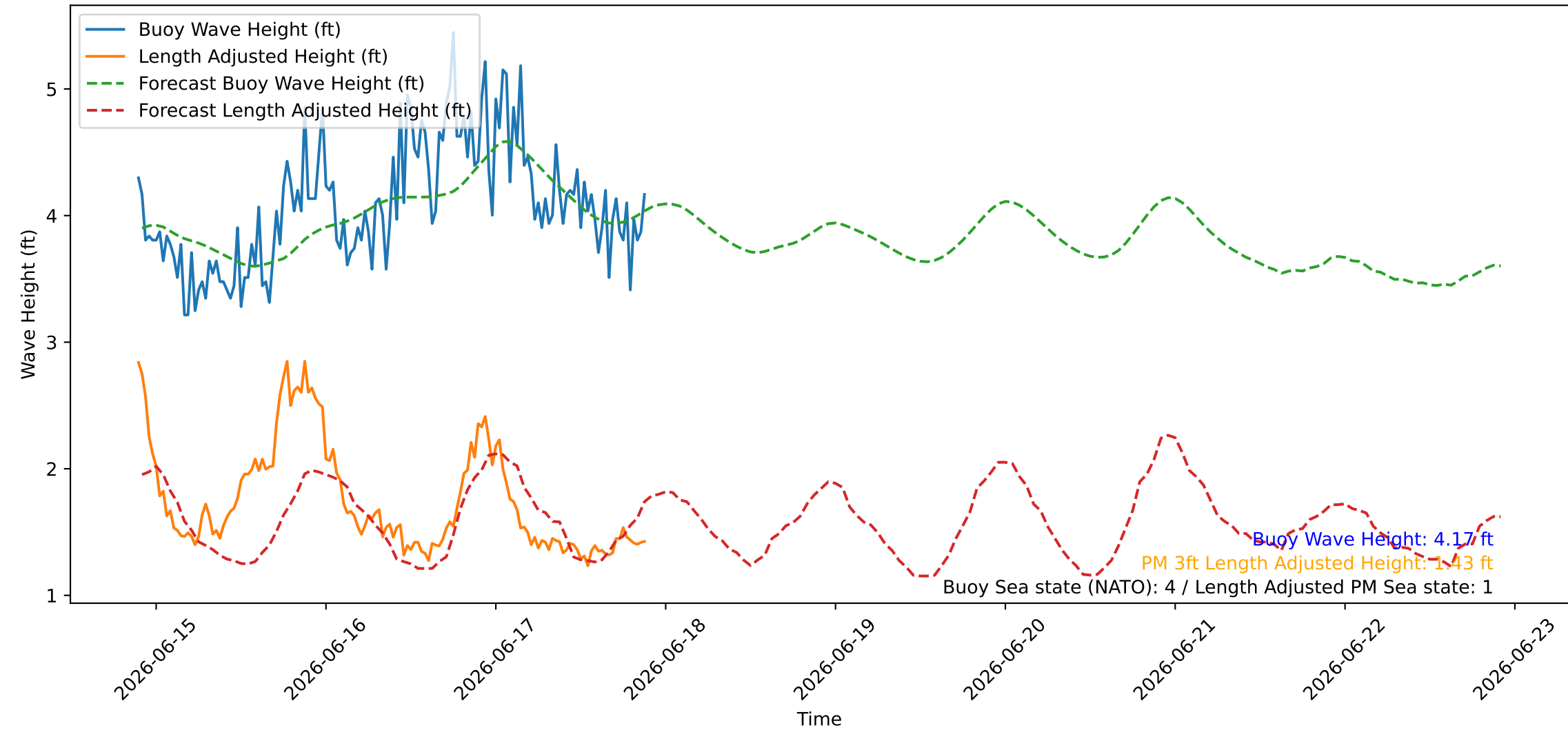
Wave Heights over Time for Oceanside Harbor at 2026-06-17 21:30:26
