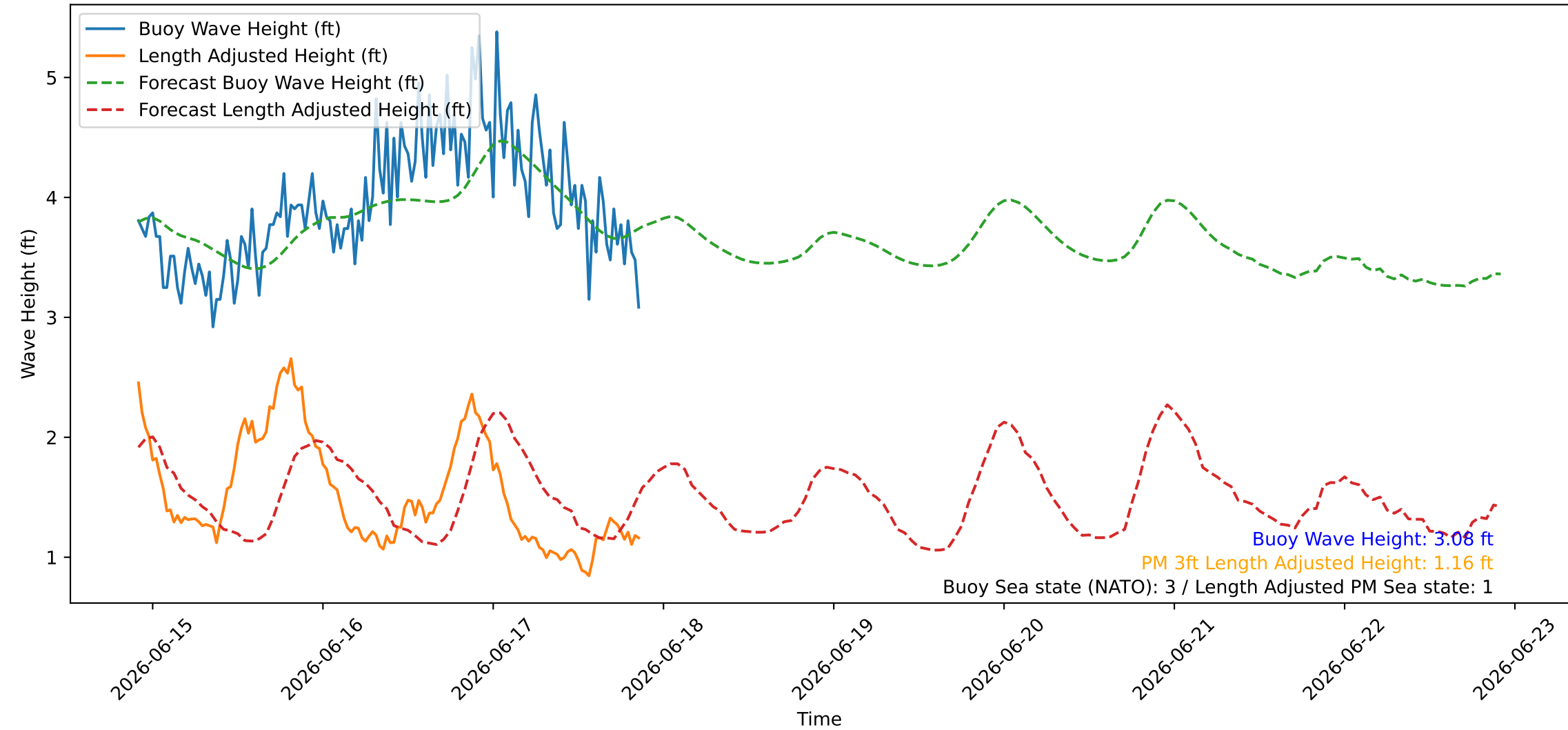
Wave Heights over Time for Red Beach at 2026-06-17 21:30:46
