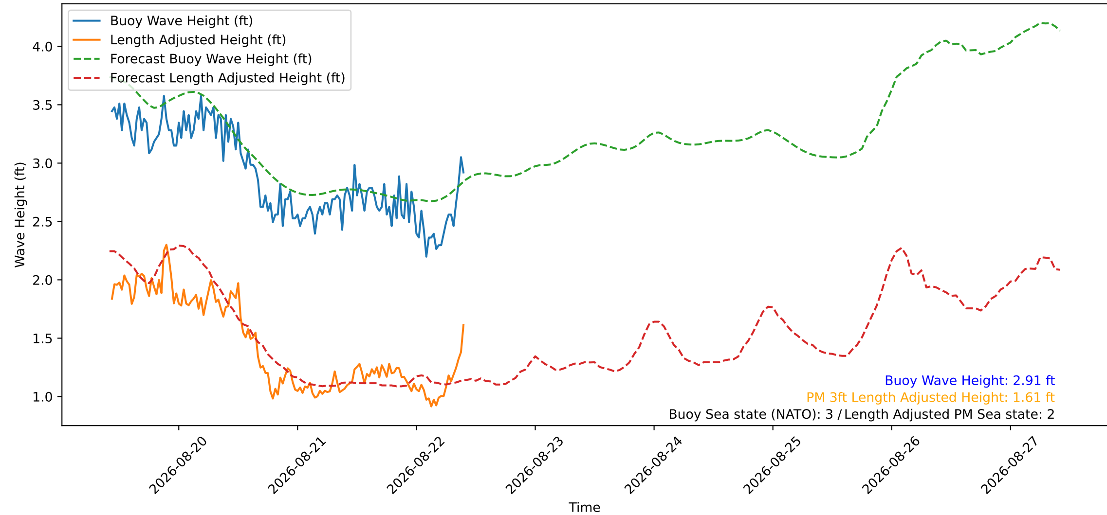
Wave Heights over Time for Oceanside Harbor at 2026-08-22 10:20:29
