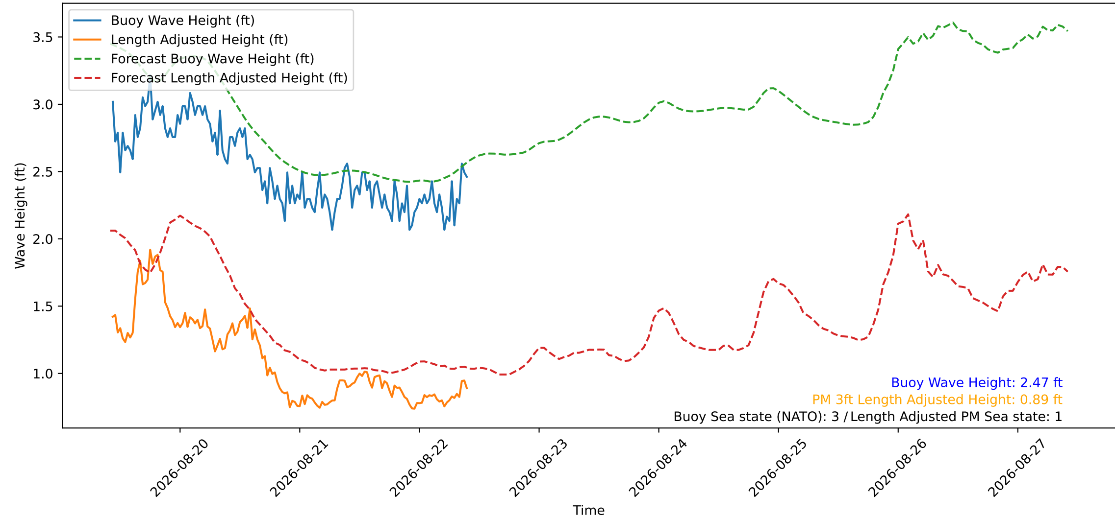
Wave Heights over Time for Red Beach at 2026-08-22 10:20:50
