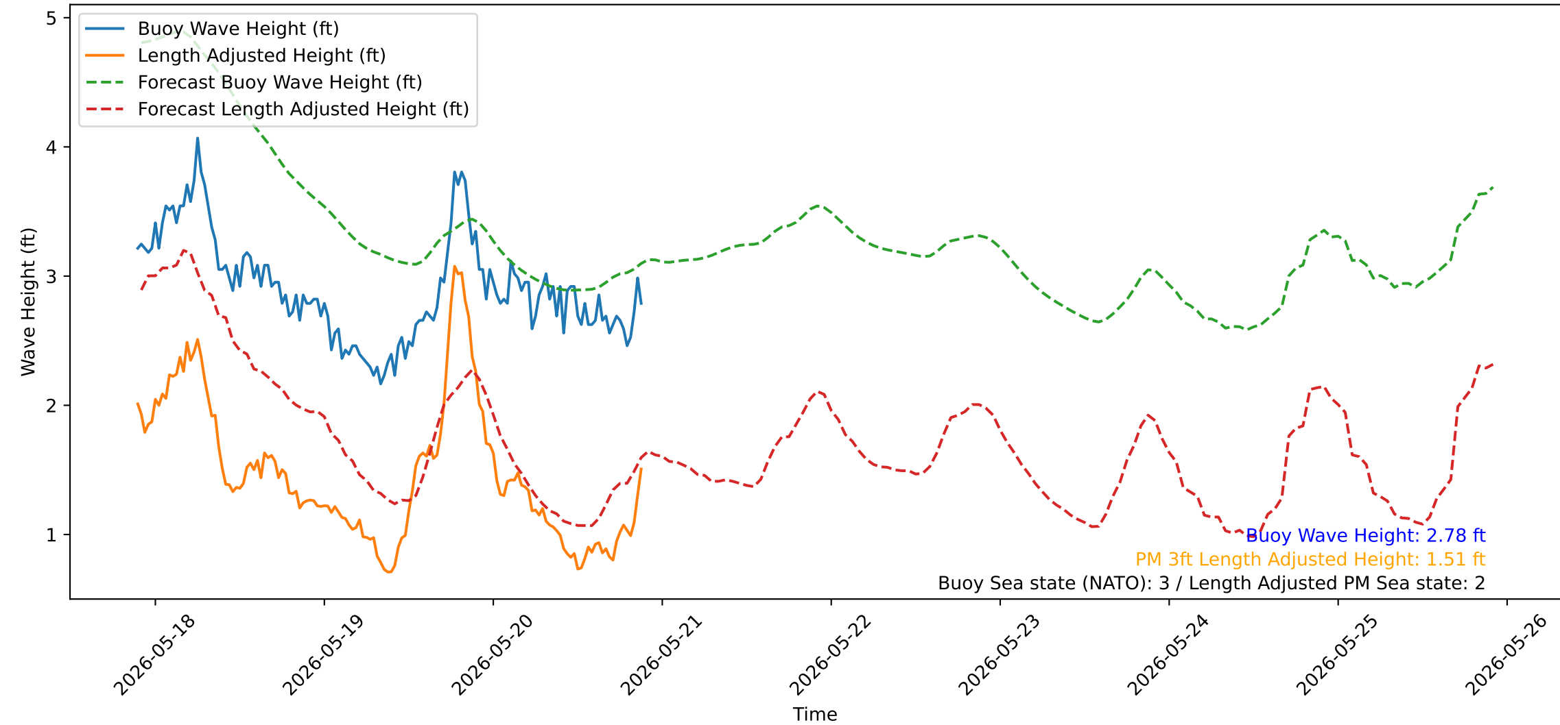
Wave Heights over Time for Green Beach at 2026-05-20 21:41:13
