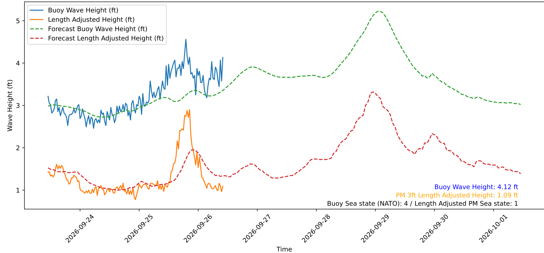
Wave Heights over Time for Green Beach at 2026-09-26 10:51:15
