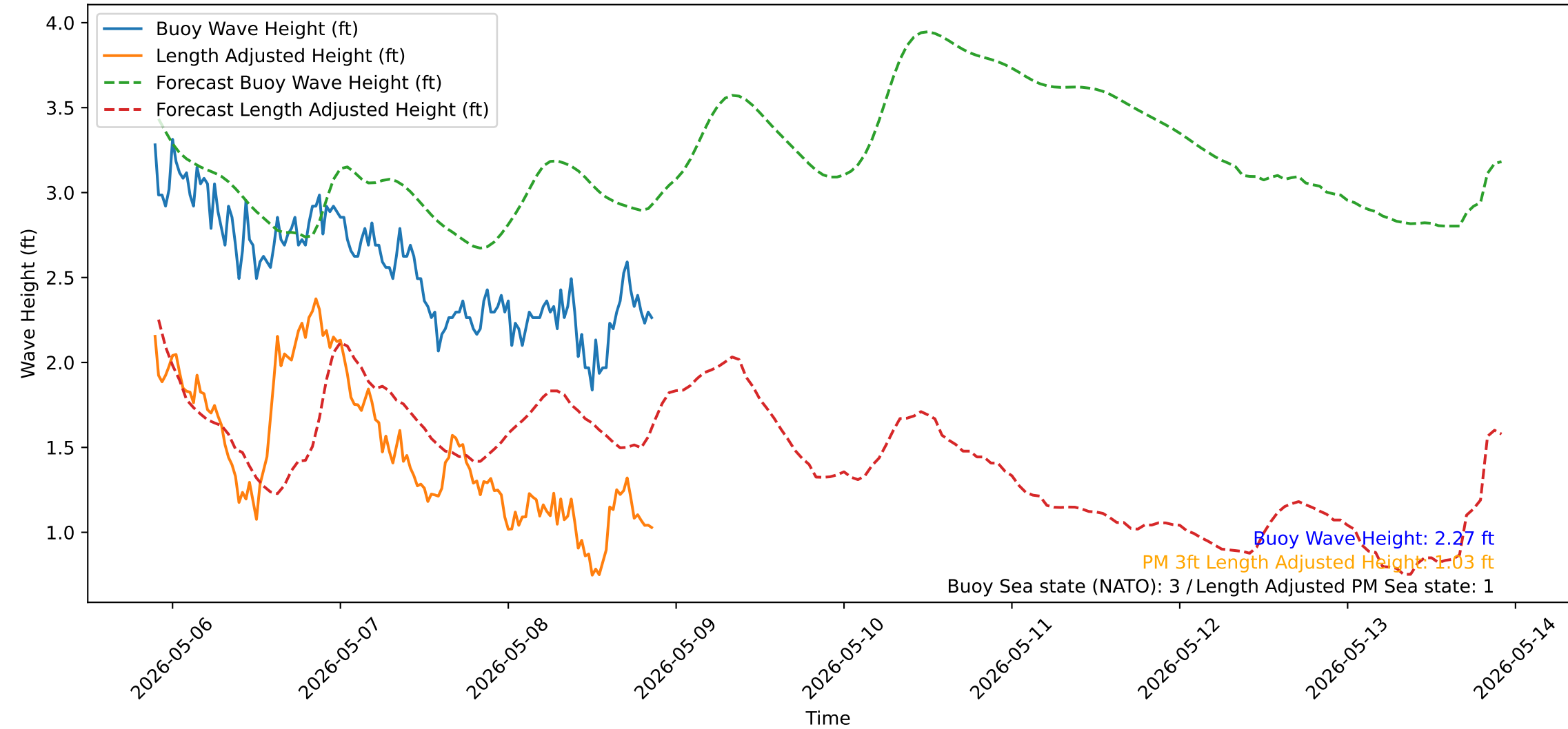
Wave Heights over Time for Green Beach at 2026-05-08 21:31:14
