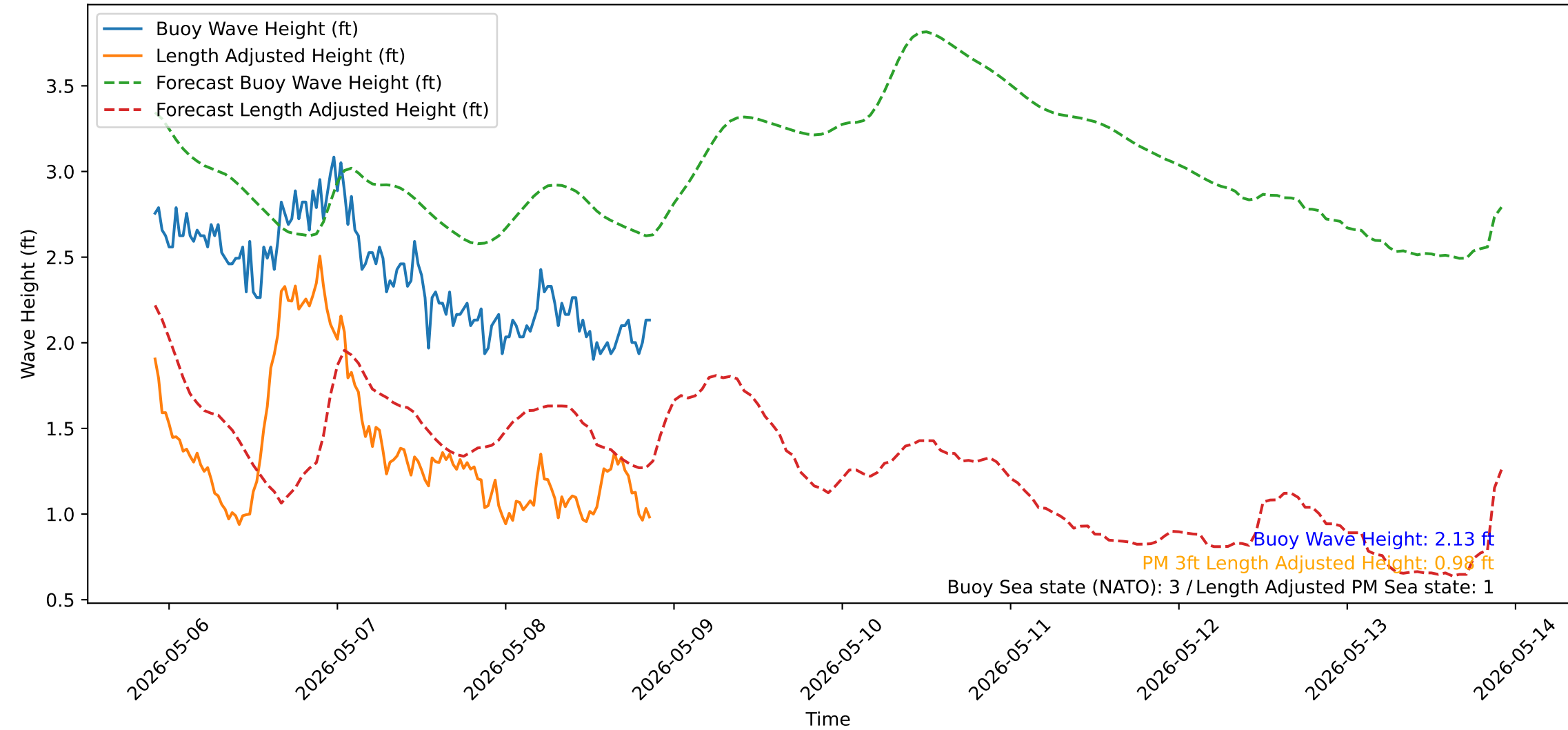
Wave Heights over Time for Red Beach at 2026-05-08 21:30:51
