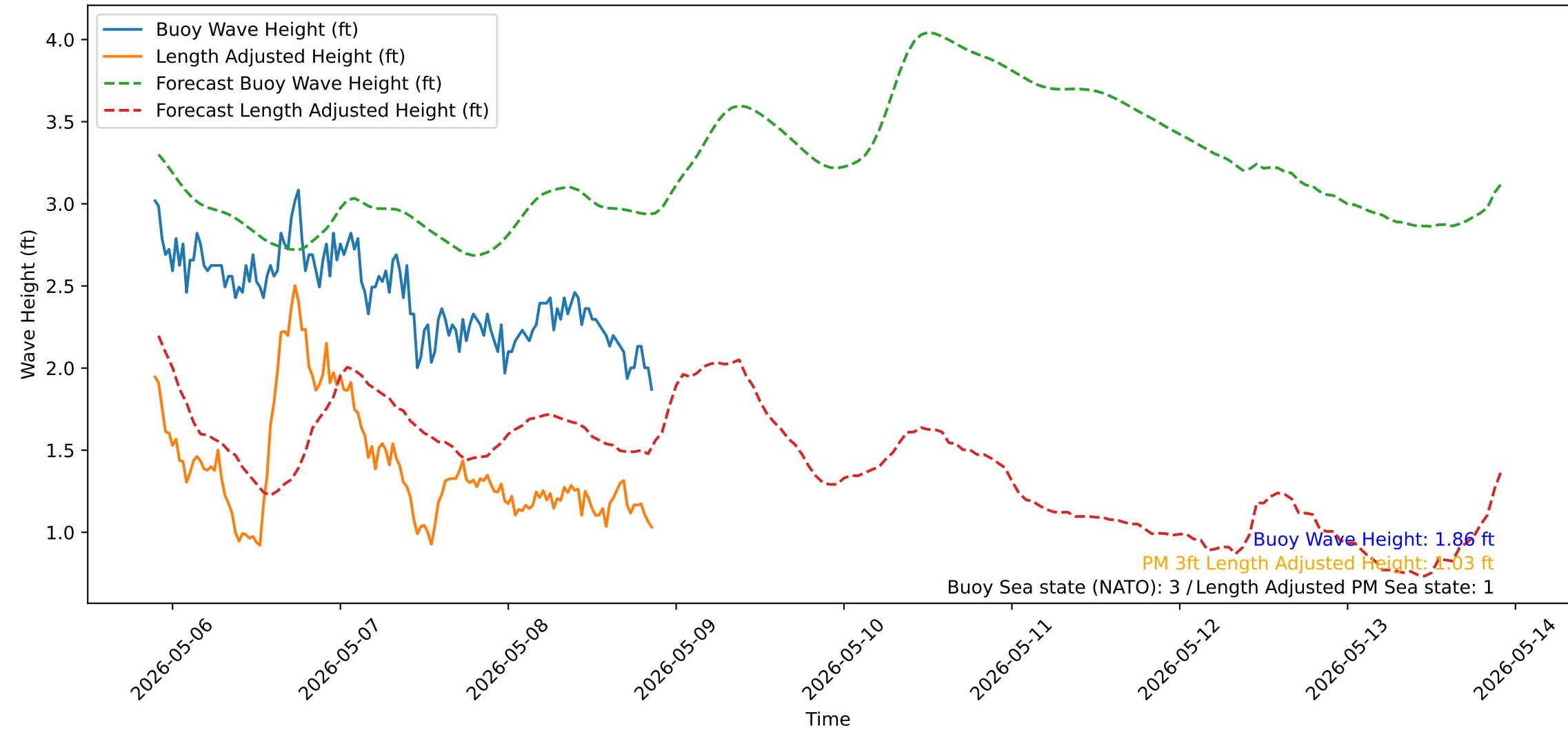
Wave Heights over Time for Oceanside Harbor at 2026-05-08 21:30:31
