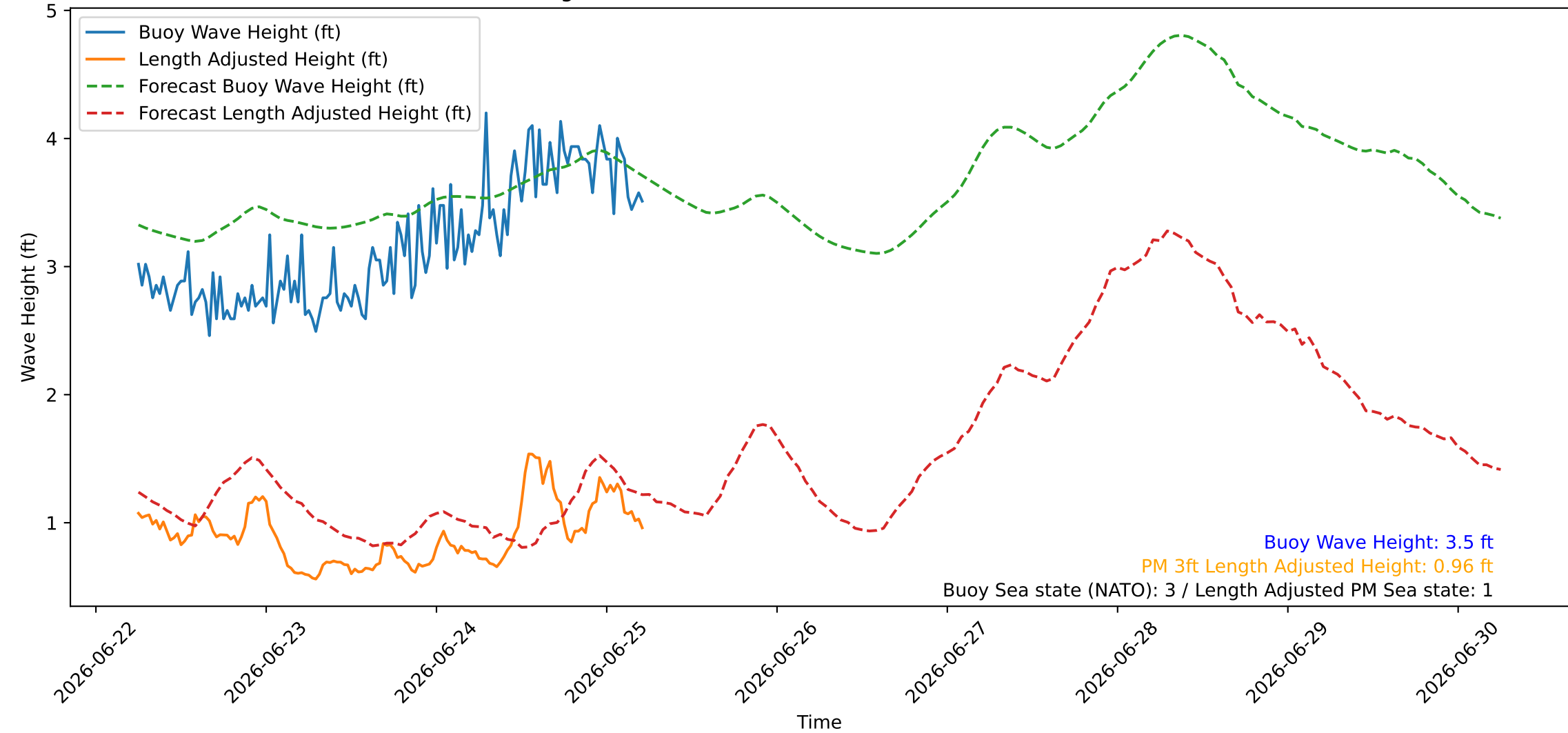
Wave Heights over Time for Green Beach at 2026-06-25 06:01:07
