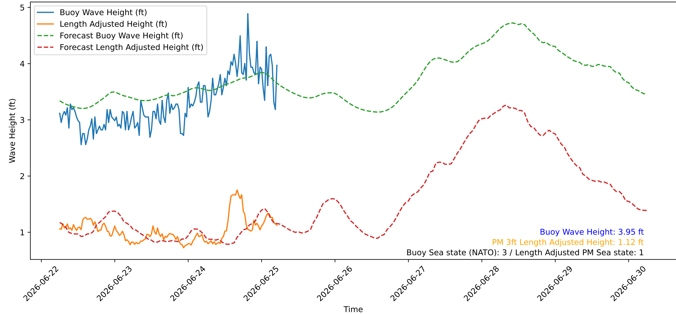
Wave Heights over Time for Oceanside Harbor at 2026-06-25 06:00:26
