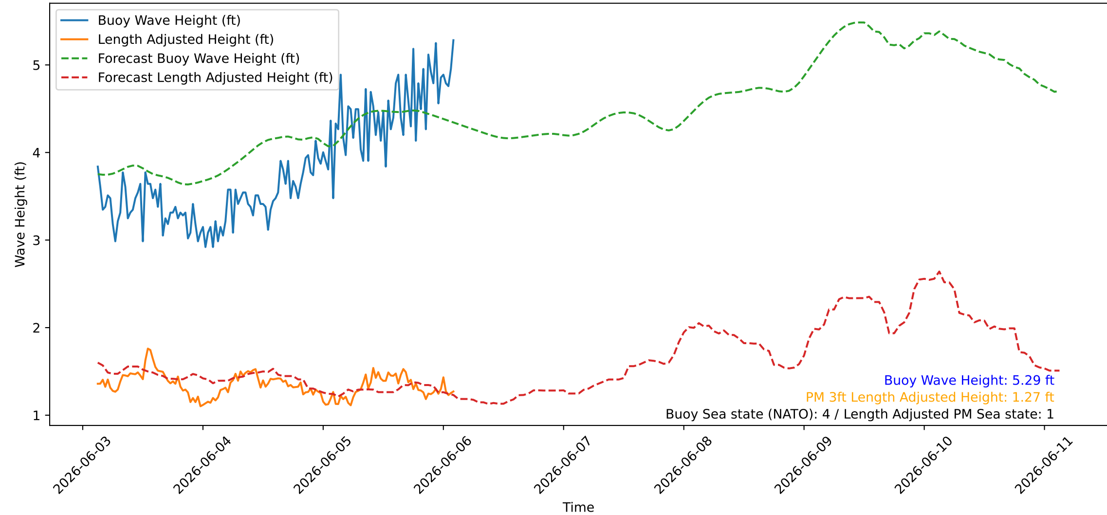
Wave Heights over Time for Oceanside Harbor at 2026-06-06 03:00:26
