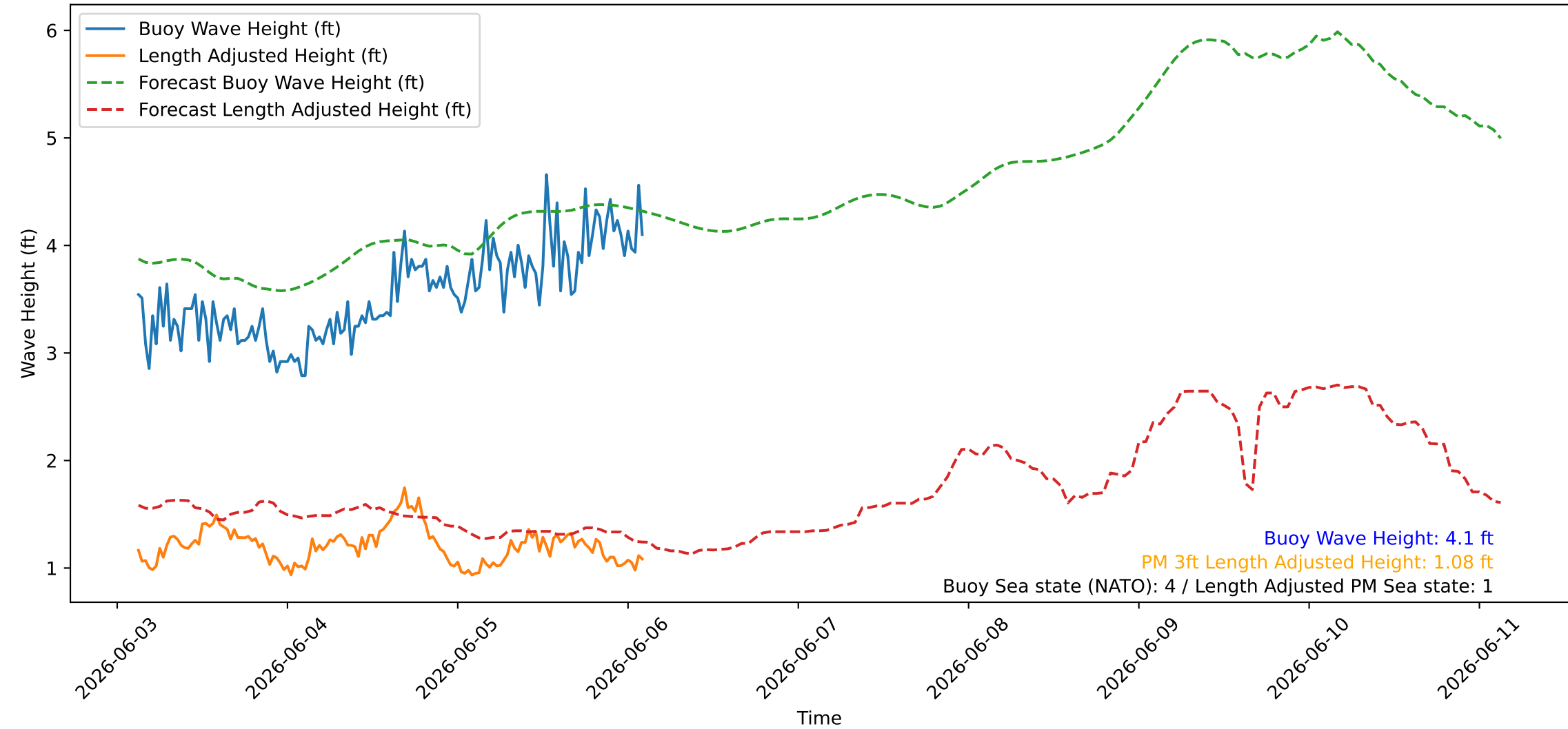
Wave Heights over Time for Green Beach at 2026-06-06 03:01:08
