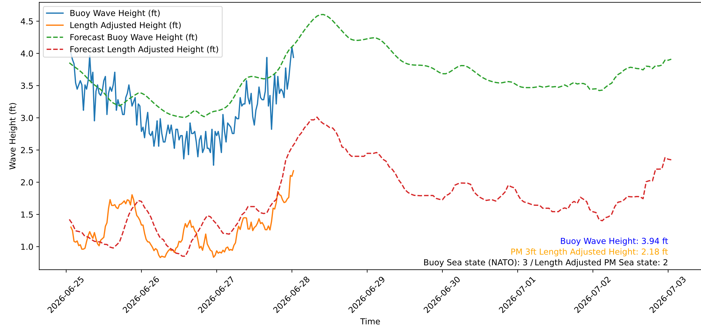
Wave Heights over Time for Green Beach at 2026-06-28 01:21:09
