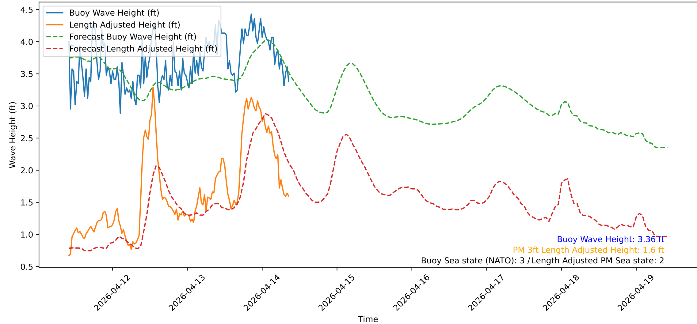
Wave Heights over Time for Red Beach at 2026-04-14 09:30:50
