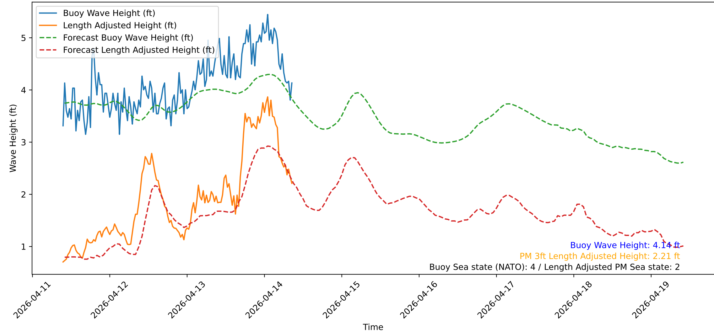
Wave Heights over Time for Oceanside Harbor at 2026-04-14 09:30:31
