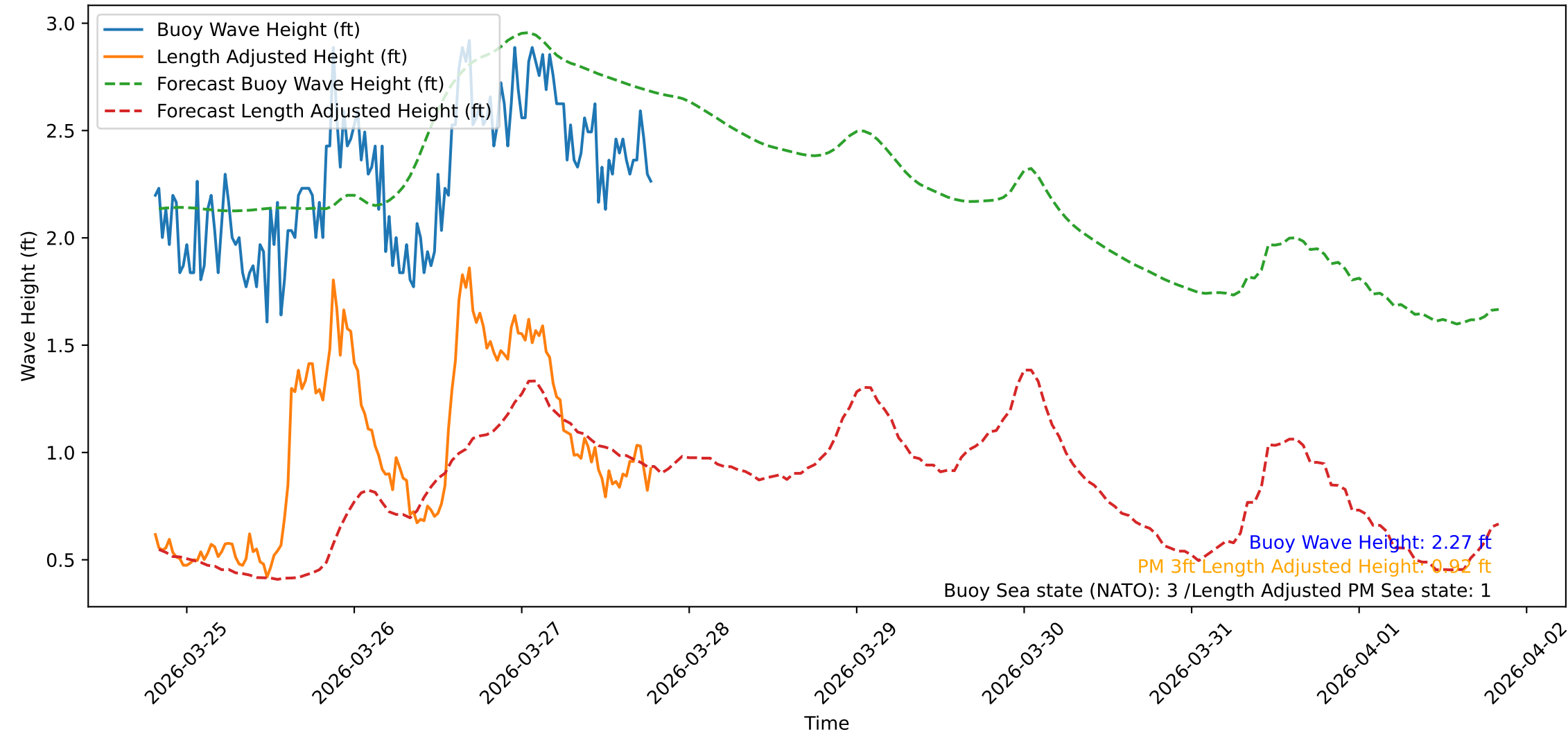
Wave Heights over Time for Oceanside Harbor at 2026-03-27 19:30:31
