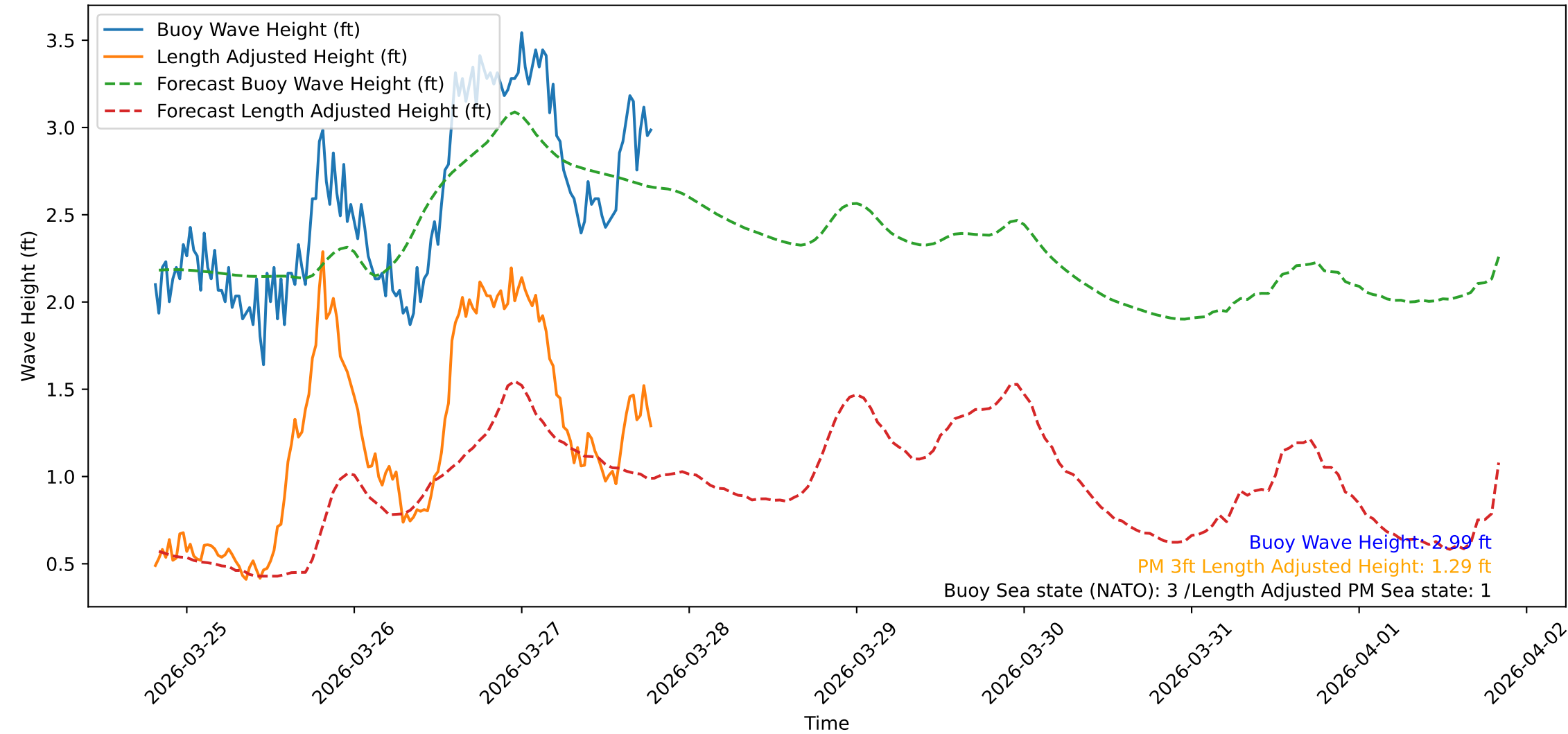
Wave Heights over Time for Green Beach at 2026-03-27 19:31:09
