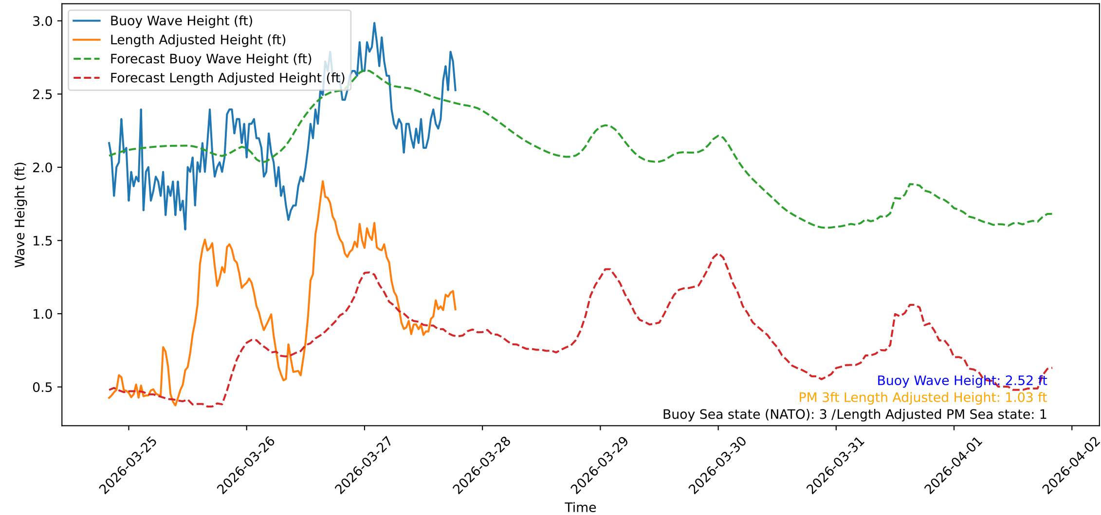
Wave Heights over Time for Red Beach at 2026-03-27 19:30:47
