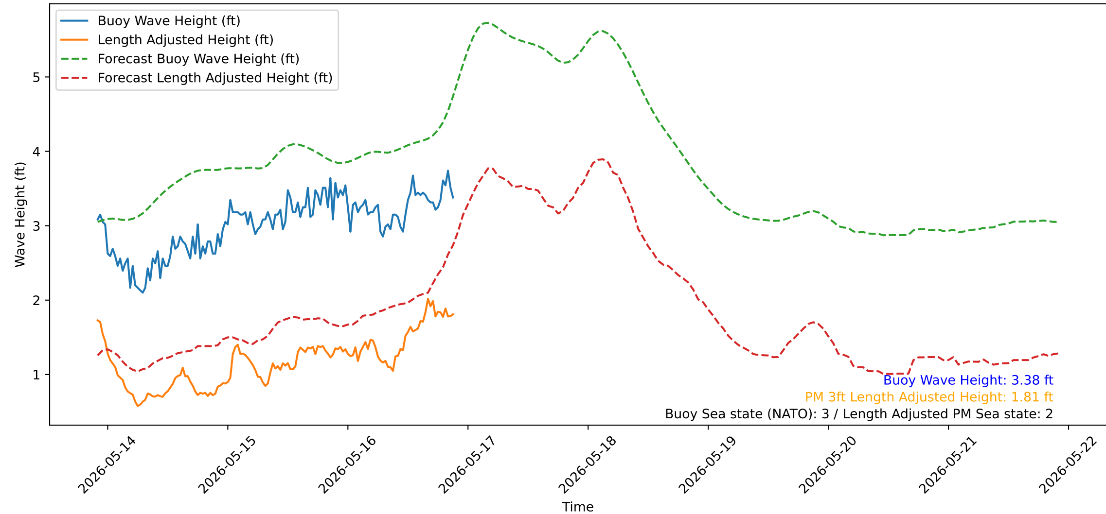
Wave Heights over Time for Green Beach at 2026-05-16 21:51:15
