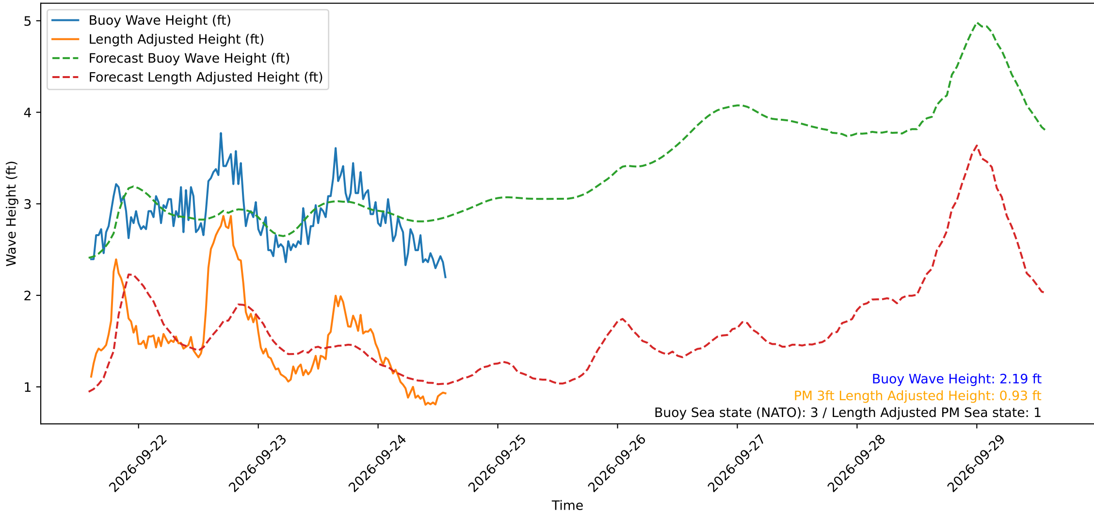
Wave Heights over Time for Oceanside Harbor at 2026-09-24 14:20:30
