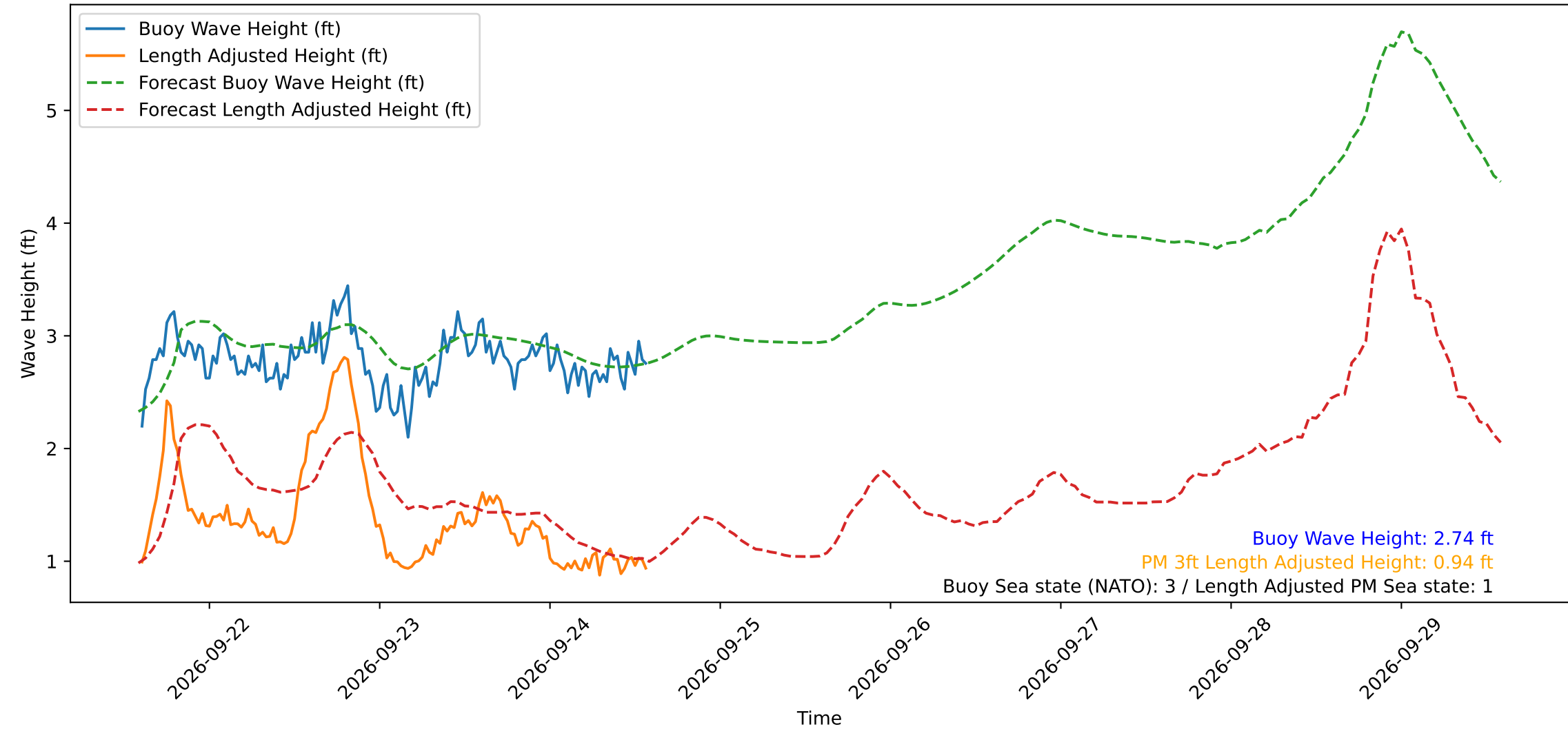
Wave Heights over Time for Green Beach at 2026-09-24 14:21:17
