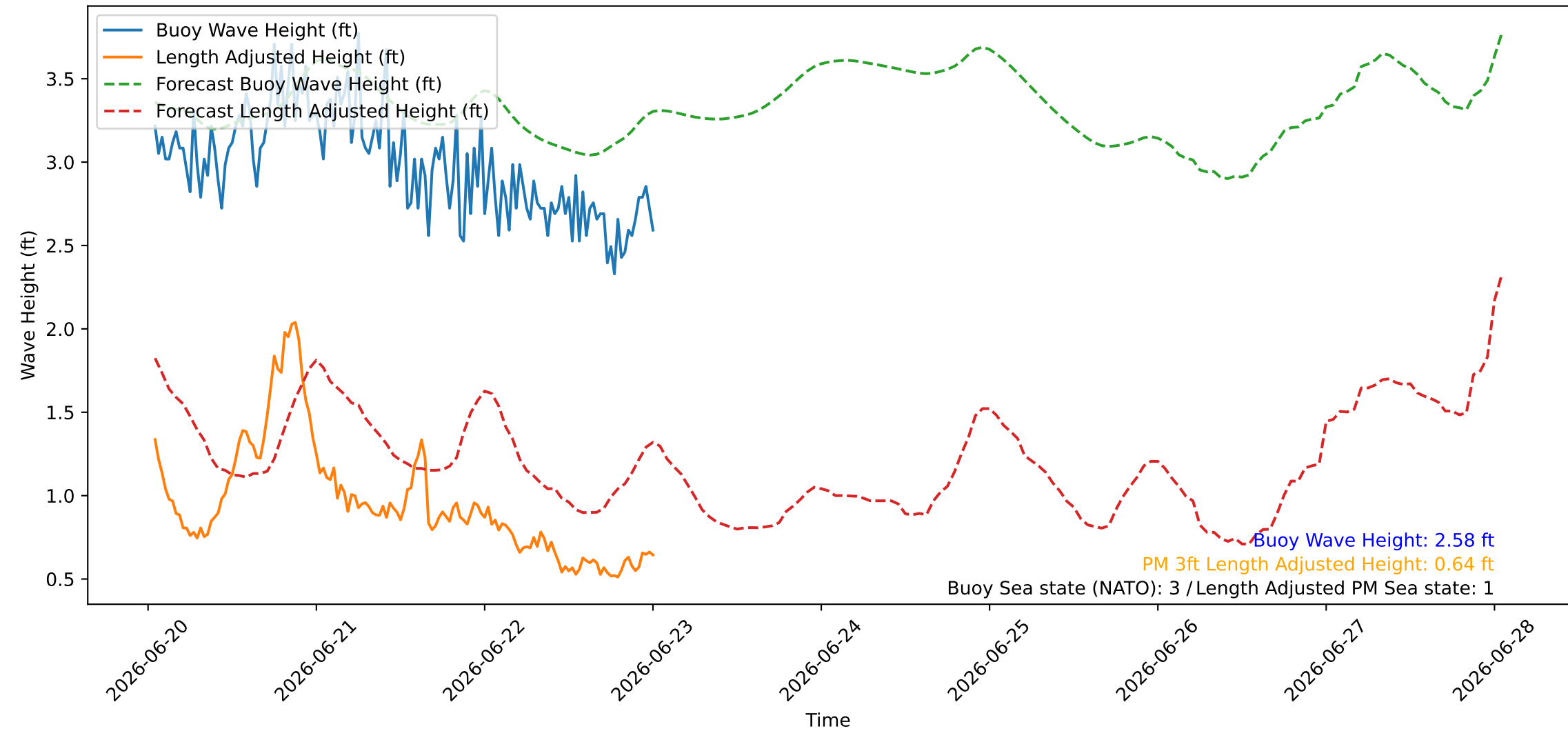
Wave Heights over Time for Red Beach at 2026-06-23 00:50:47
