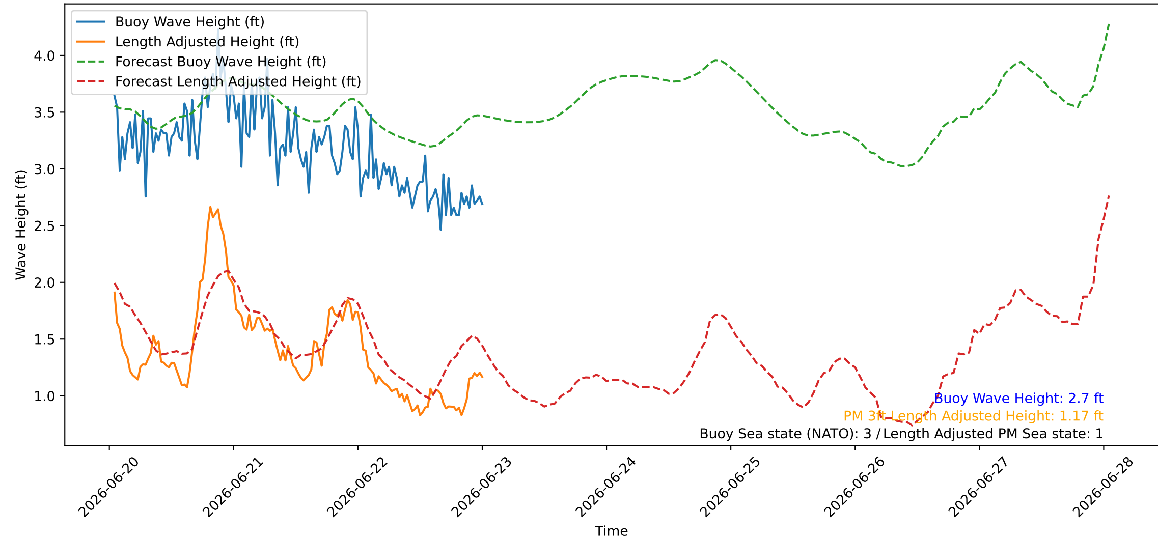
Wave Heights over Time for Green Beach at 2026-06-23 00:51:10
