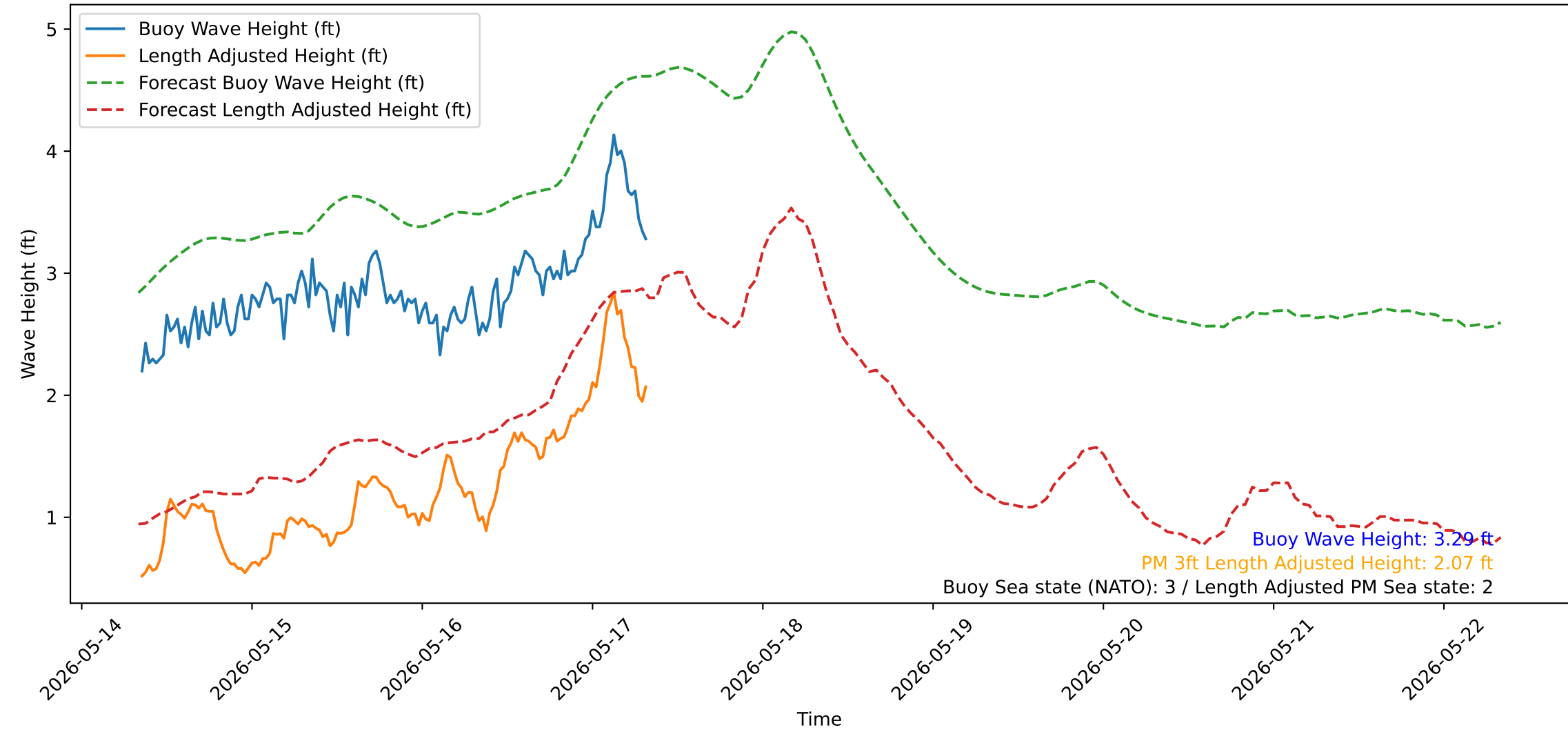
Wave Heights over Time for Red Beach at 2026-05-17 08:20:52
