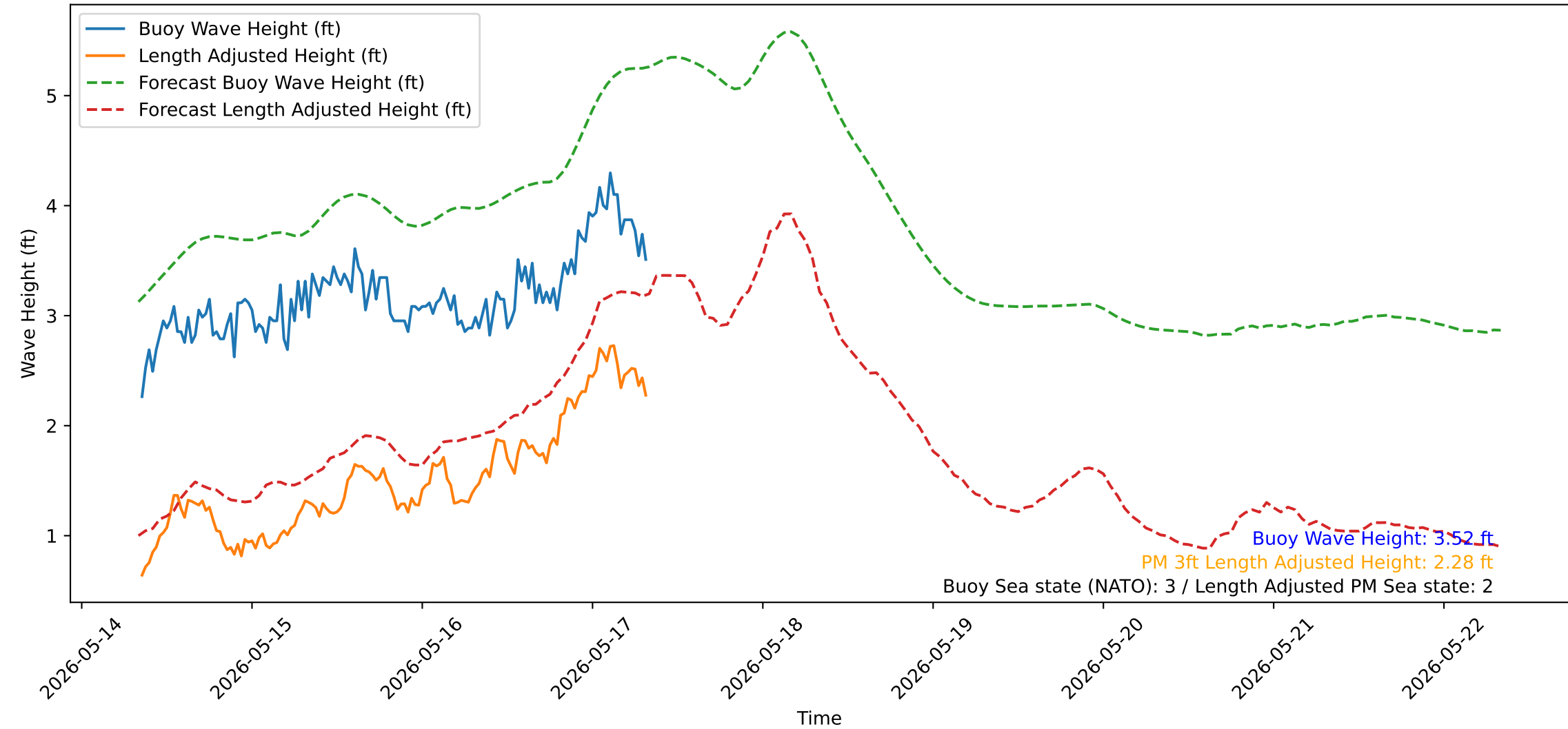
Wave Heights over Time for Oceanside Harbor at 2026-05-17 08:20:32
