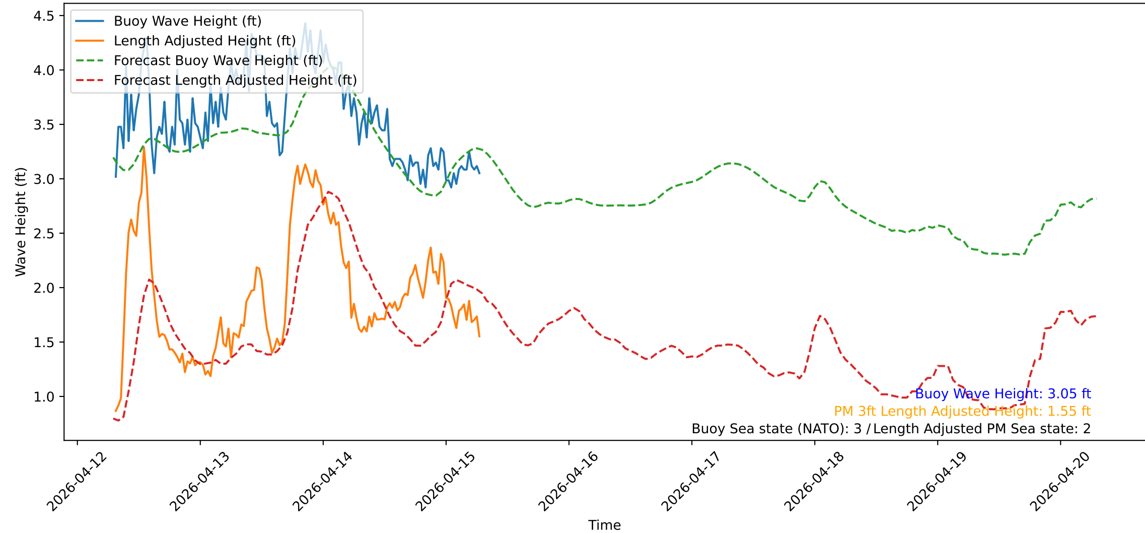
Wave Heights over Time for Red Beach at 2026-04-15 07:10:50
