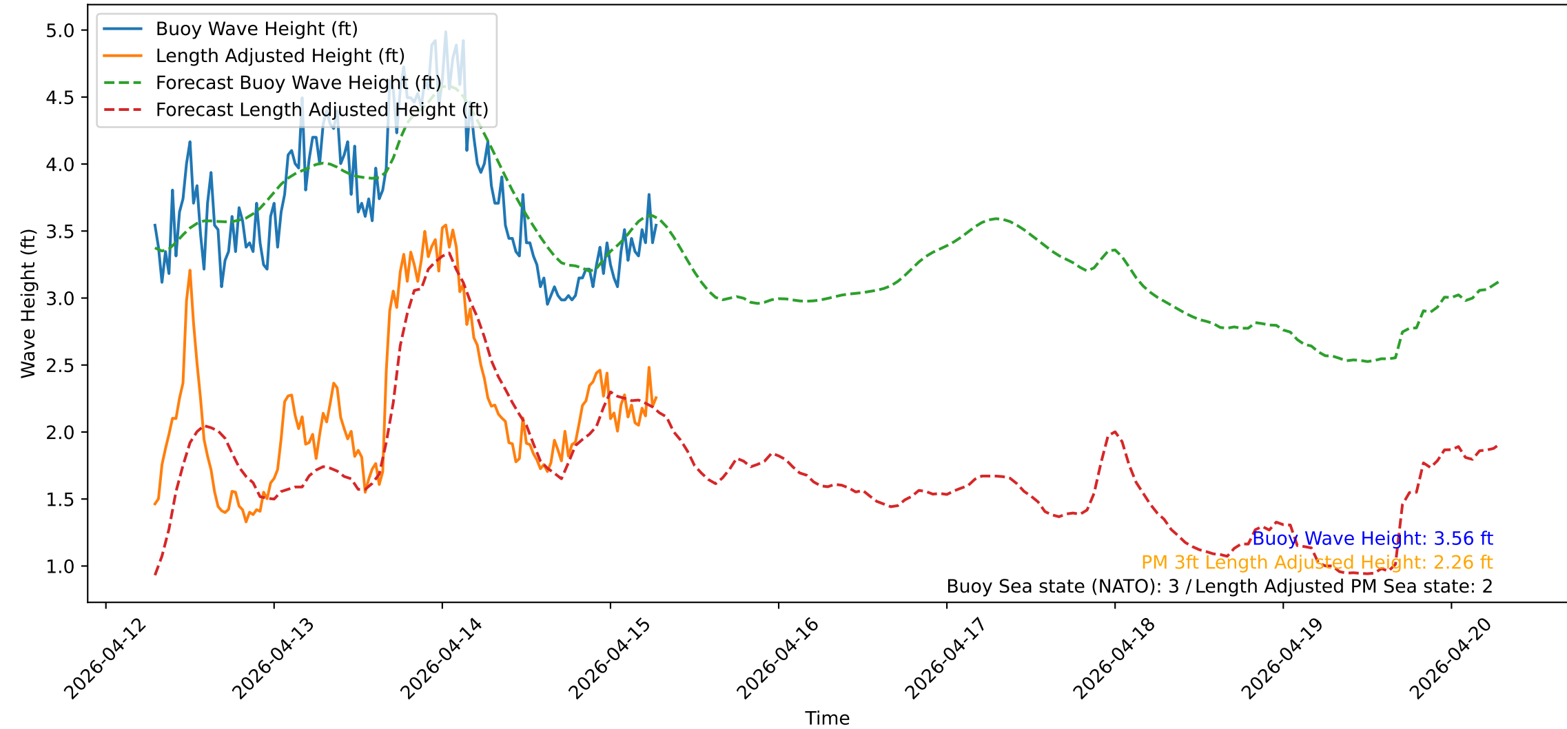
Wave Heights over Time for Green Beach at 2026-04-15 07:11:13
