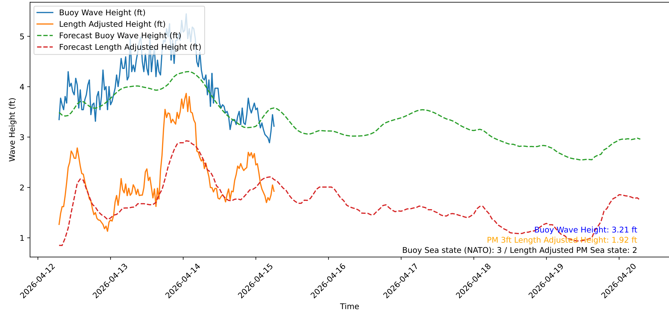
Wave Heights over Time for Oceanside Harbor at 2026-04-15 07:10:31
