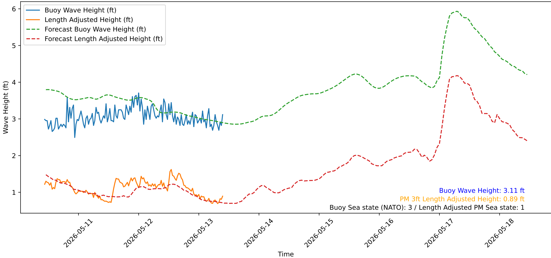
Wave Heights over Time for Oceanside Harbor at 2026-05-13 10:30:32
