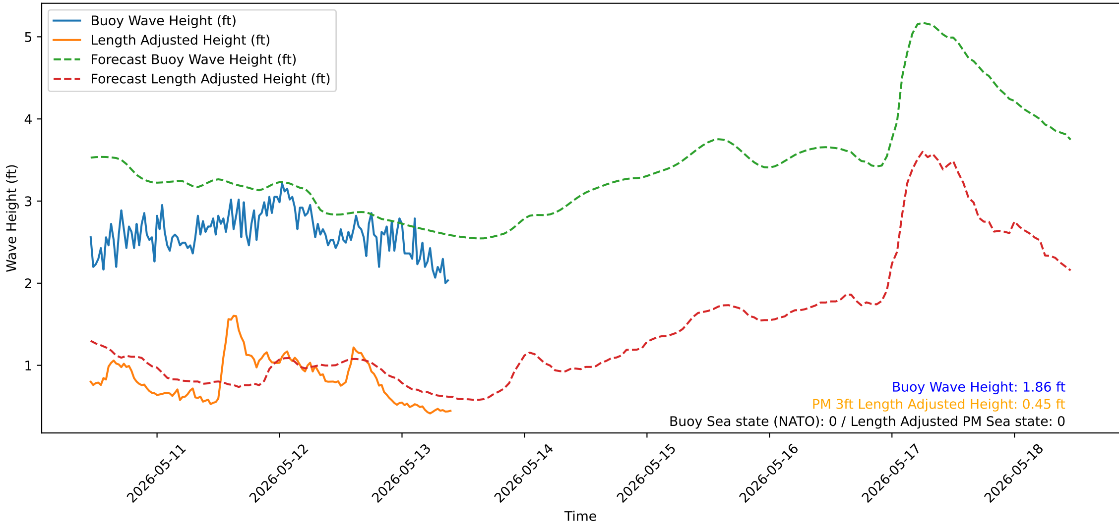
Wave Heights over Time for Red Beach at 2026-05-13 10:30:52
