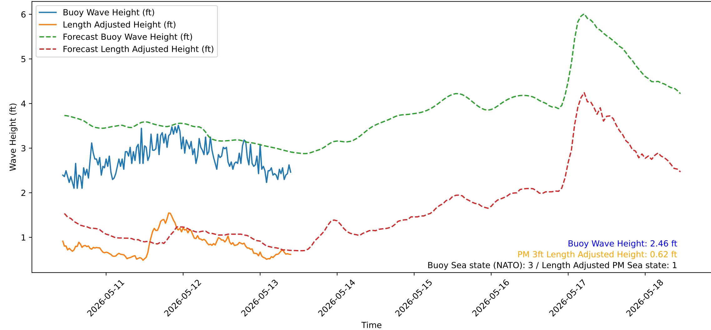
Wave Heights over Time for Green Beach at 2026-05-13 10:31:14
