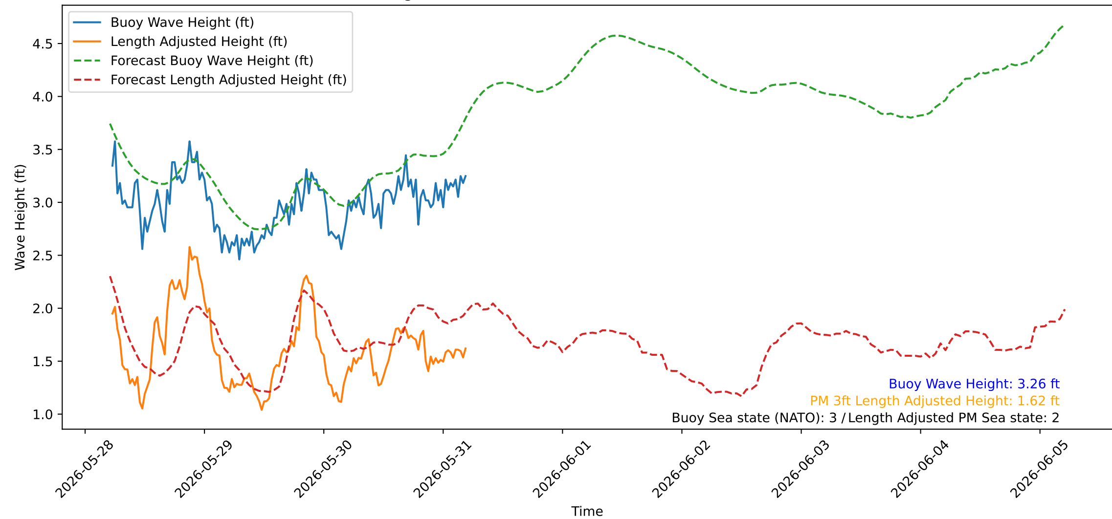
Wave Heights over Time for Green Beach at 2026-05-31 05:21:08
