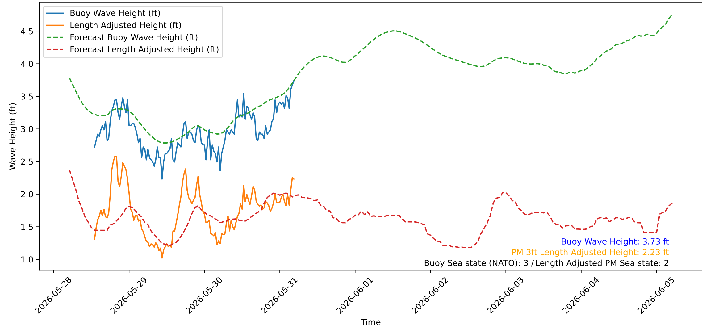
Wave Heights over Time for Oceanside Harbor at 2026-05-31 05:20:25
